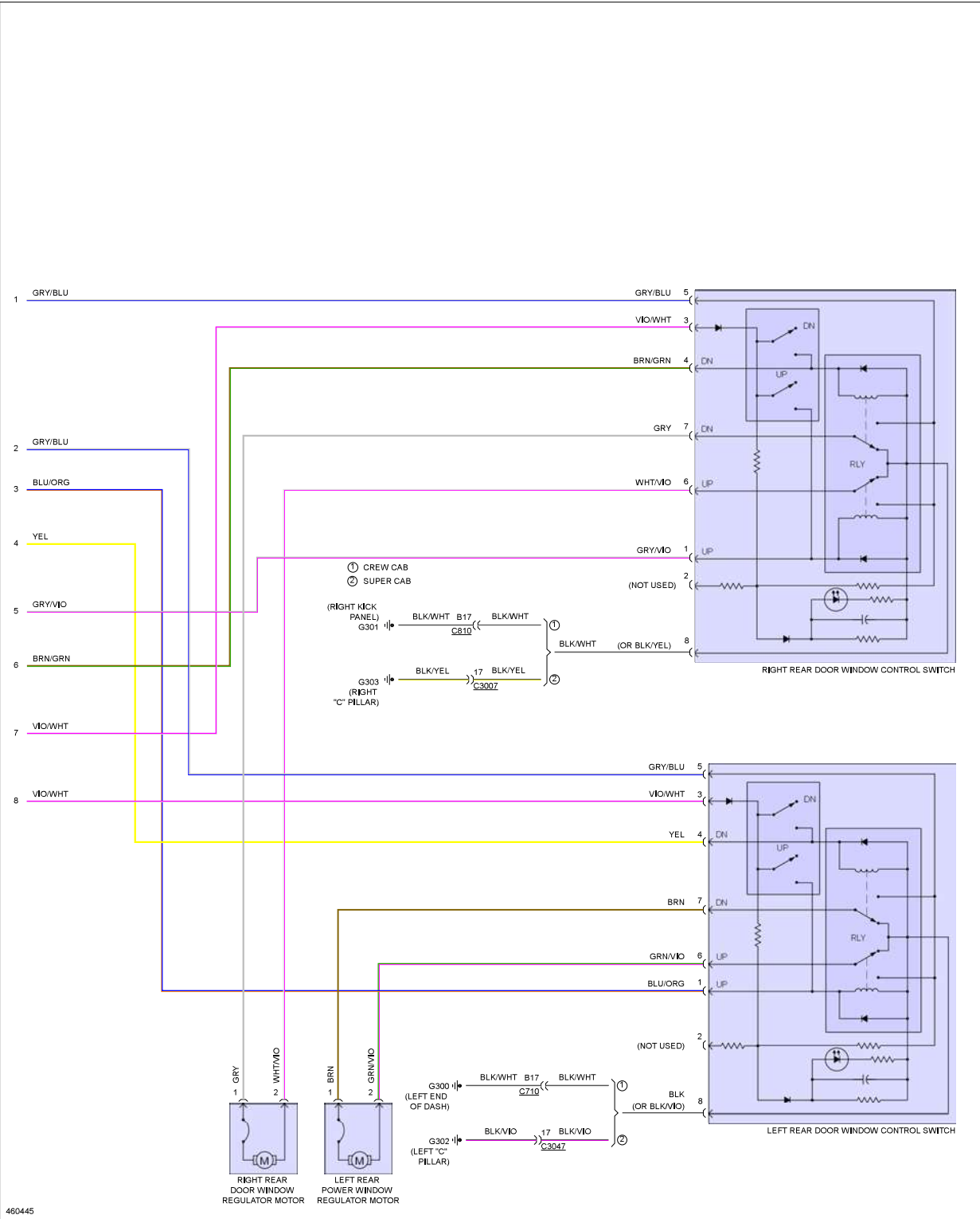
Fig 2: Power Windows Circuit, Crew Cab (2 of 2)
