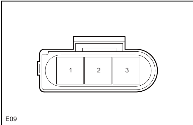
CKP Sensor Connector
