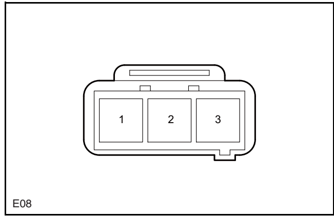
Instrument Cluster Connector A
