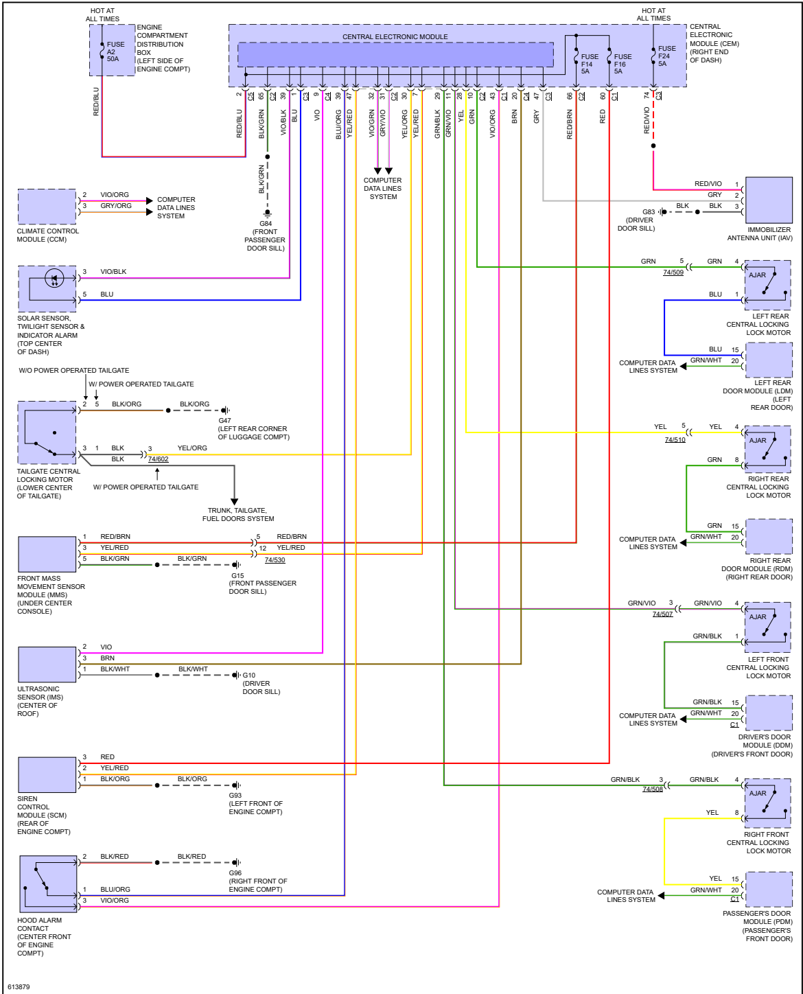
Fig 1: Anti-theft Circuit
