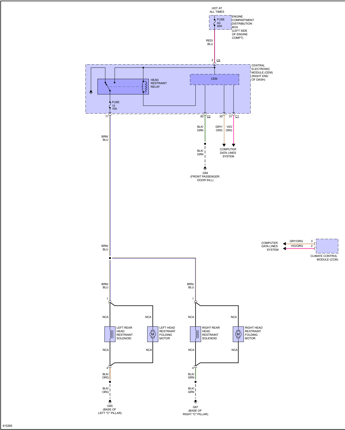
Fig 6: Rear Head Restraint Circuit
