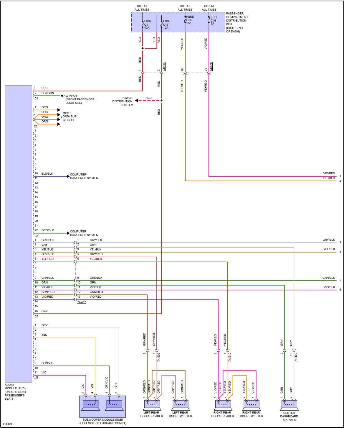
Fig 8: Radio Circuit, Premium IHU (1 of 3)
