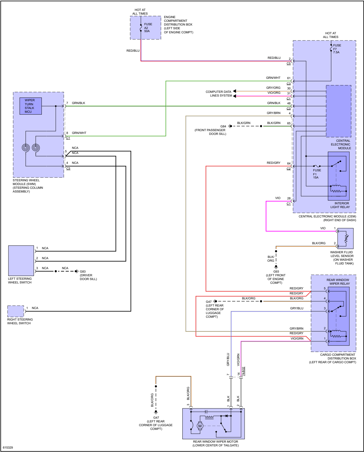
Fig 3: Rear Wiper/Washer Circuit
