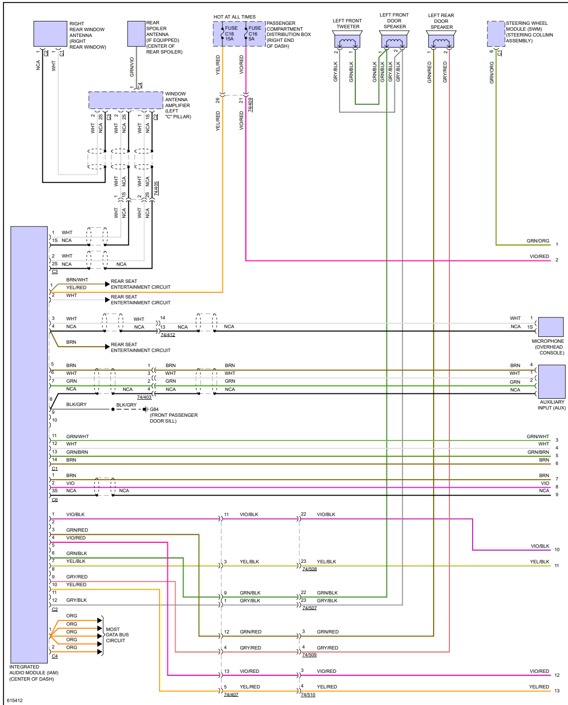
Fig 3: Radio Circuit, Base (1 of 2)
