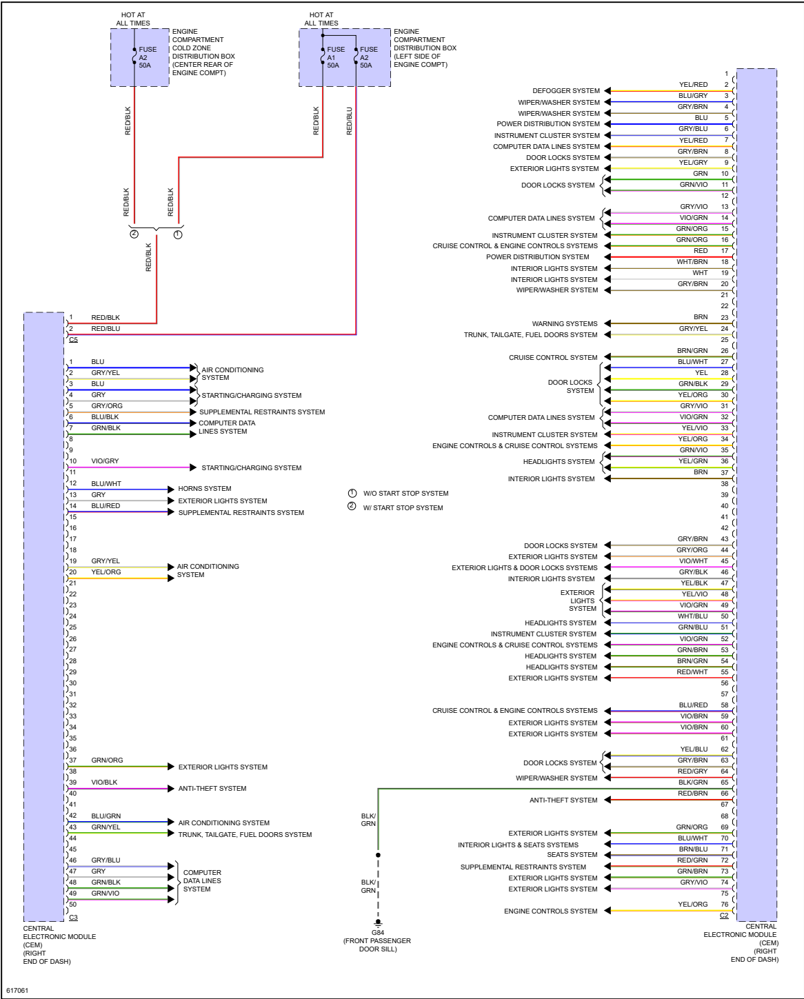
Fig 2: Body Control Modules Circuit (2 of 2)
