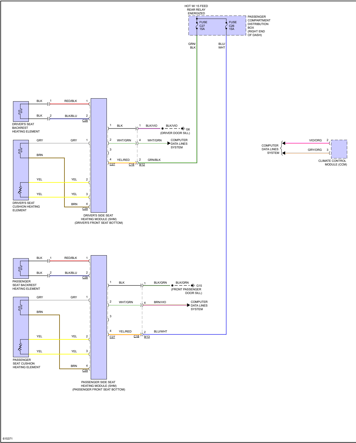
Fig 2: Front Heated Seats Circuit, W/O Fans
