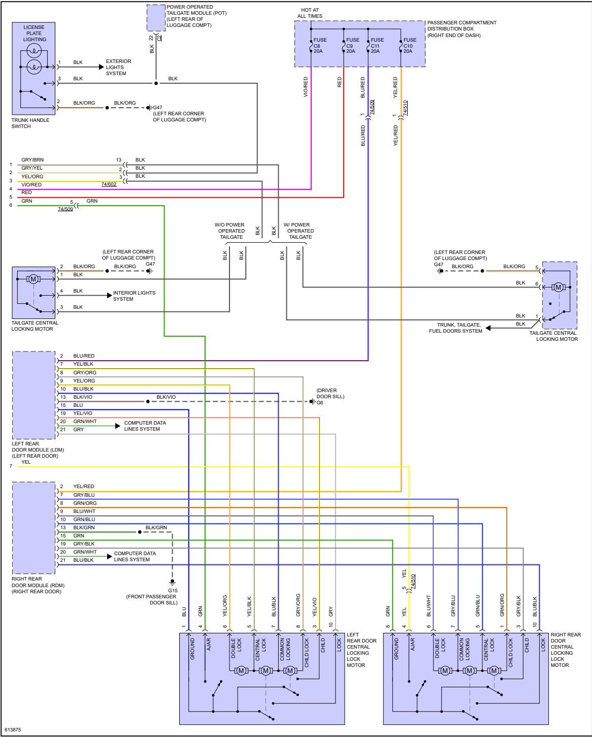
Fig 4: Power Door Locks Circuit, W/O Intelligent Key (2 of 2)
