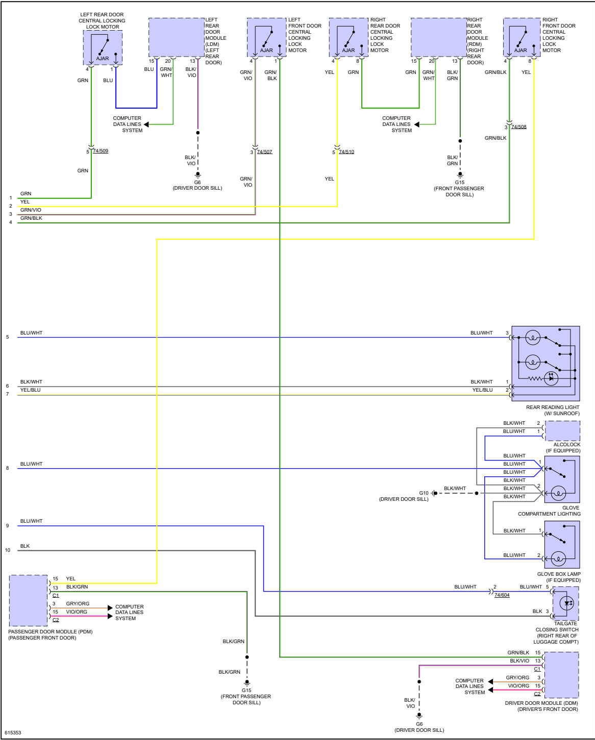
Fig 2: Courtesy Lamps Circuit (2 of 2)
