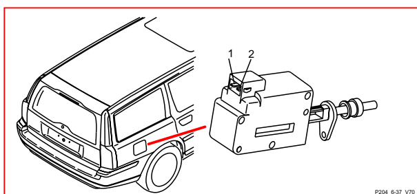
6/37 Lock motor, fuel filler flap V70
