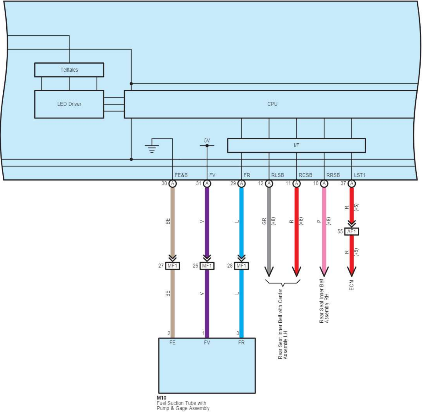
F6(A), F7(B) Combination Meter Assembly
