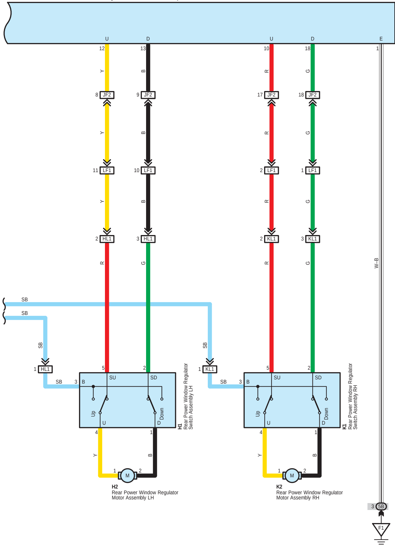
J1 Power Window Regulator Master Switch Assembly
