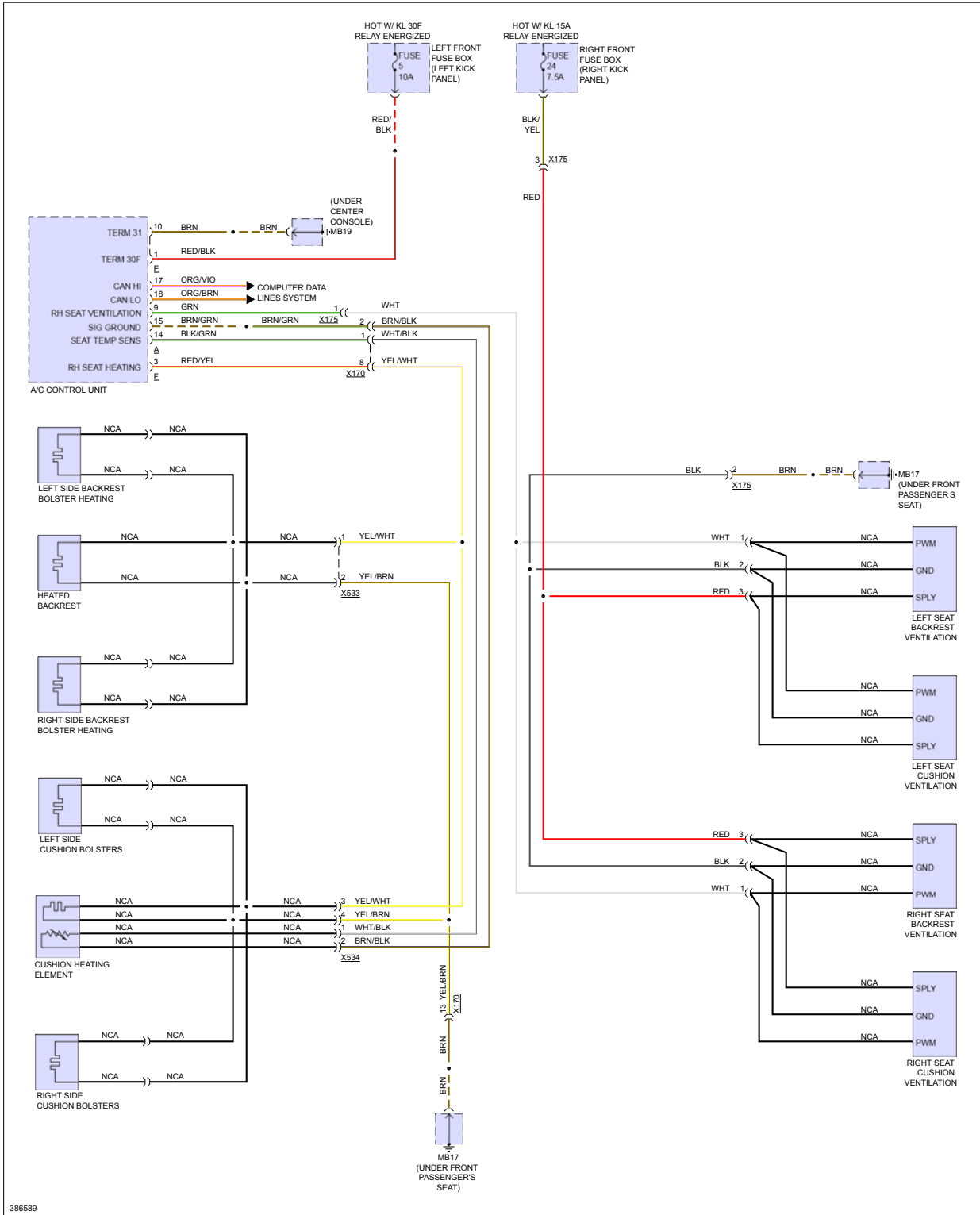
Fig 1: Front Heated Seats Circuit, W/ Passenger Power Seats
