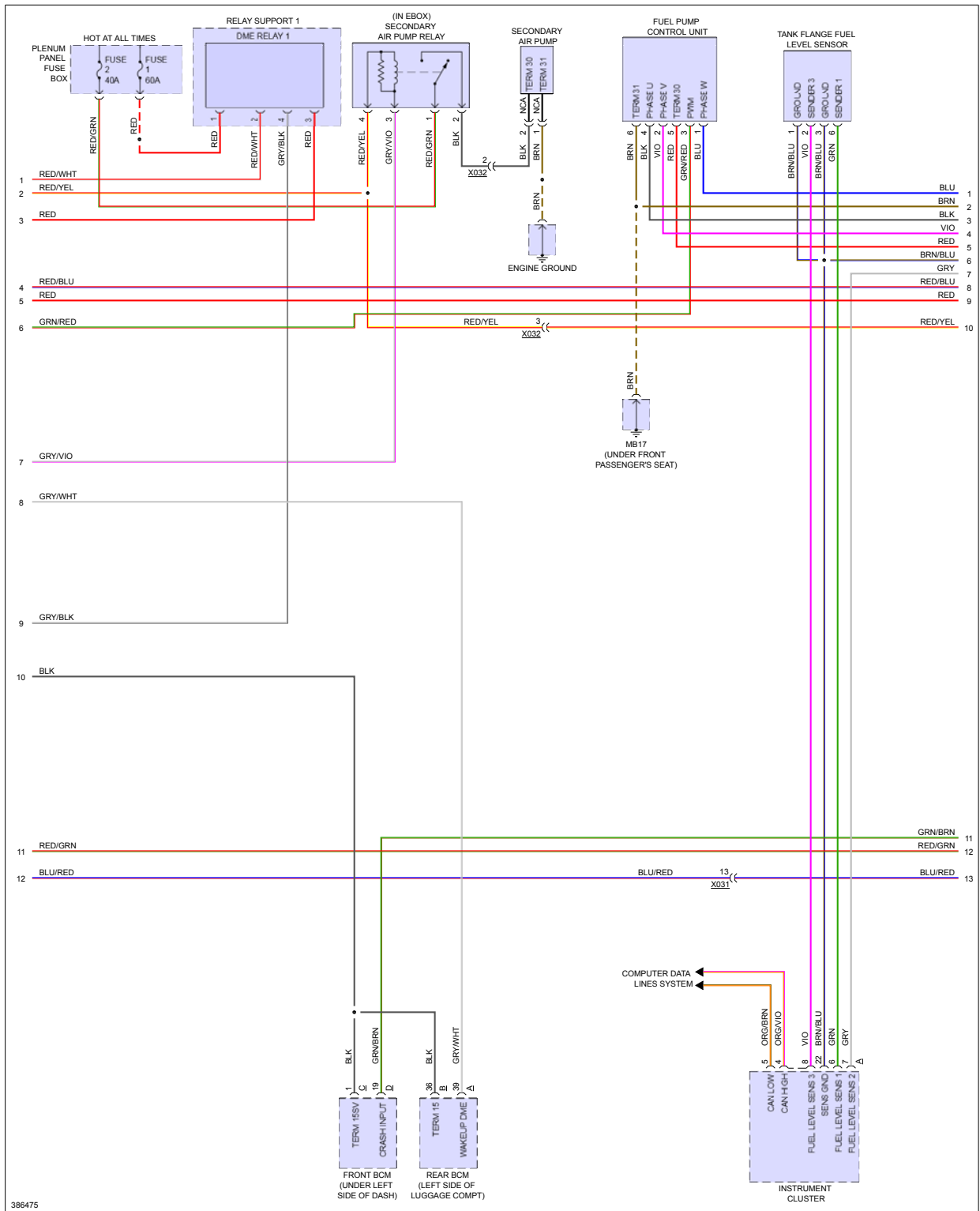
Fig 2: 4.8L Twin Turbo, Engine Performance Circuit (2 of 5)
