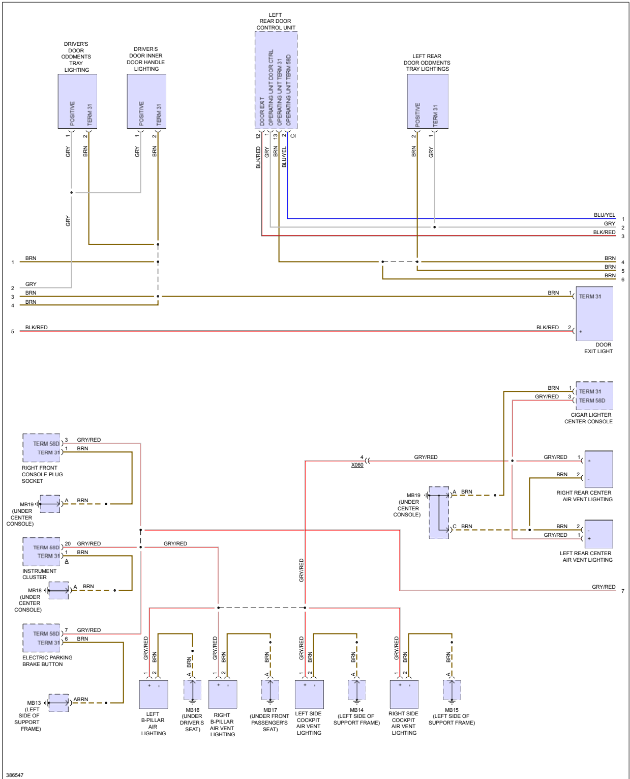
Fig 3: Interior Lights Circuit (3 of 5)
