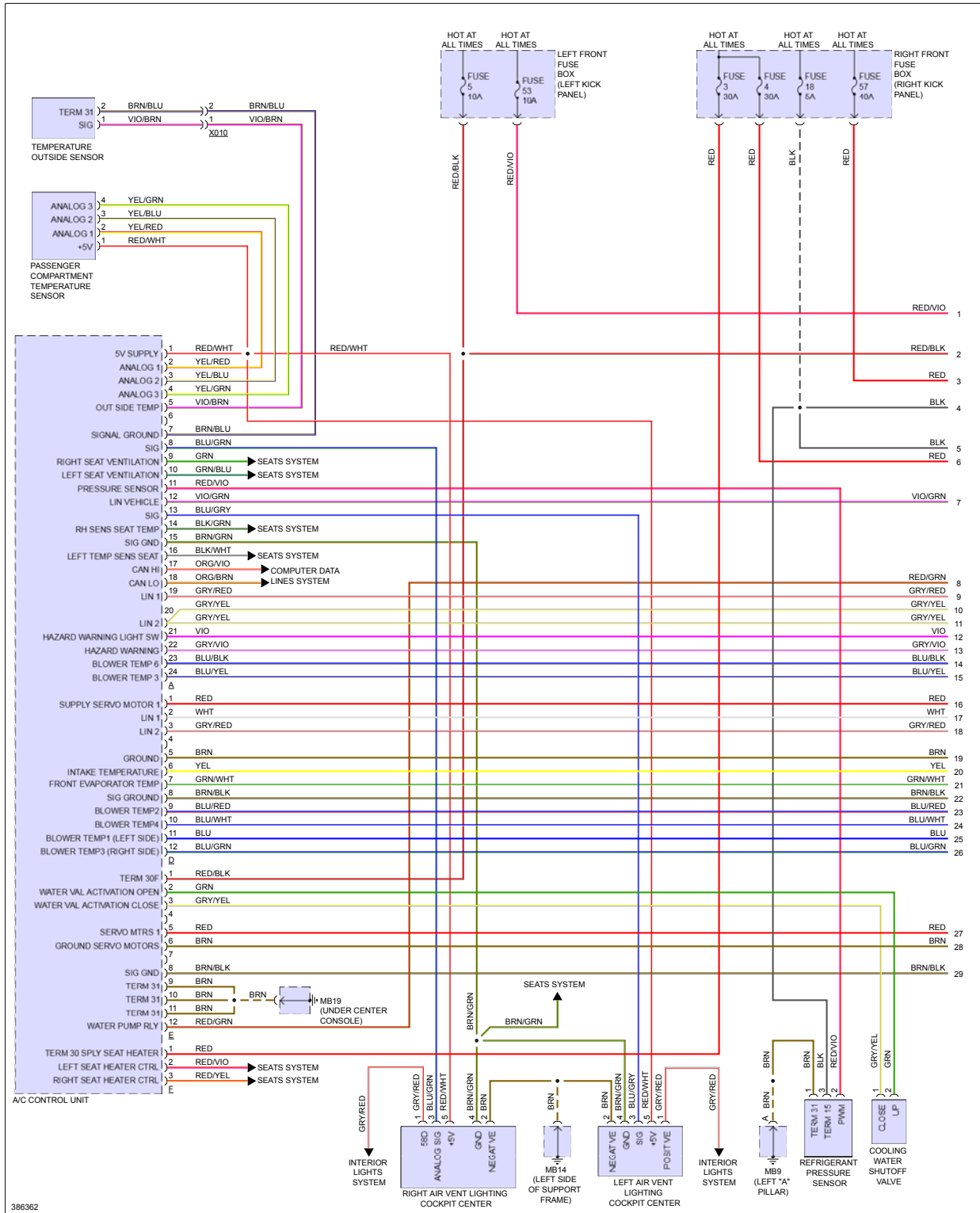
Fig 5: Automatic A/C Circuit, Hybrid (1 of 4)
