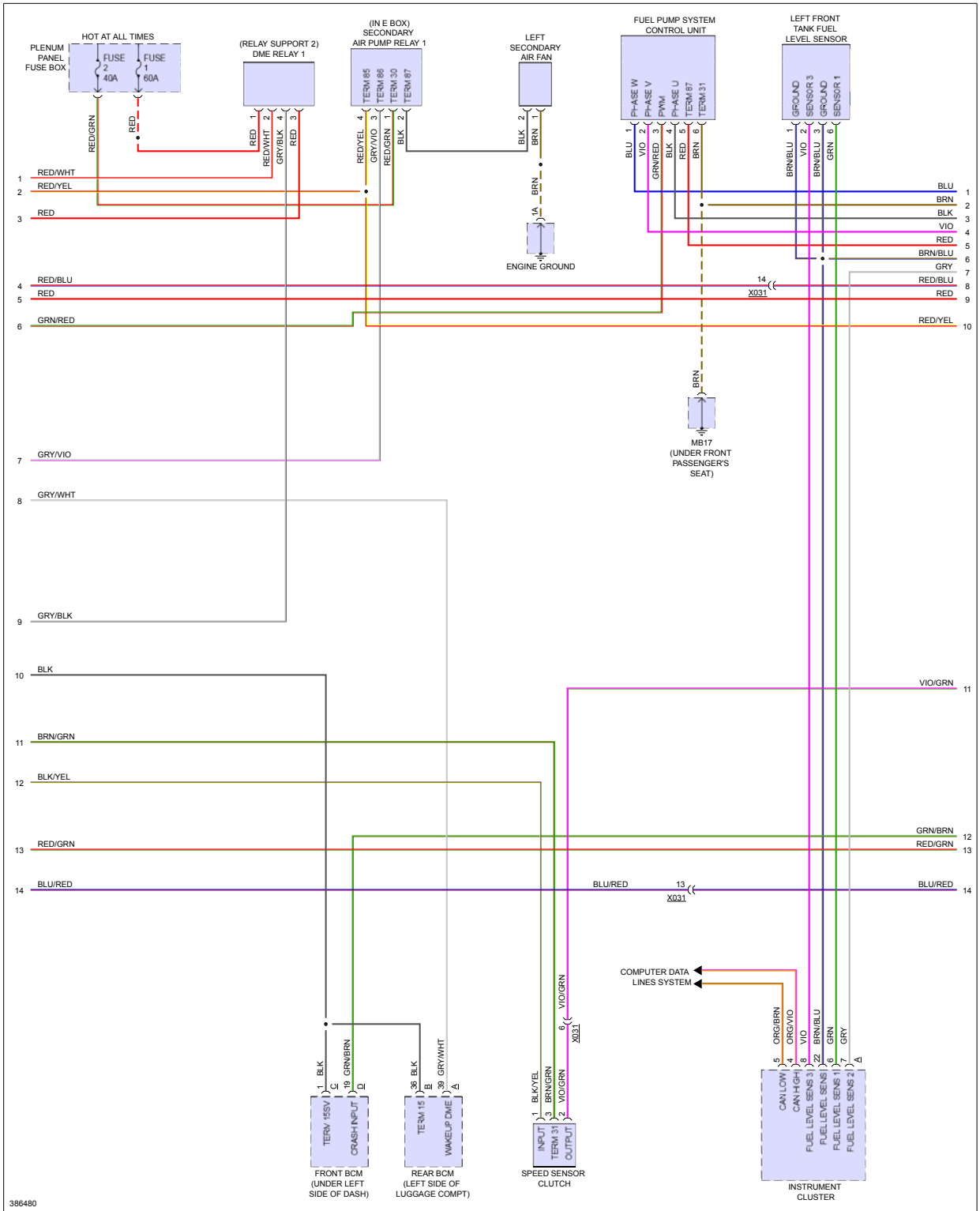
Fig 2: 3.6L, Engine Performance Circuit (2 of 5)
