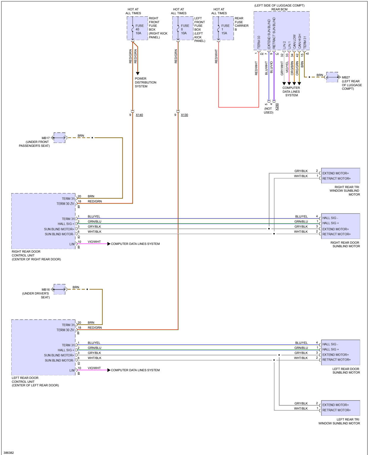
Fig 2: Rear Window Sun Shade Circuit
