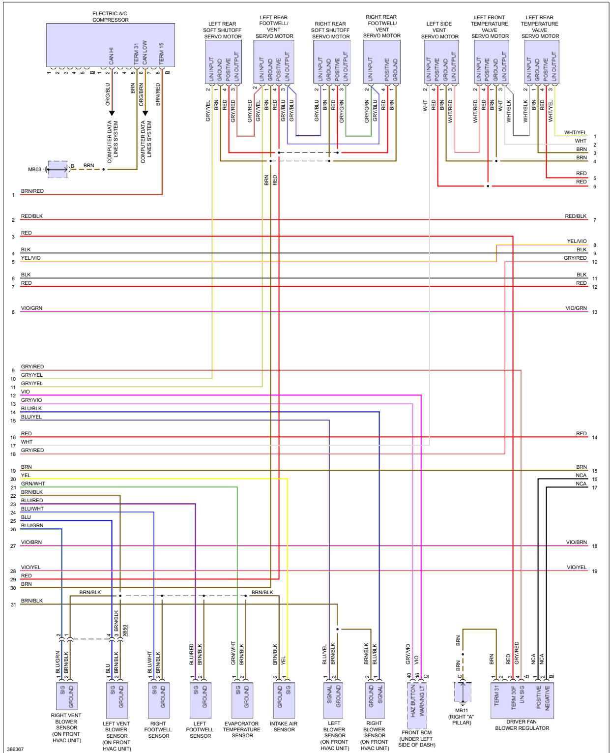
Fig 2: Automatic A/C Circuit, Except Hybrid (2 of 4)
