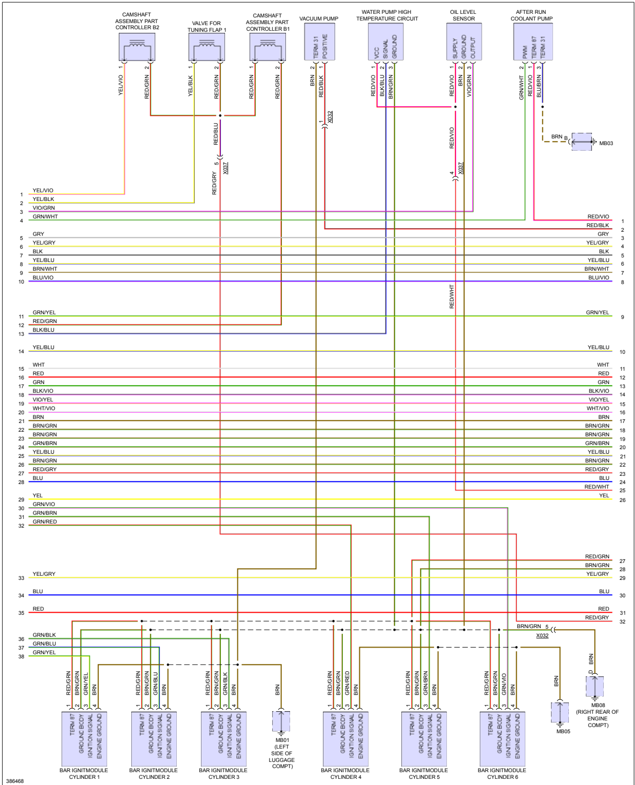
Fig 2: 3.0L Hybrid, Engine Performance Circuit (2 of 7)
