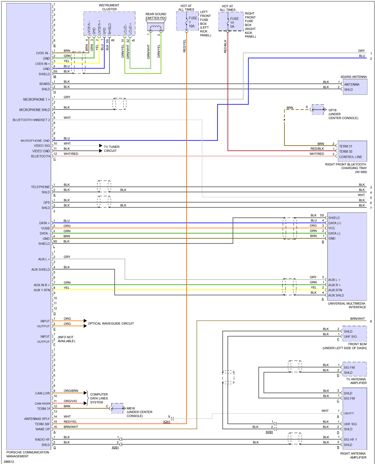
Fig 4: Navigation Circuit, W/ Bose (1 of 2)
