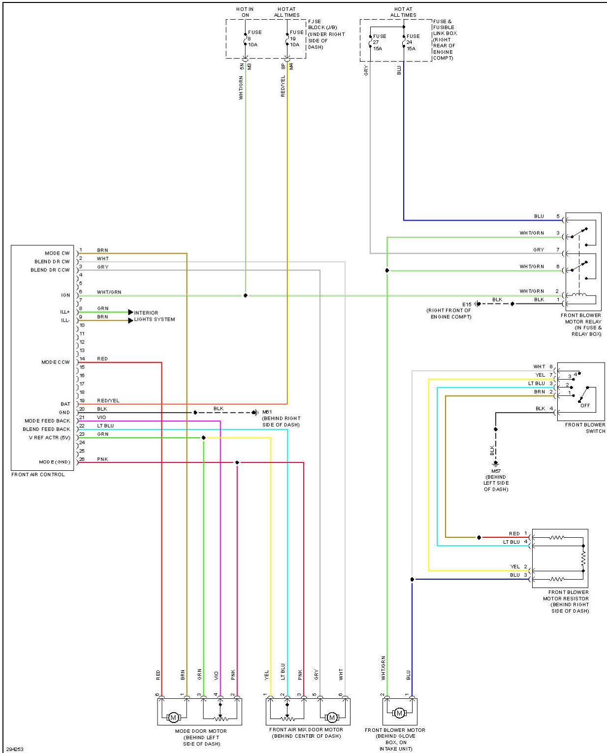
Fig. 1: Heater Circuit
