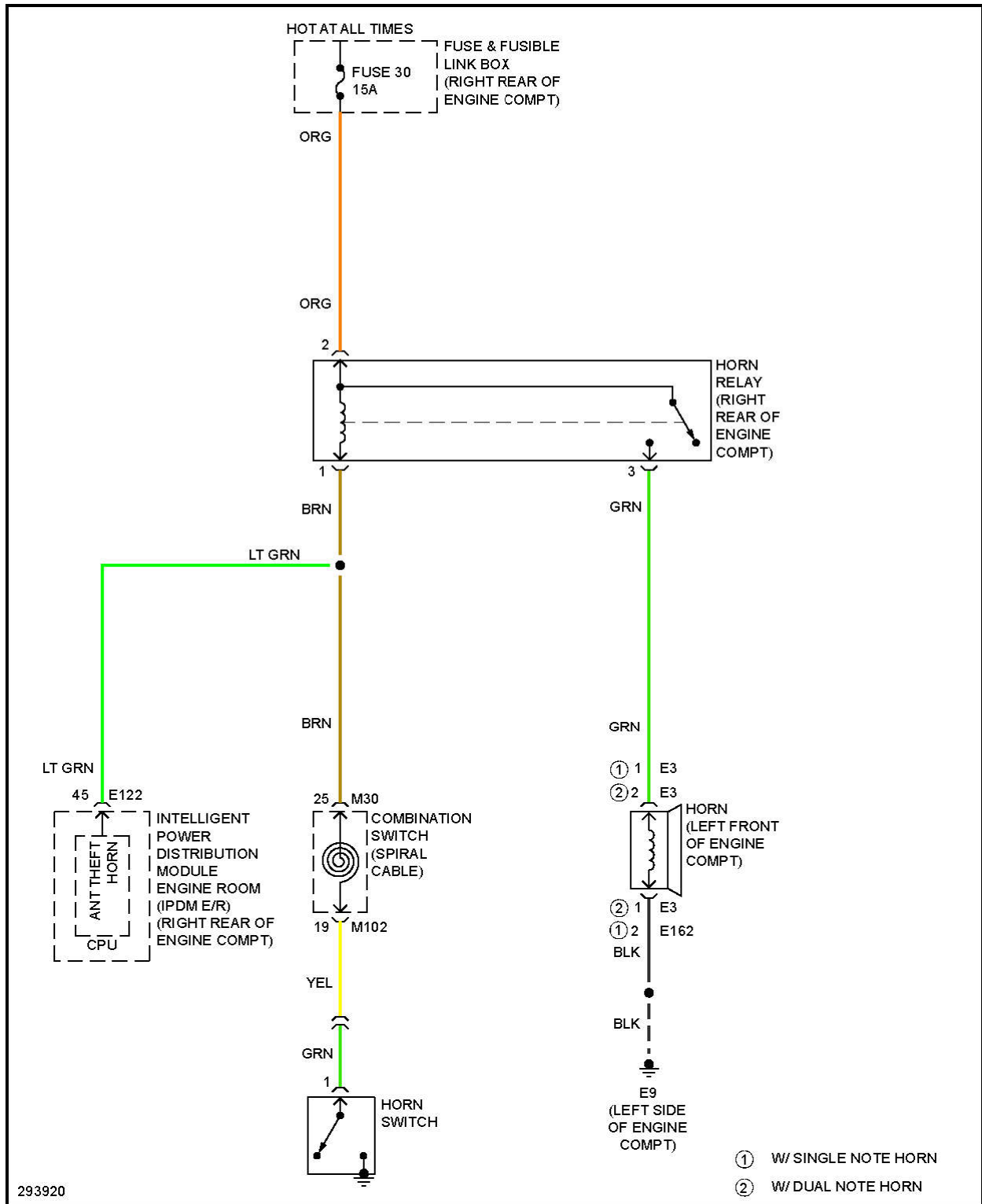
Fig. 32: Horn Circuit
