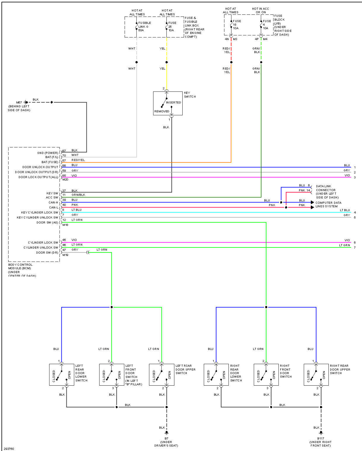
Fig. 46: Door Lock Circuit, King Cab (1 of 2)
