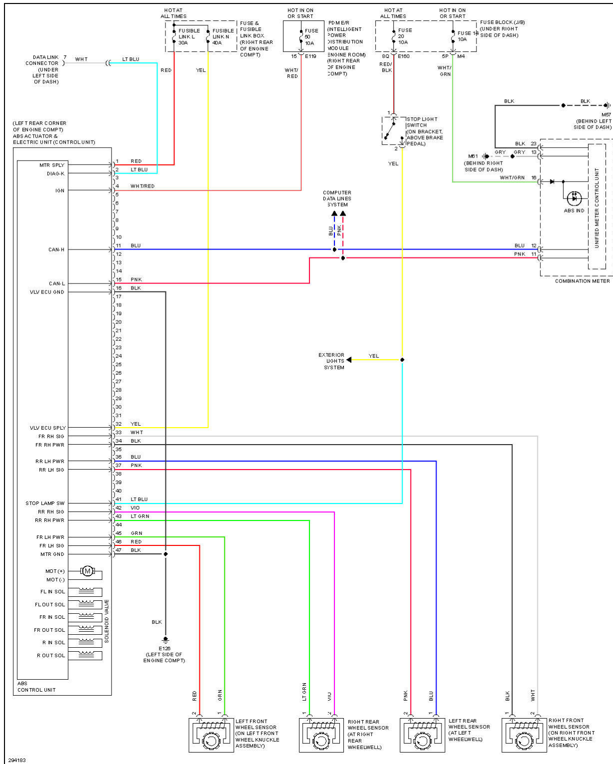
Fig. 6: Anti-lock Brakes Circuit, W/O Traction Control
