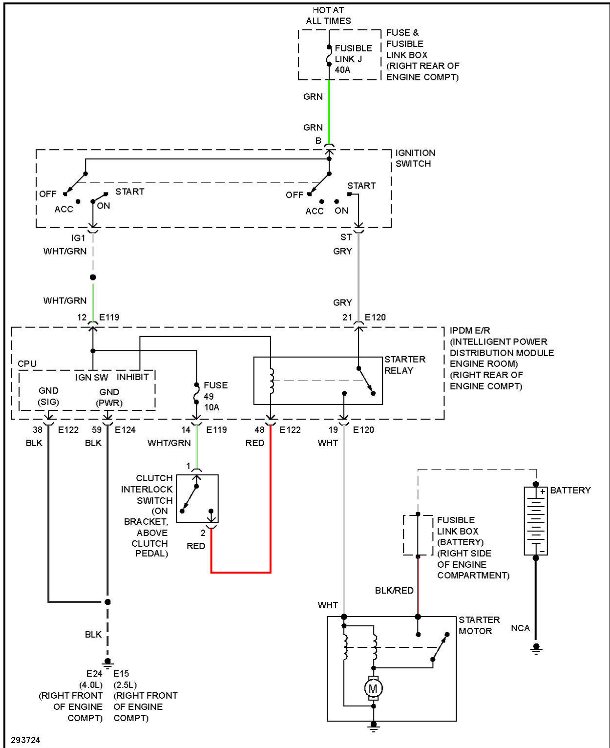
Fig. 63: Starting Circuit, M/T W/O Clutch Interlock
