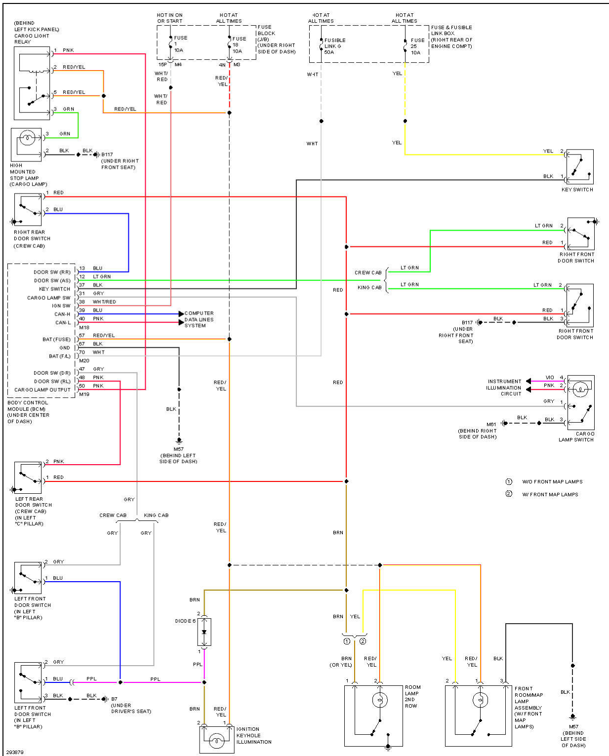
Fig. 36: Courtesy Lamps Circuit, W/O Power Door Locks
