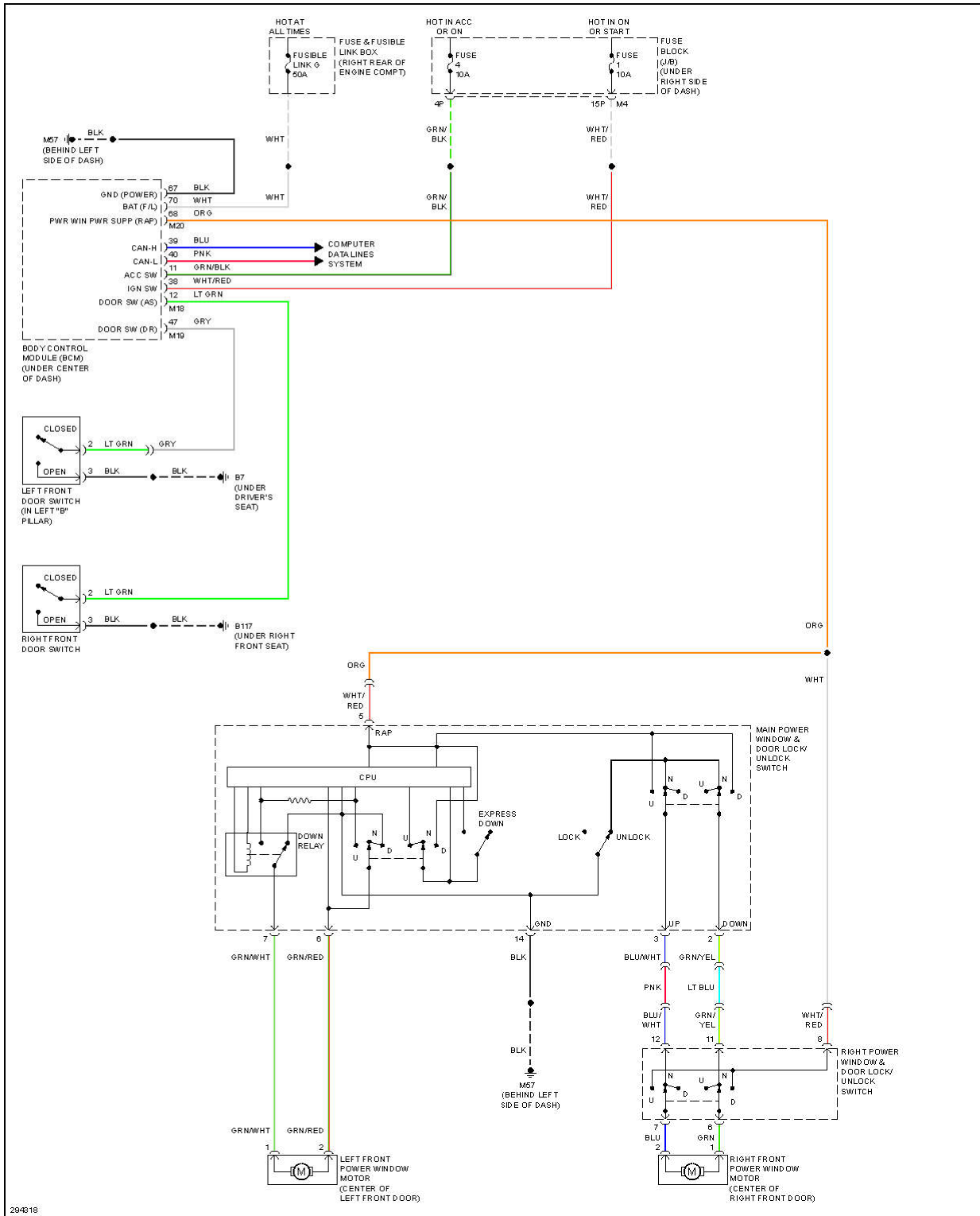
Fig. 54: Power Windows Circuit, King Cab
