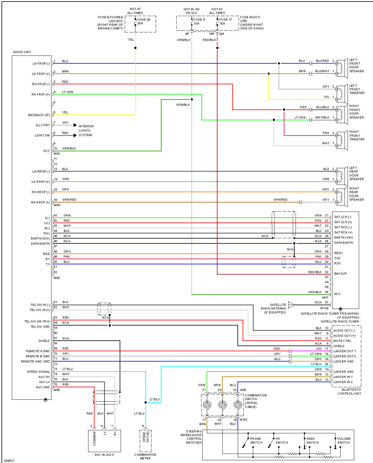
Fig. 58: Premium Sound Radio Circuit, King Cab
