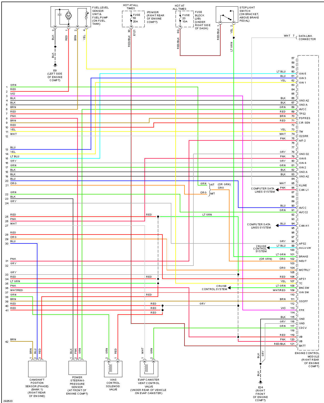
Fig. 22: 4.0L, Engine Performance Circuit (4 of 4)
