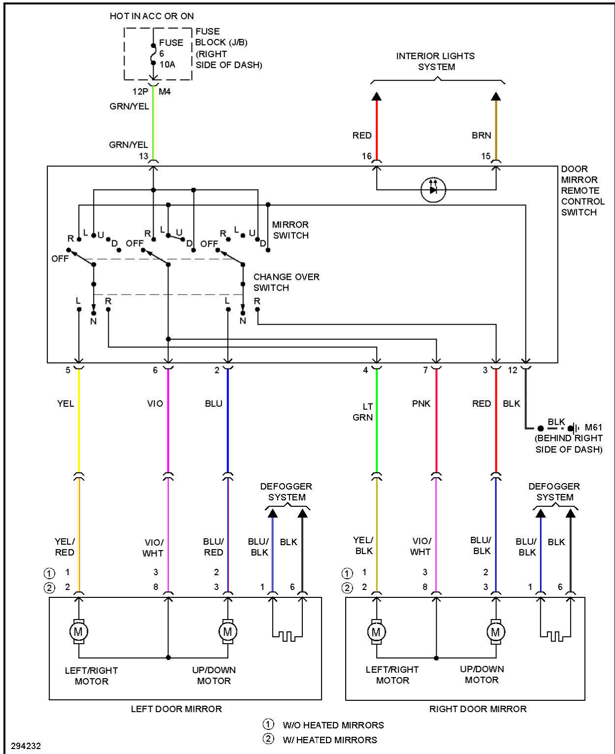
Fig. 49: Power Mirror Circuit
