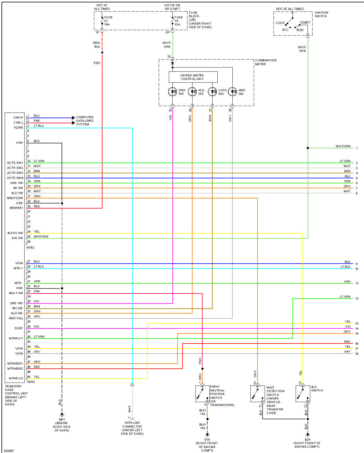
Fig. 68: 4WD Circuit, M/T (1 of 2)
