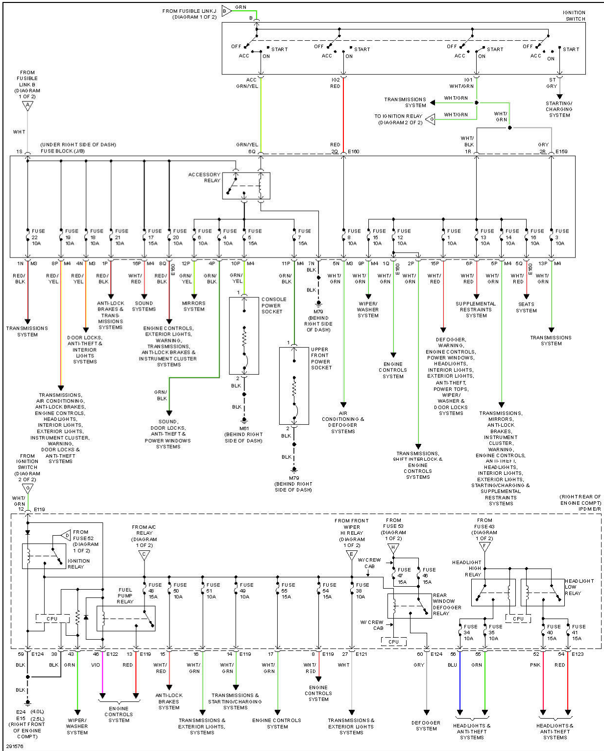
Fig. 39: Power Distribution Circuit (2 of 2)
