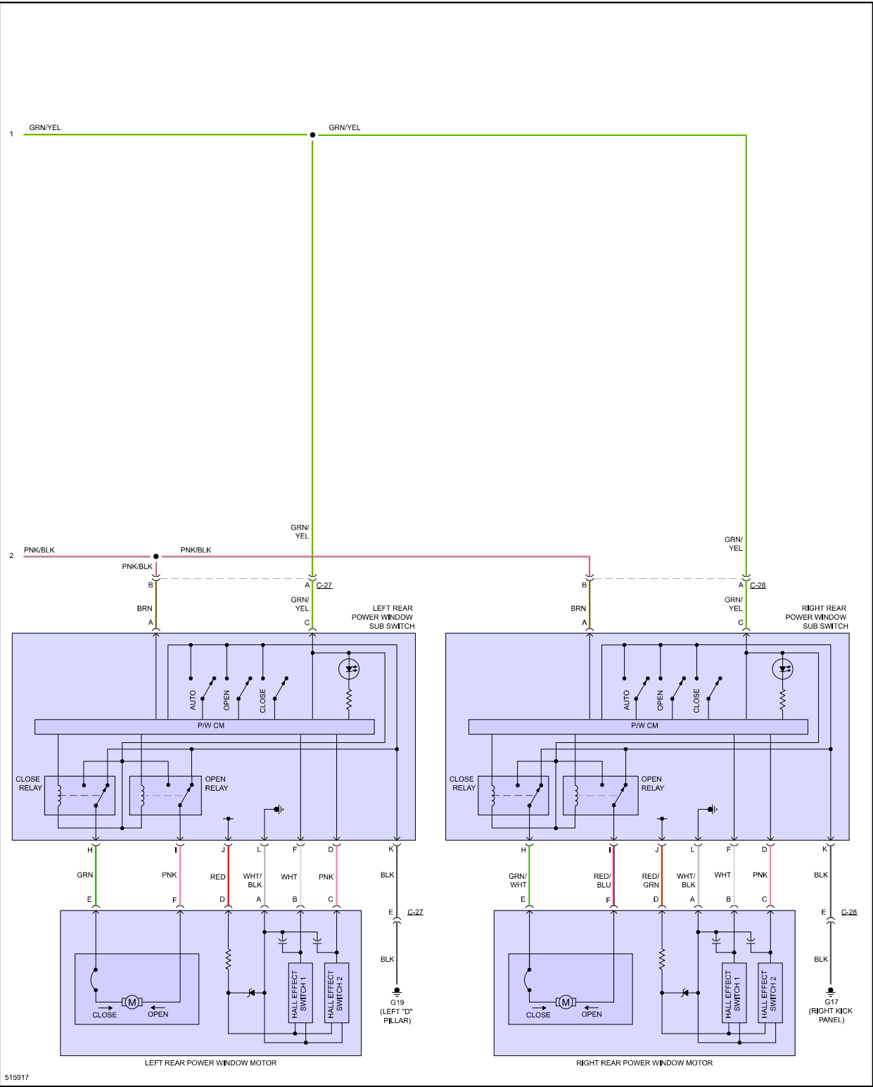
Fig 2: Power Windows Circuit, W/ All Windows Auto Open/Close (2 of 2)
