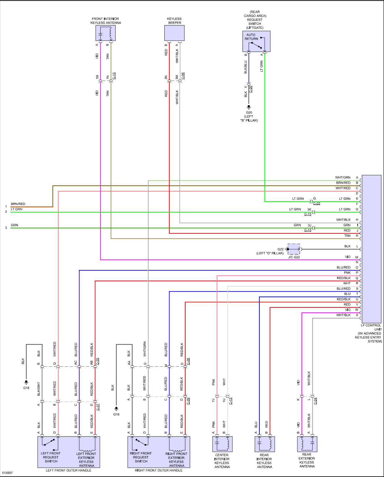
Fig 5: Anti-theft Circuit (5 of 5)
