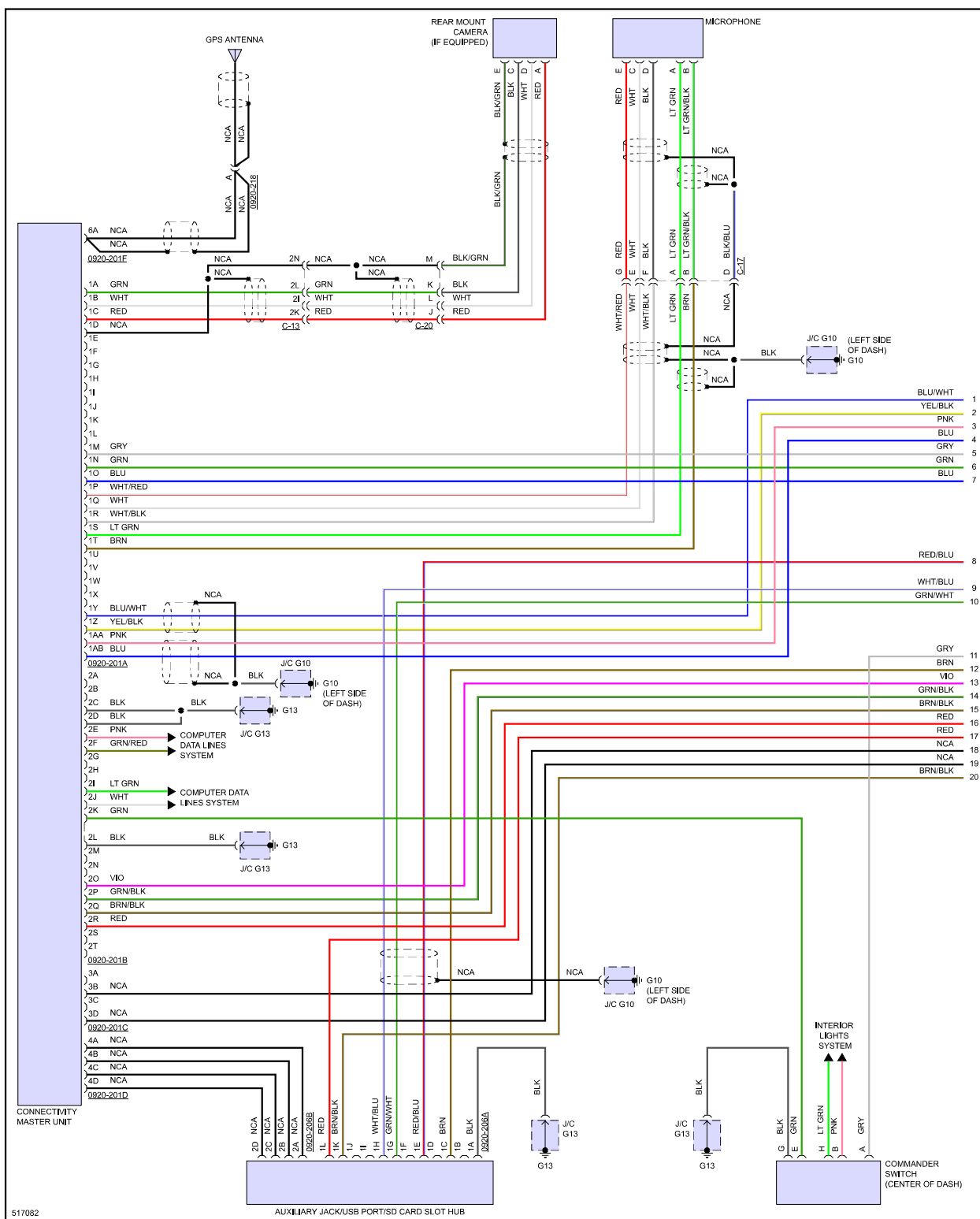
Fig 7: Radio Circuit, W/O Bose (1 of 3)
