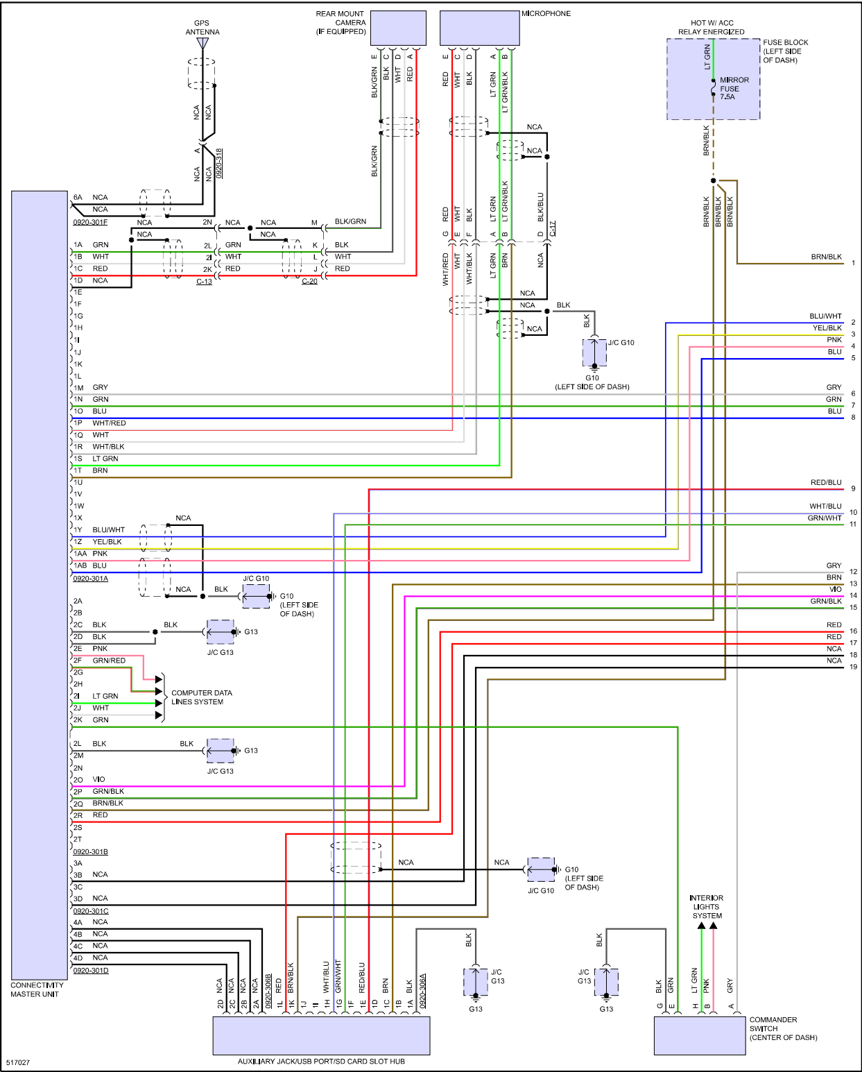
Fig 3: Navigation Circuit, W/ Bose (1 of 6)
