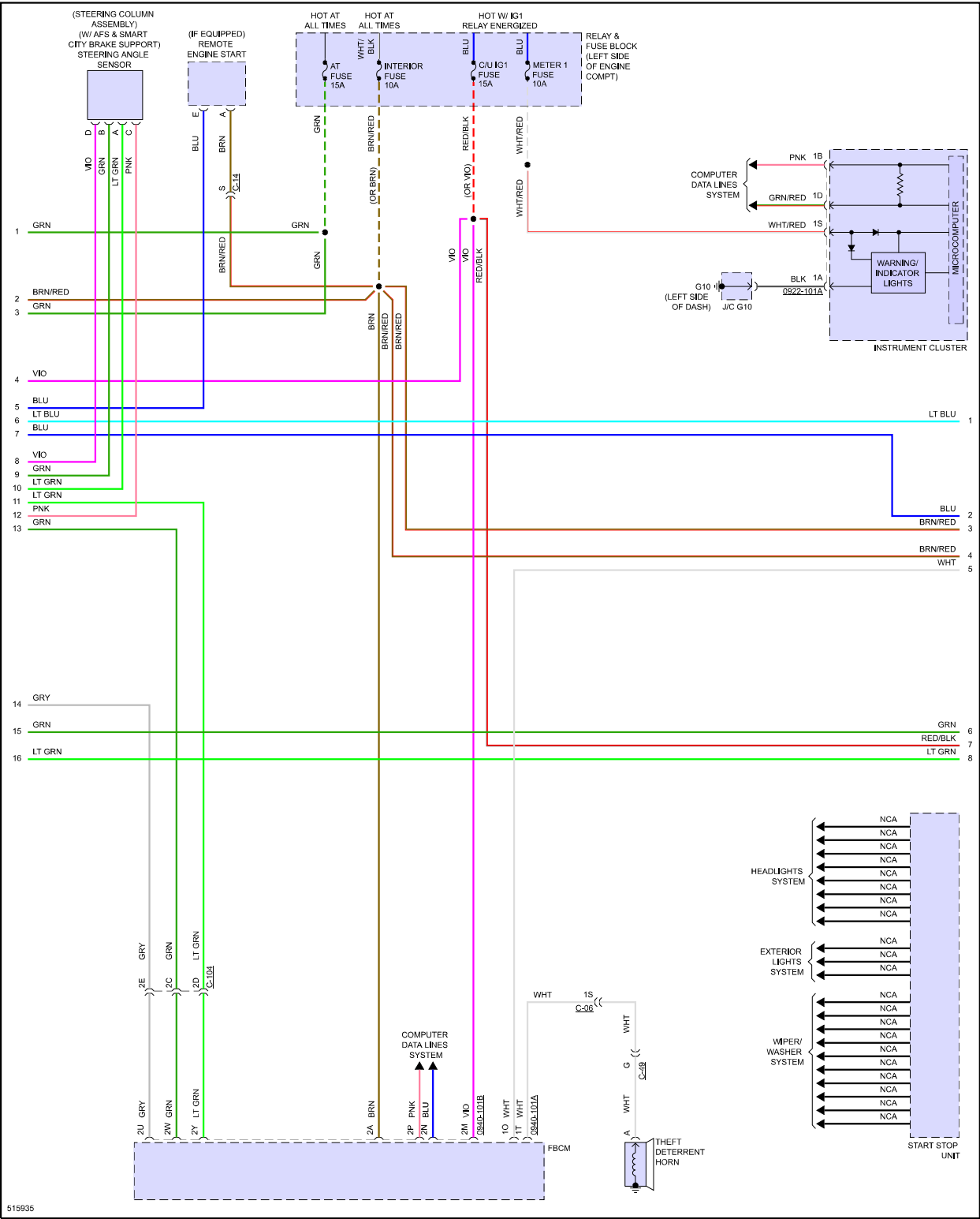
Fig 2: Power Door Locks Circuit (2 of 5)
