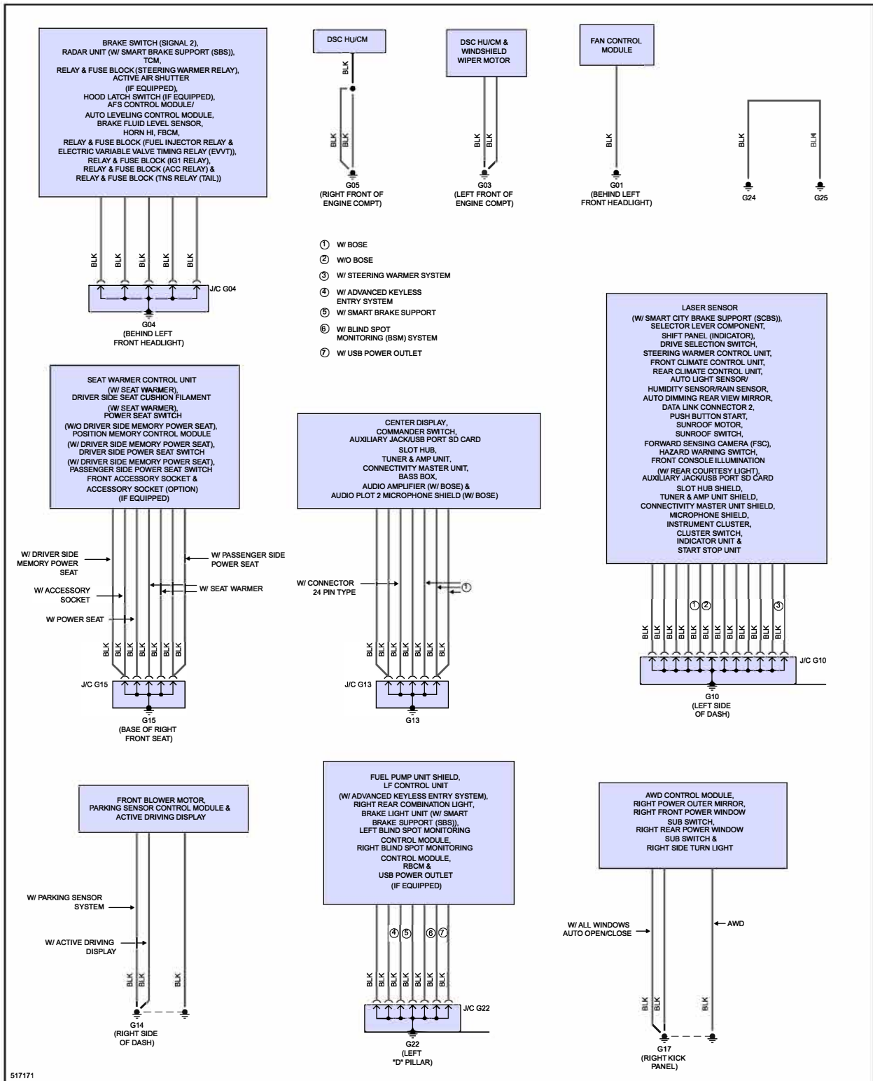
Fig 1: Ground Distribution Circuit (1 of 2)
