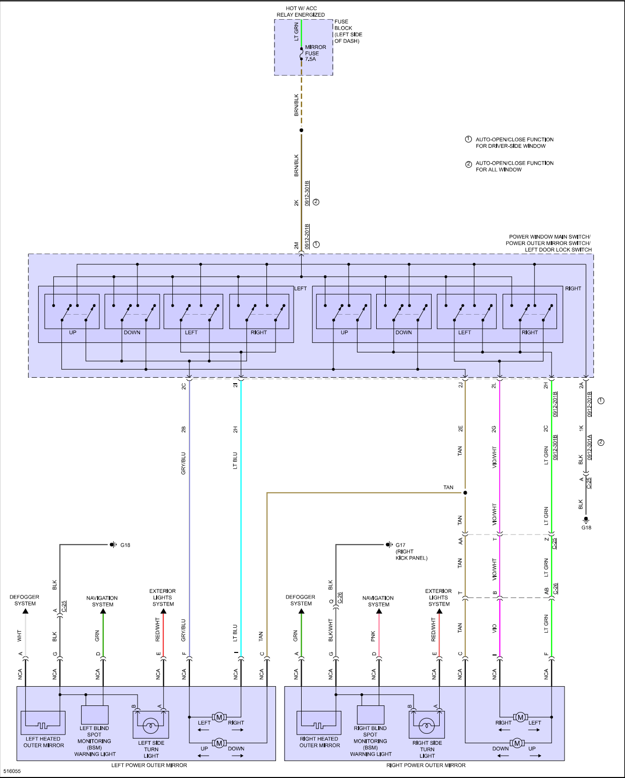
Fig 2: Power Mirror Circuit
