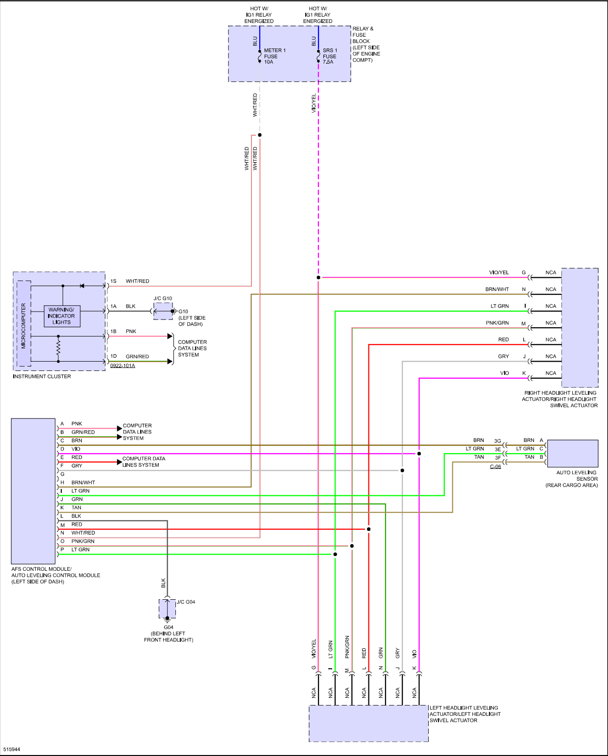
Fig 4: Headlamps Leveling Circuit
