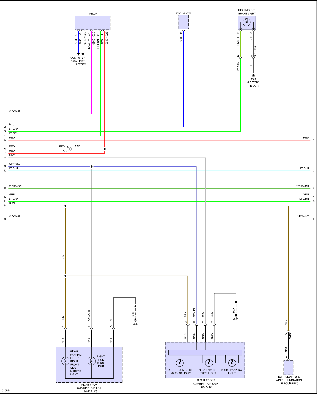
Fig 5: Exterior Lamps Circuit, W/ Smart Brake Support (4 of 5)
