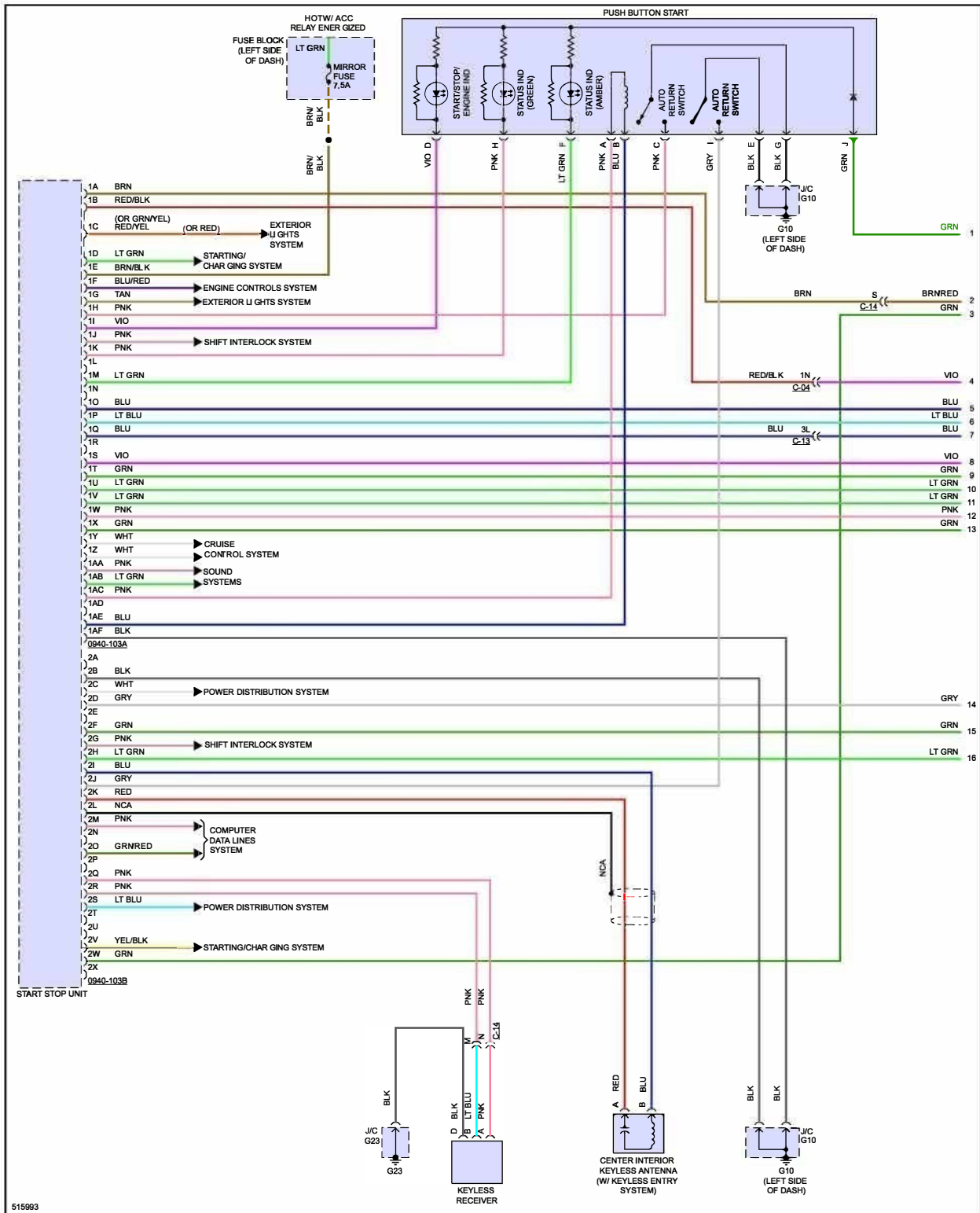
Fig 1: Anti-theft Circuit (1 of 5)
