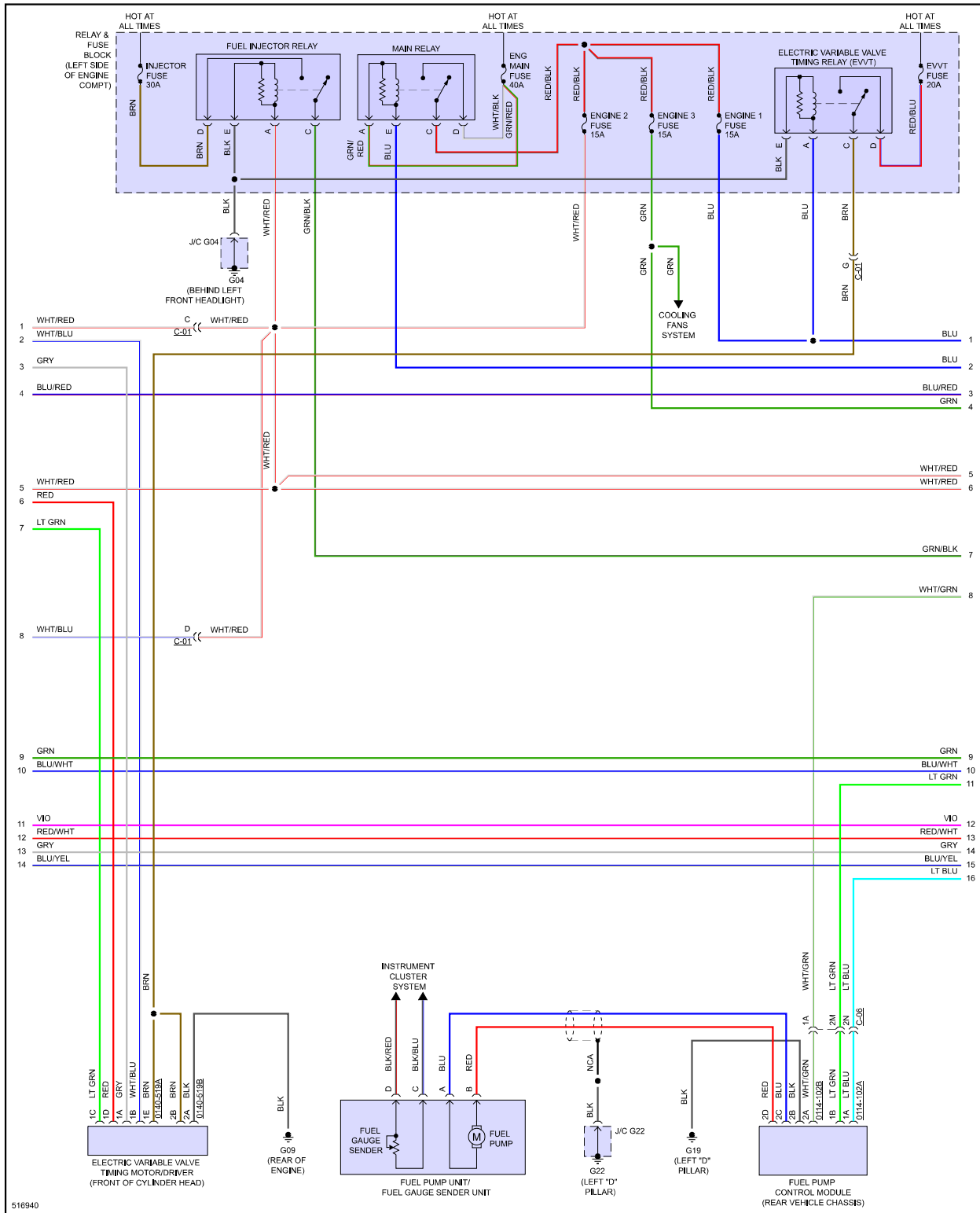
Fig 4: 2.5L, Engine Performance Circuit (4 of 7)
