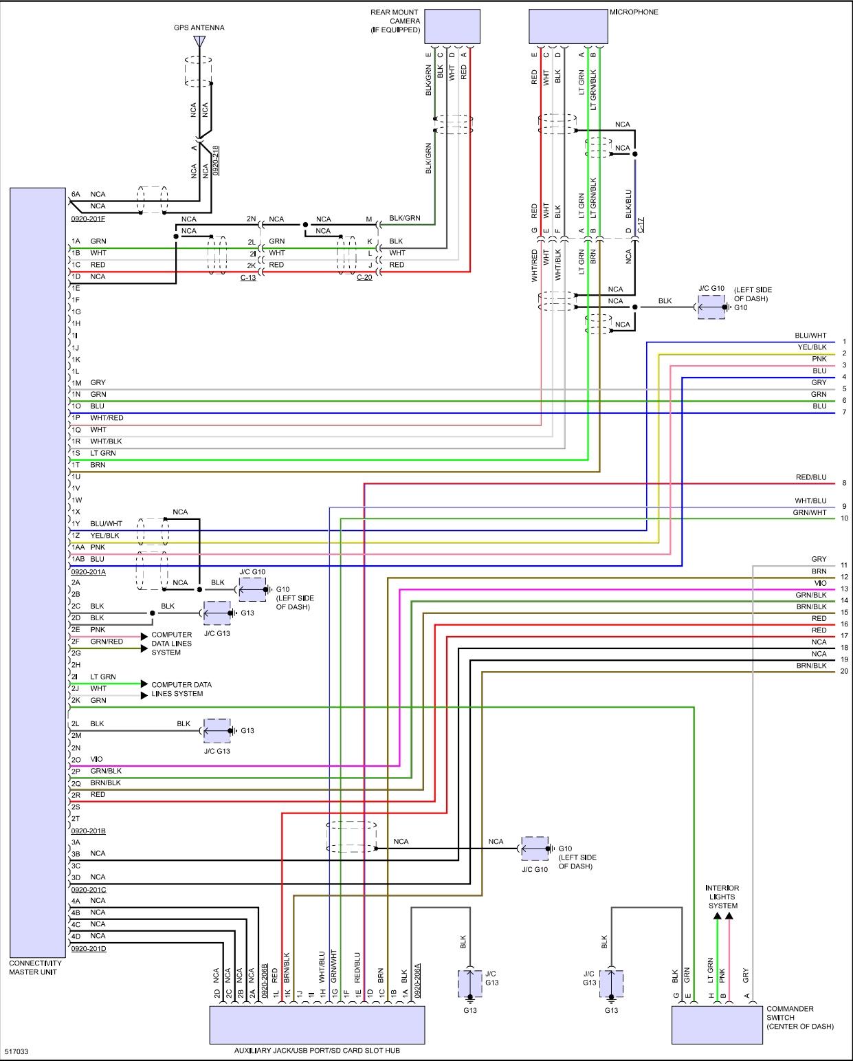
Fig 9: Navigation Circuit, W/O Bose (1 of 3)
