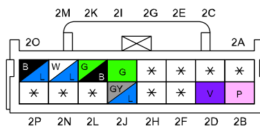
0920-302B AUDIO AMPLIFIER
