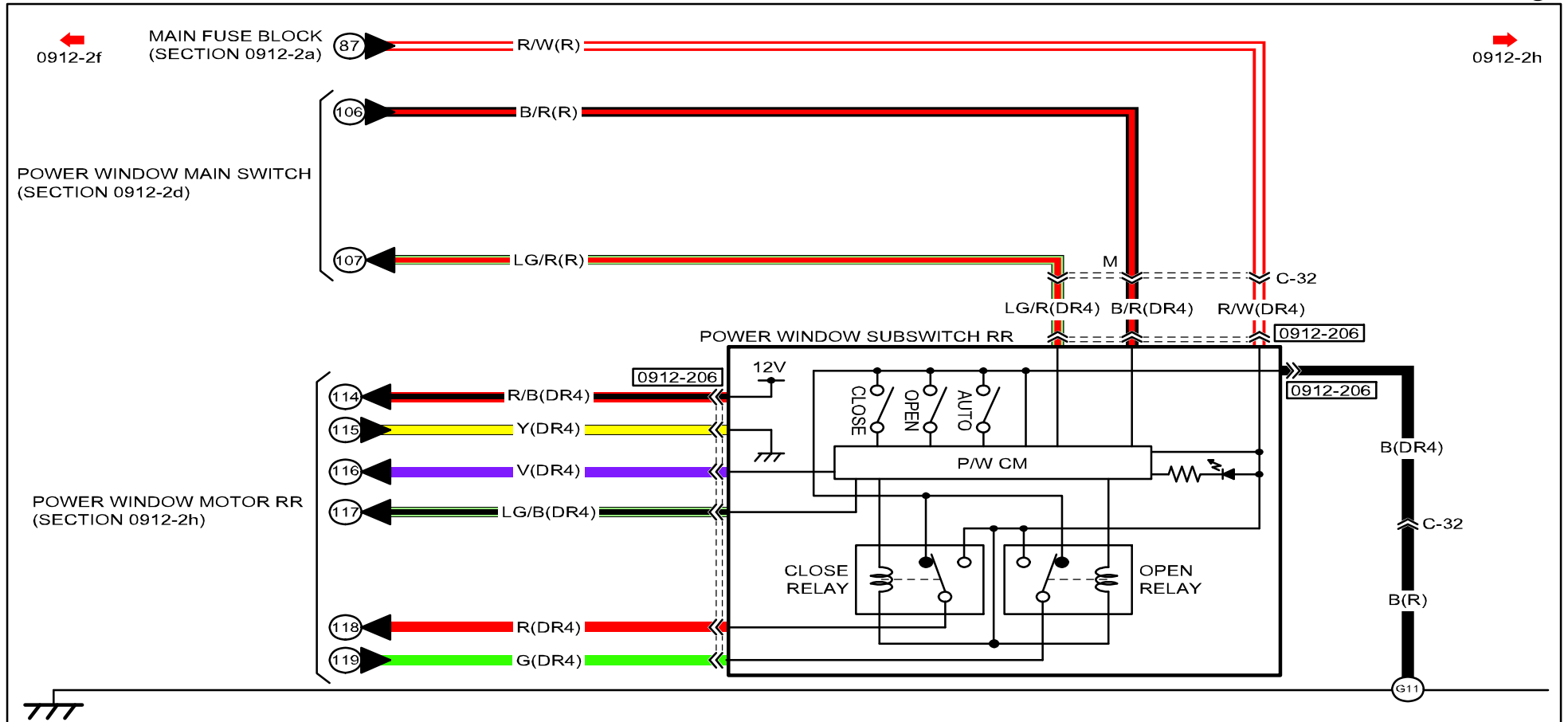
0912-206 POWER WINDOW SUBSWITCH RR
