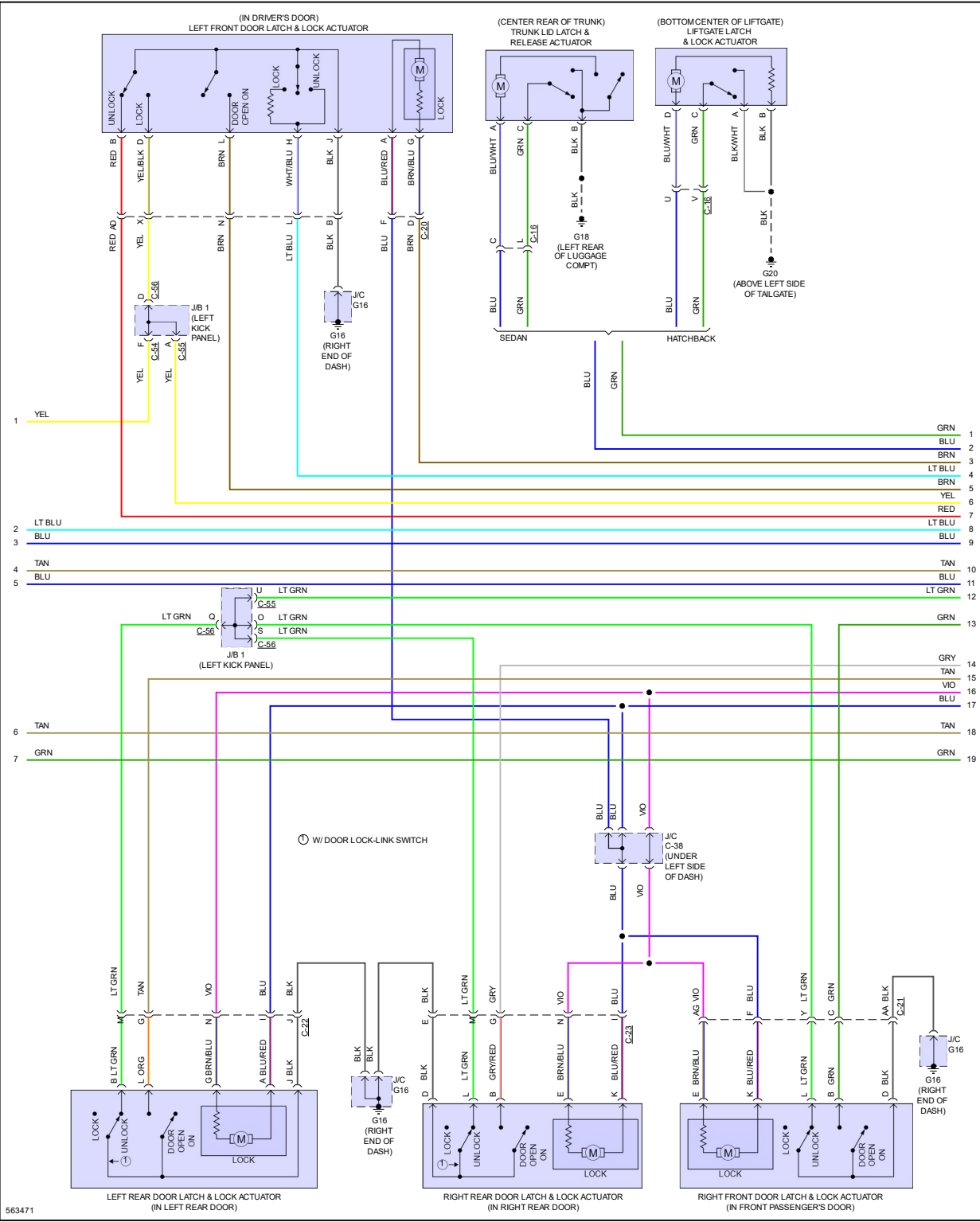
Fig 3: Anti-theft Circuit (3 of 5)
