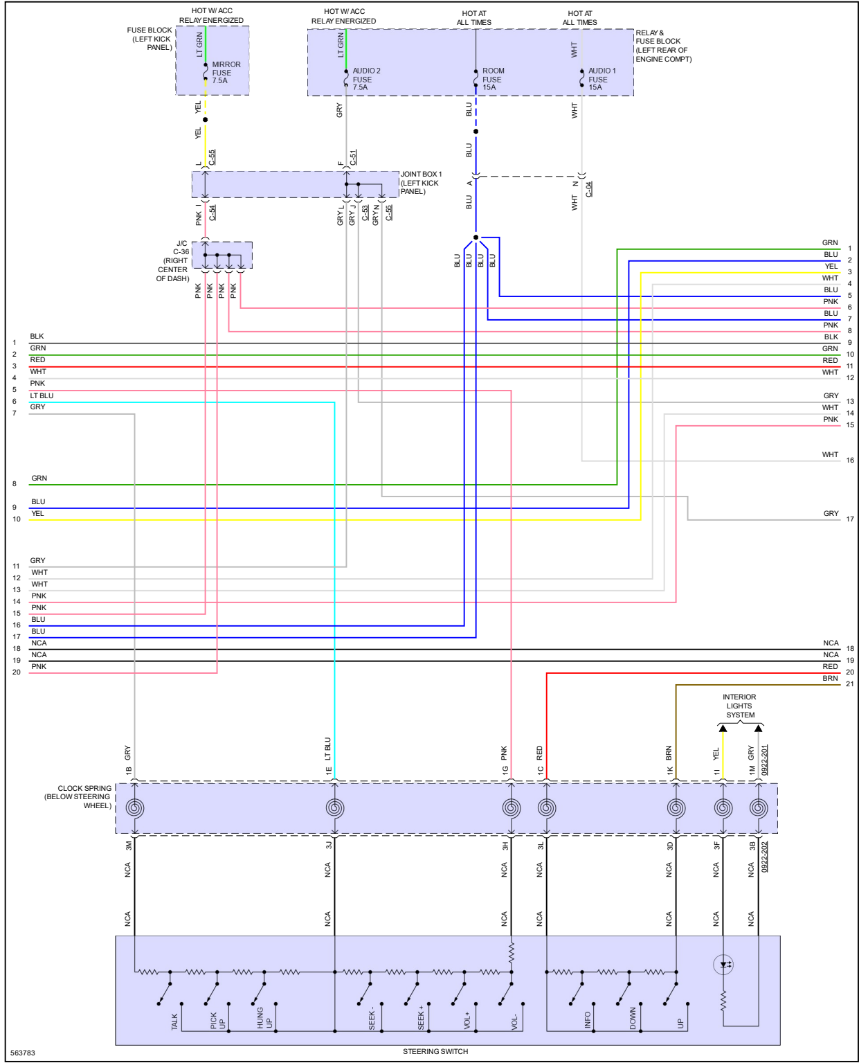
Fig 4: Navigation Circuit, W/ Bose (2 of 5)
