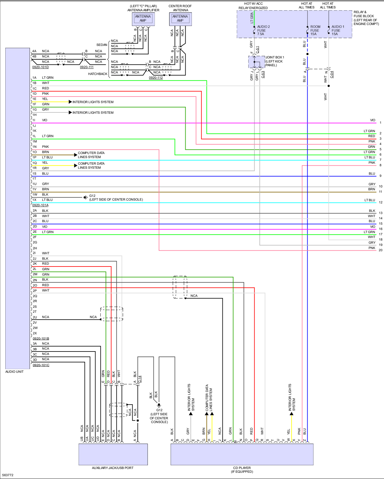
Fig 9: Radio Circuit, W/O Bose W/O Center Display (1 of 3)
