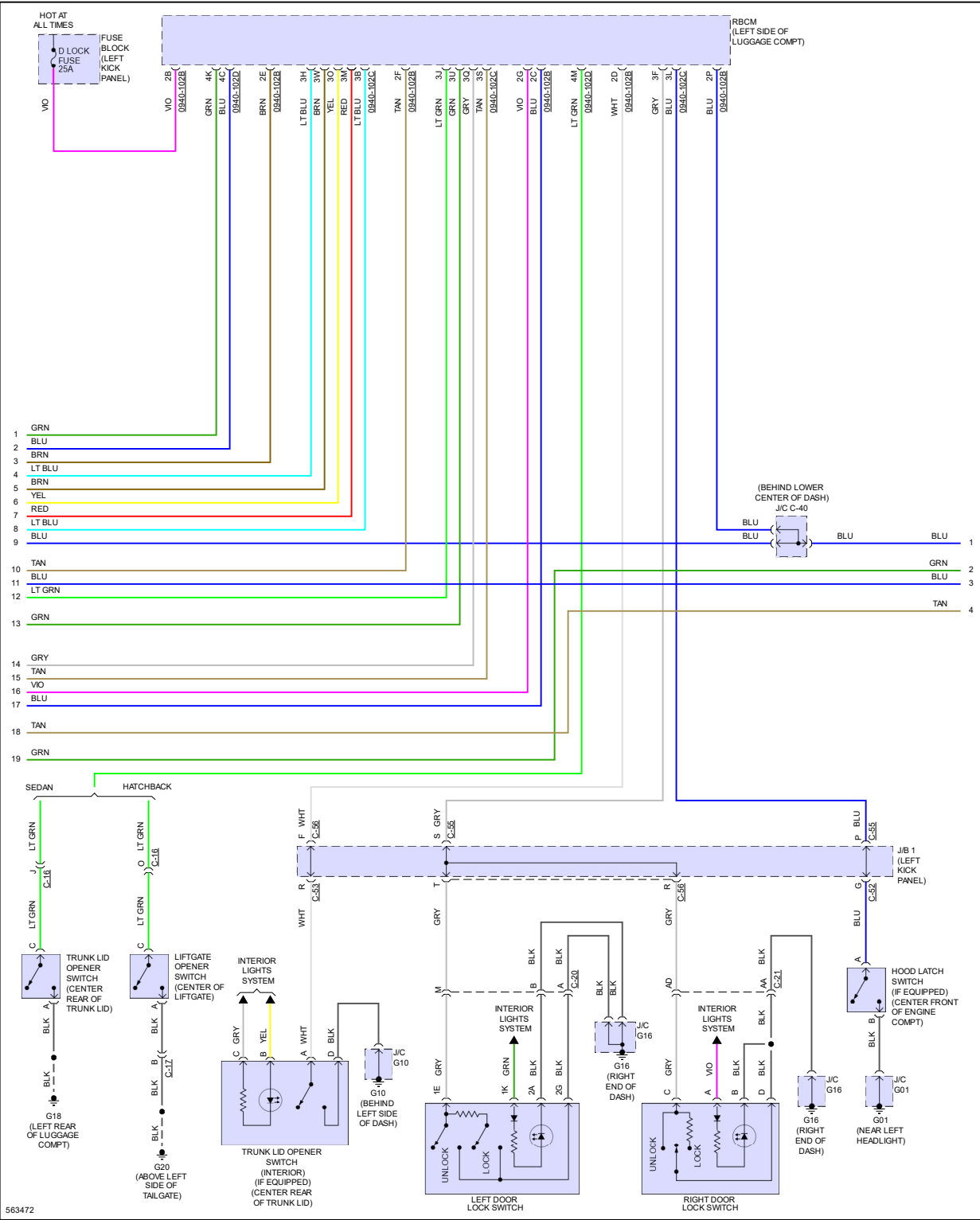
Fig 4: Power Door Locks Circuit (4 of 5)
