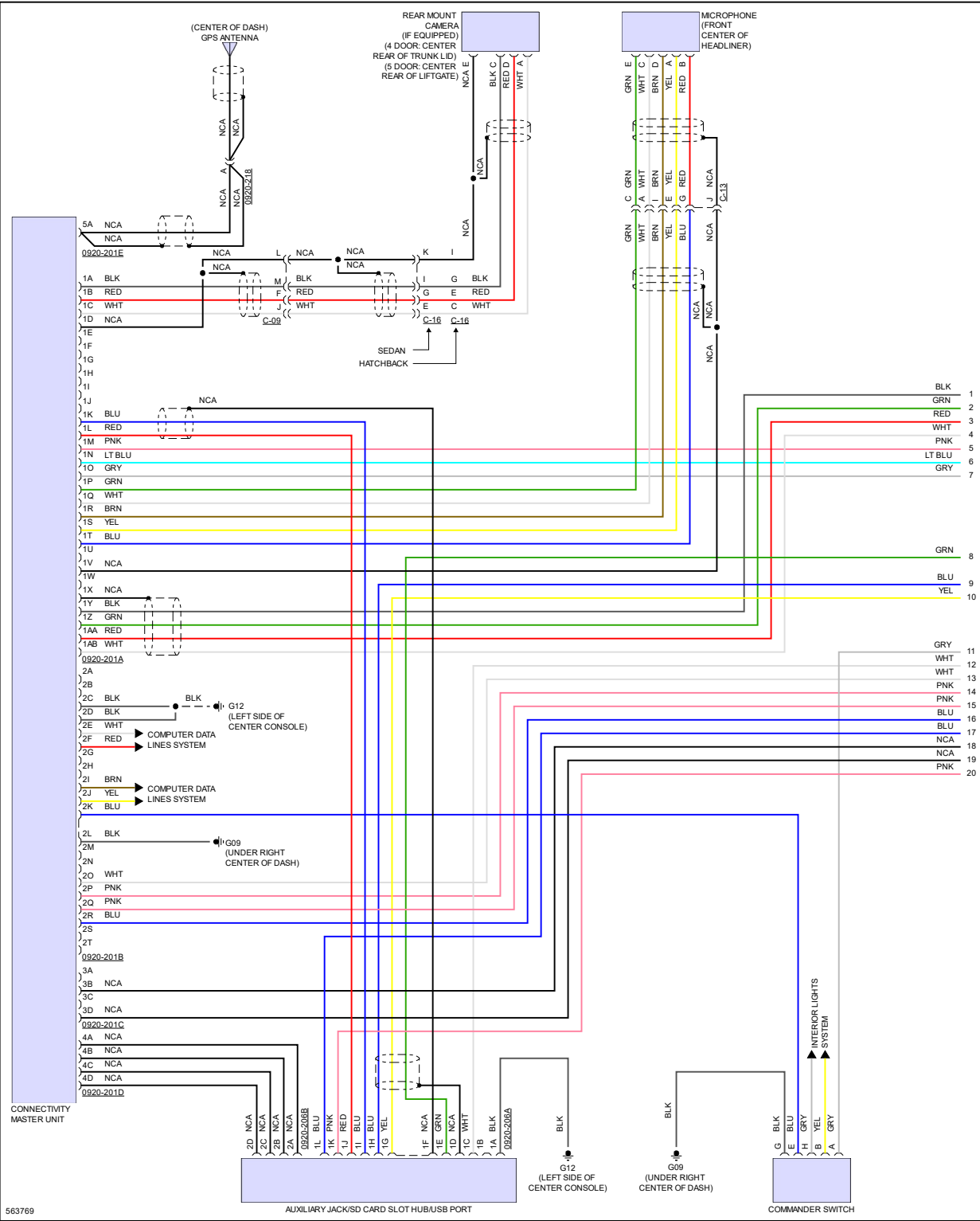
Fig 6: Radio Circuit, W/O Bose W/ Center Display (1 of 3)
