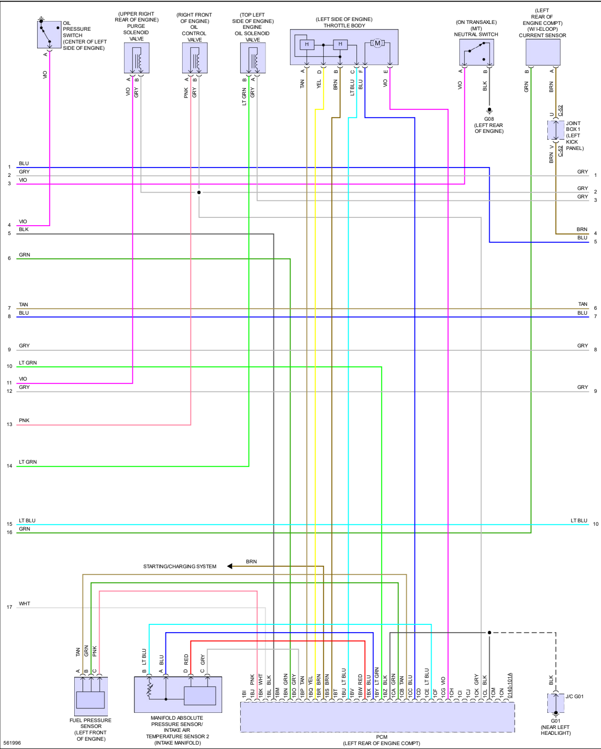
Fig 2: 2.0L SKYACTIV, Engine Performance Circuit (2 of 5)
