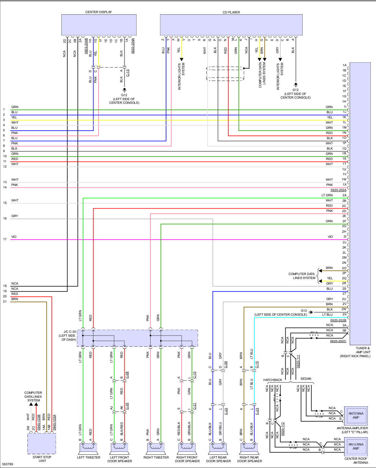
Fig 10: Navigation Circuit, W/O Bose (3 of 3)
