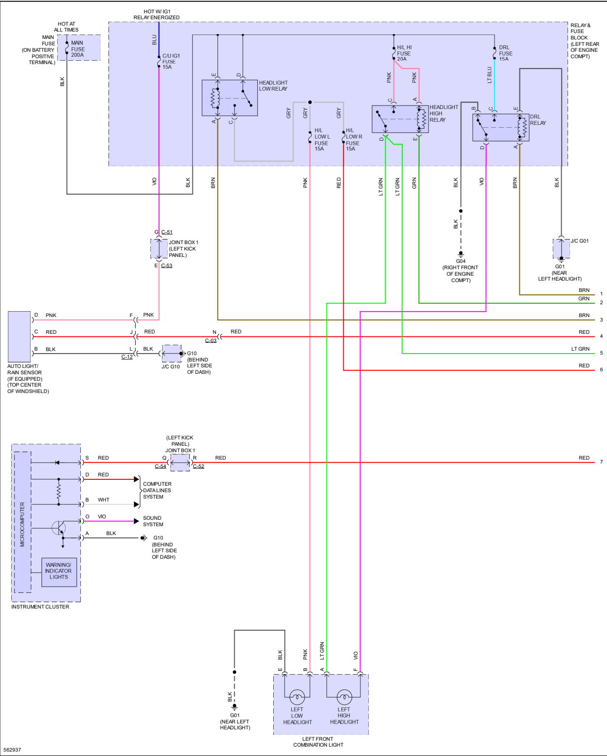
Fig 3: Headlamps Circuit, W/O LED Headlamps (1 of 2)
