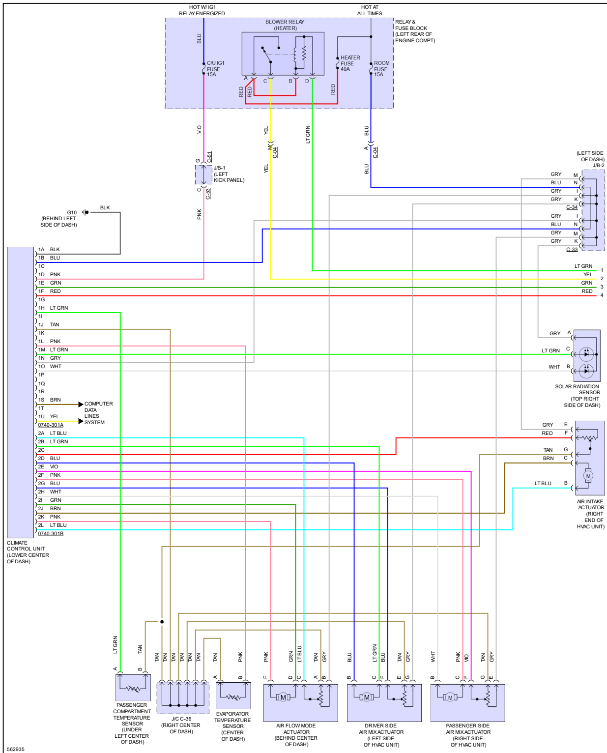
Fig 1: Automatic A/C Circuit, Dual Control (1 of 2)
