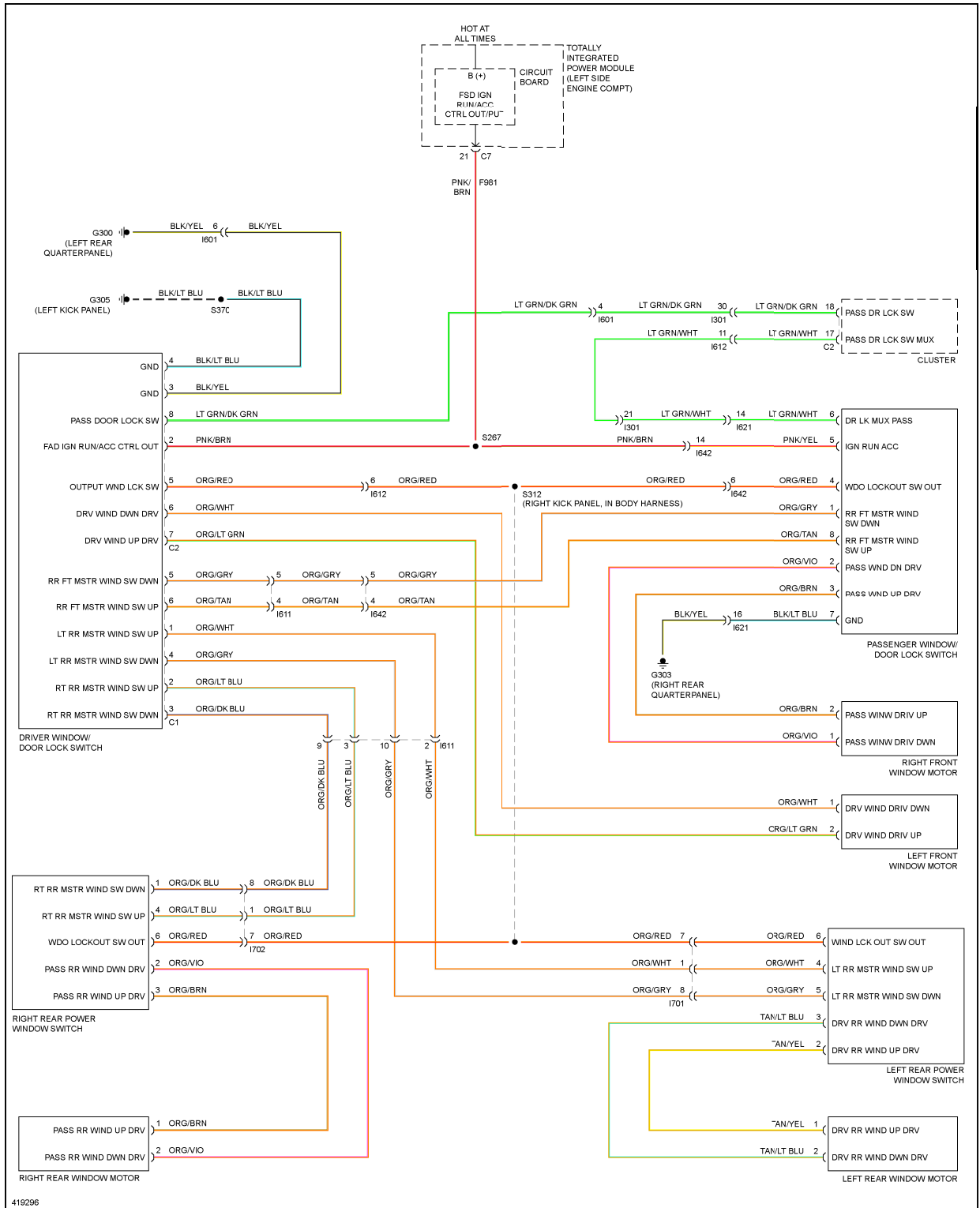
Fig. 50: Power Windows Circuit
