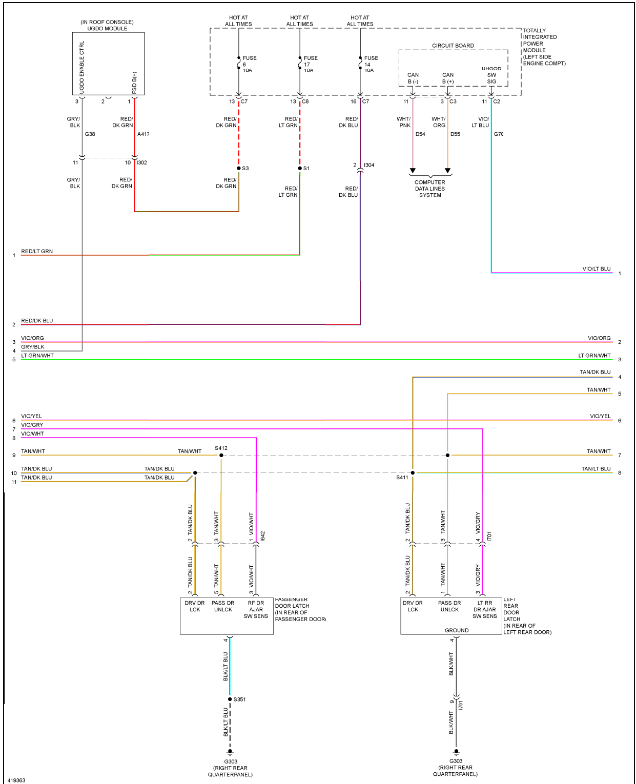
Fig. 5: Anti-theft Circuit (2 of 3)
