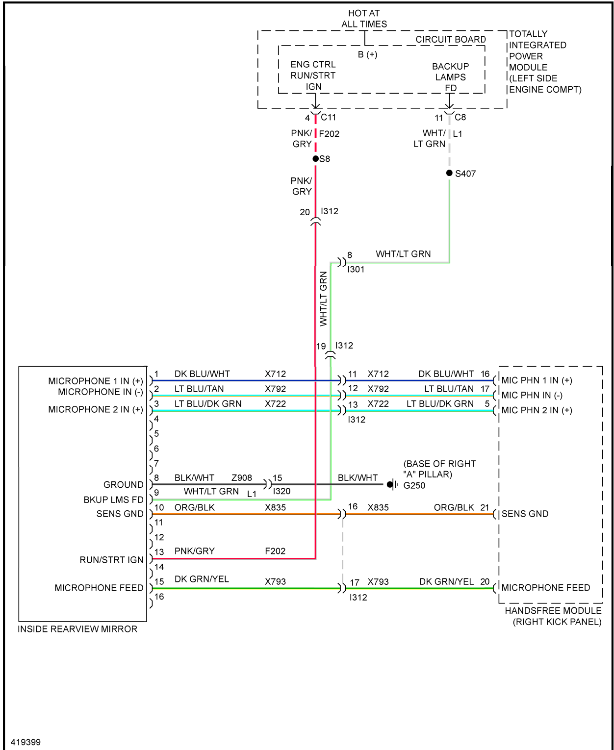
Fig. 45: Automatic Day/Night Mirror Circuit
