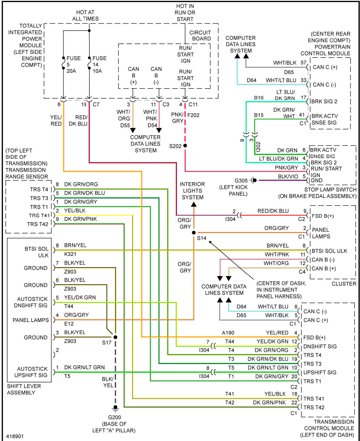
Fig. 57: Shift Interlock Circuit, CVT W/ Autostick
