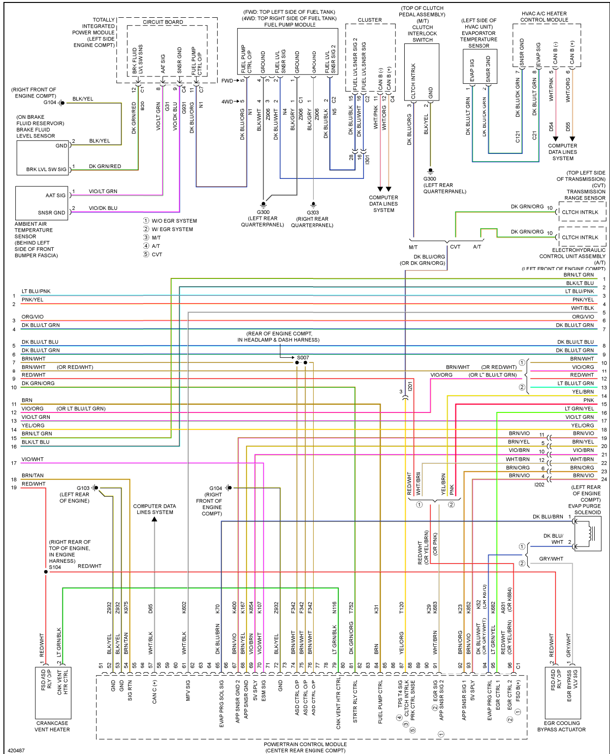
Fig. 19: 2.4L, Engine Performance Circuit (2 of 5)
