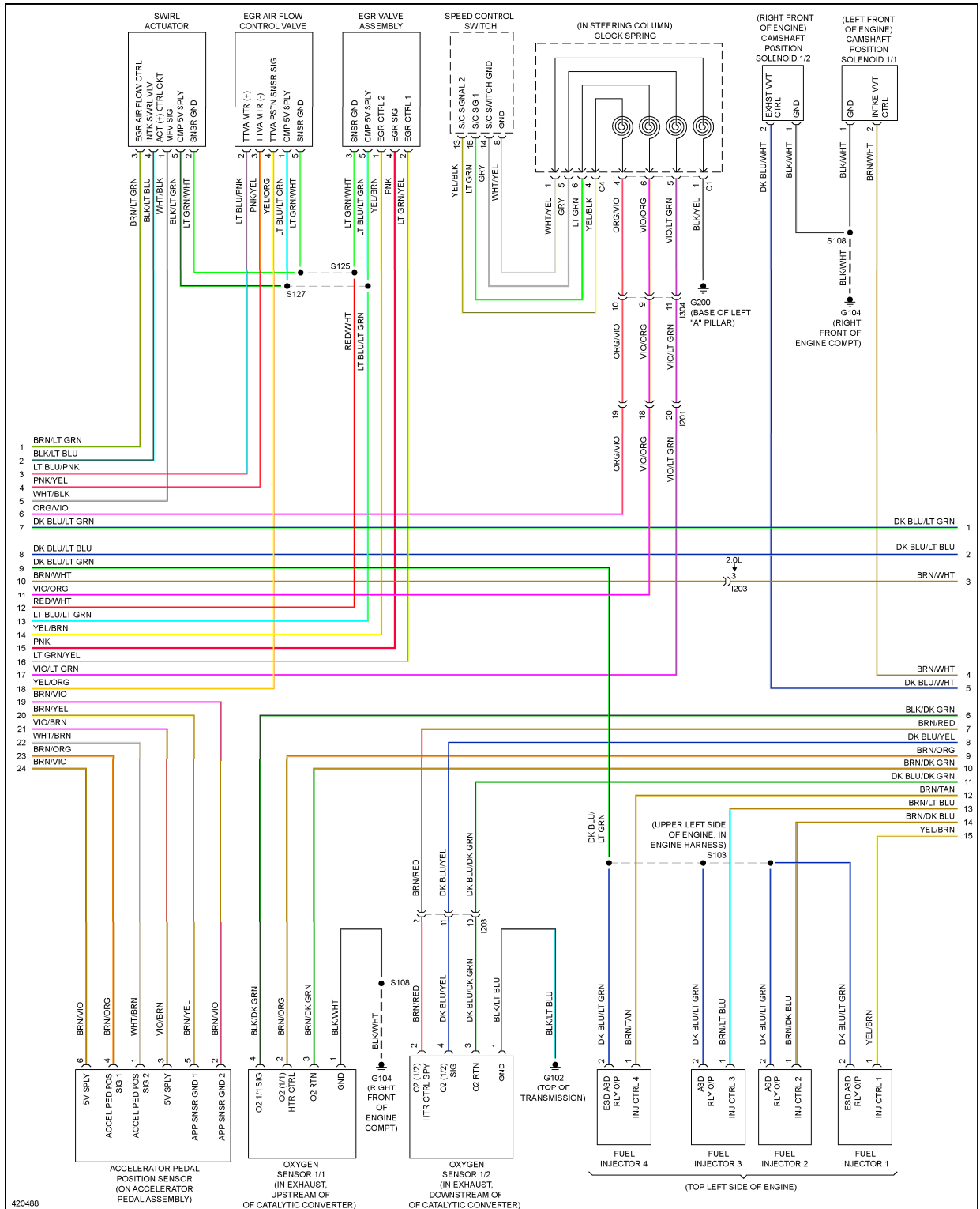
Fig. 15: 2.0L, Engine Performance Circuit (3 of 5)
