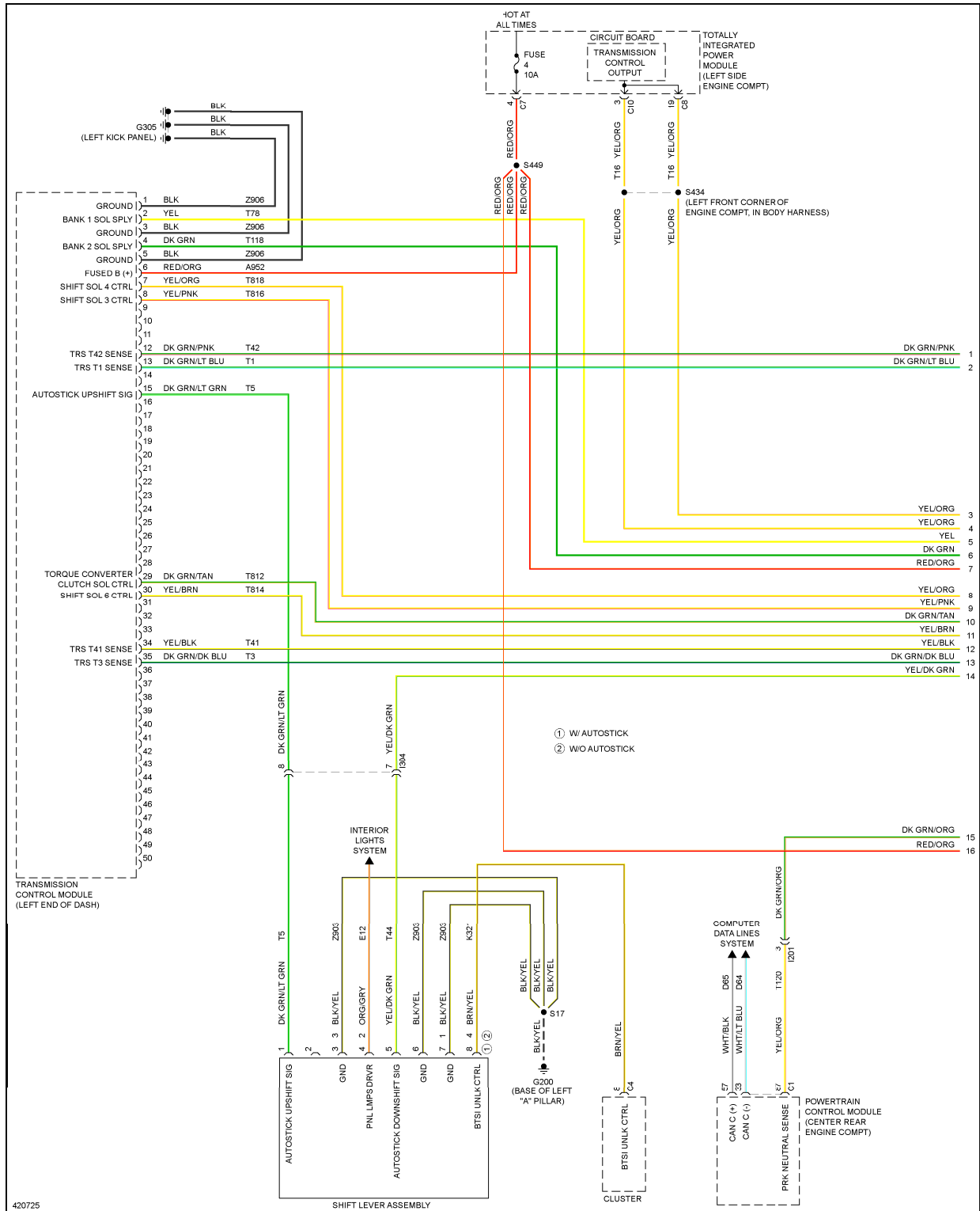
Fig. 64: A/T Circuit, 6 Speed (1 of 2)
