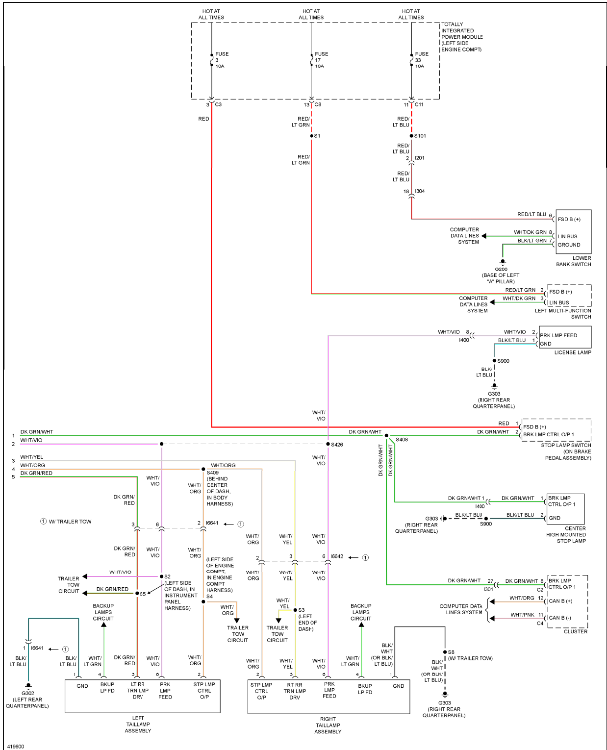
Fig. 25: Exterior Lamps Circuit (2 of 2)
