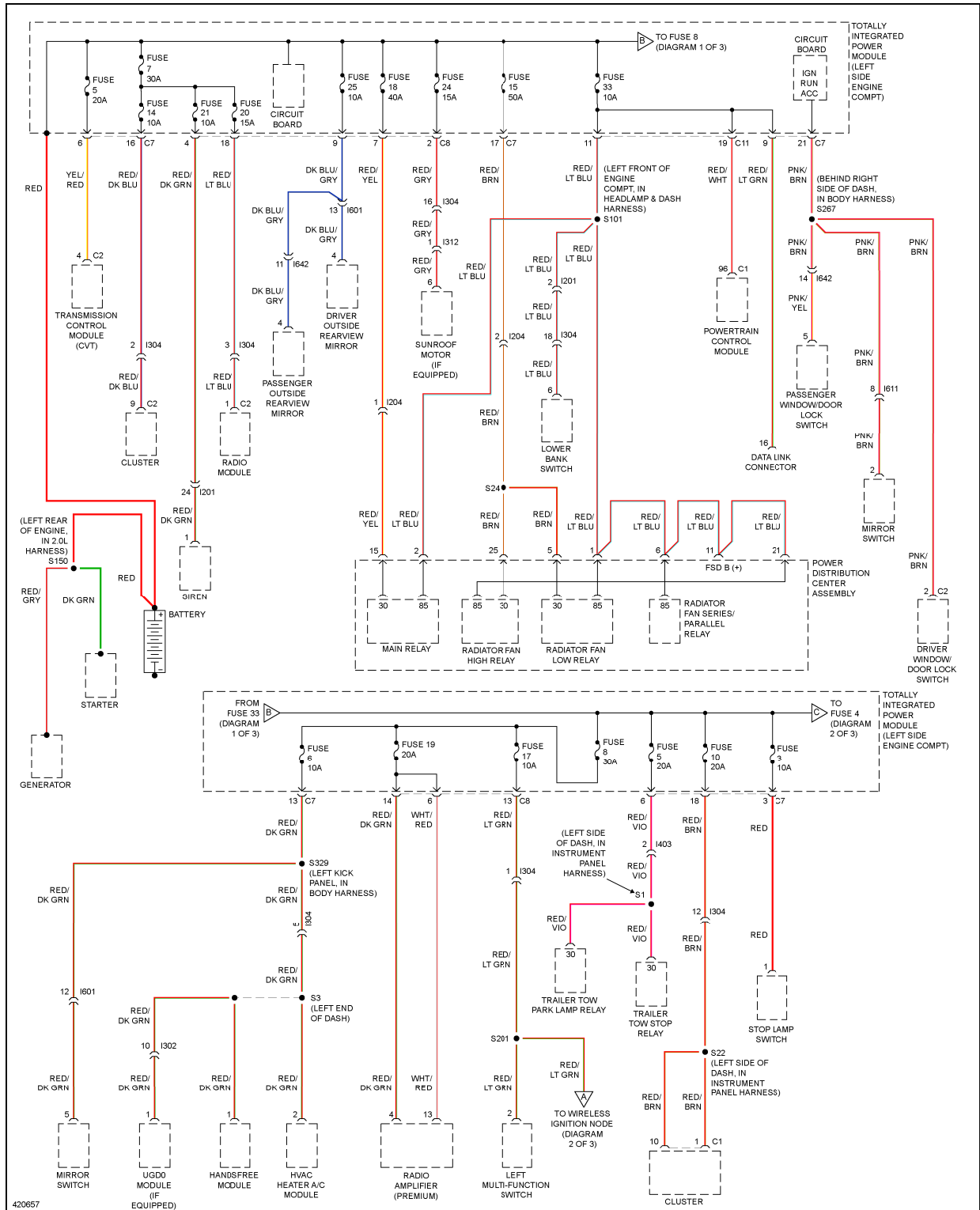
Fig. 39: Power Distribution Circuit (1 of 3)
