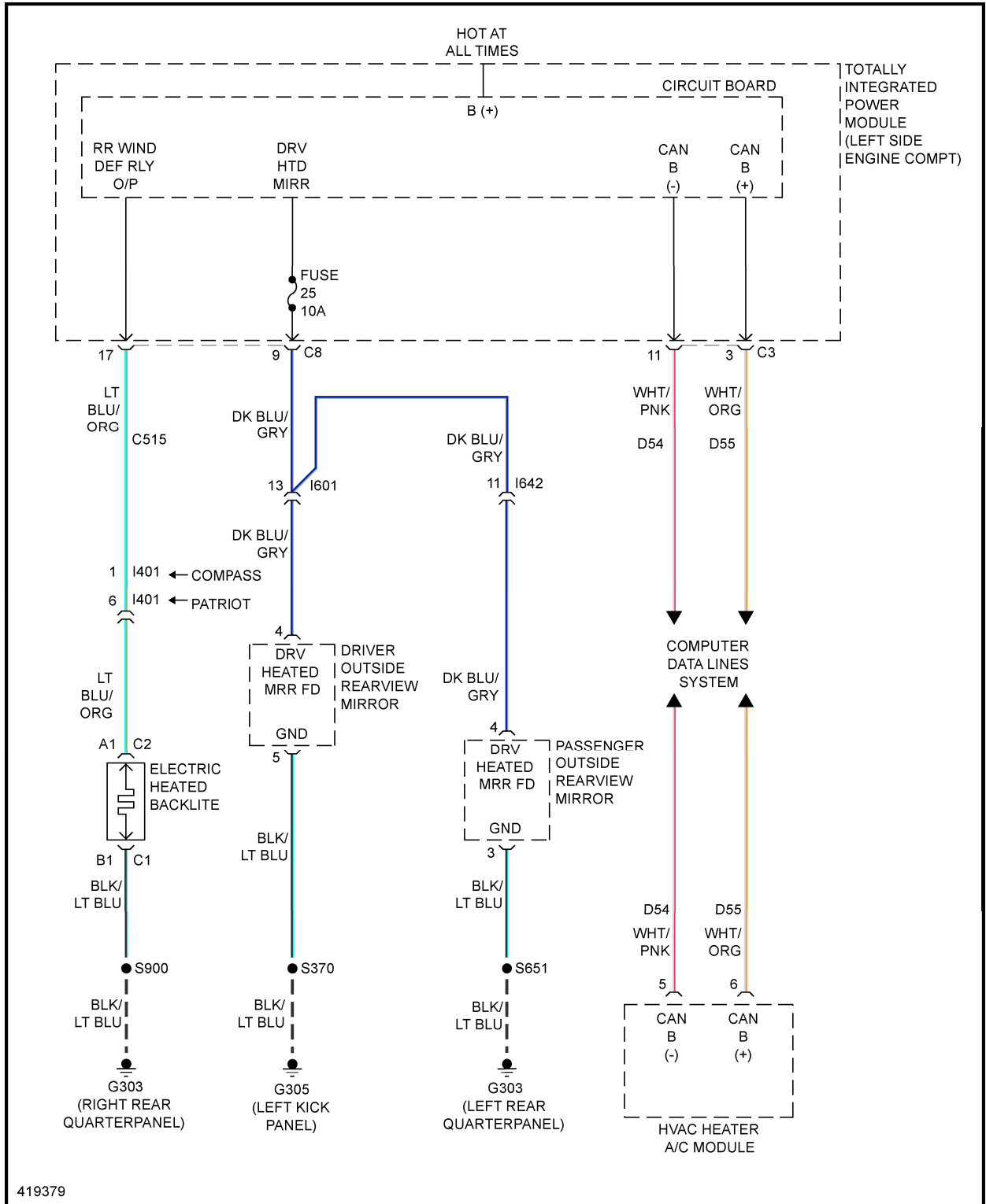
Fig. 12: Defoggers Circuit
