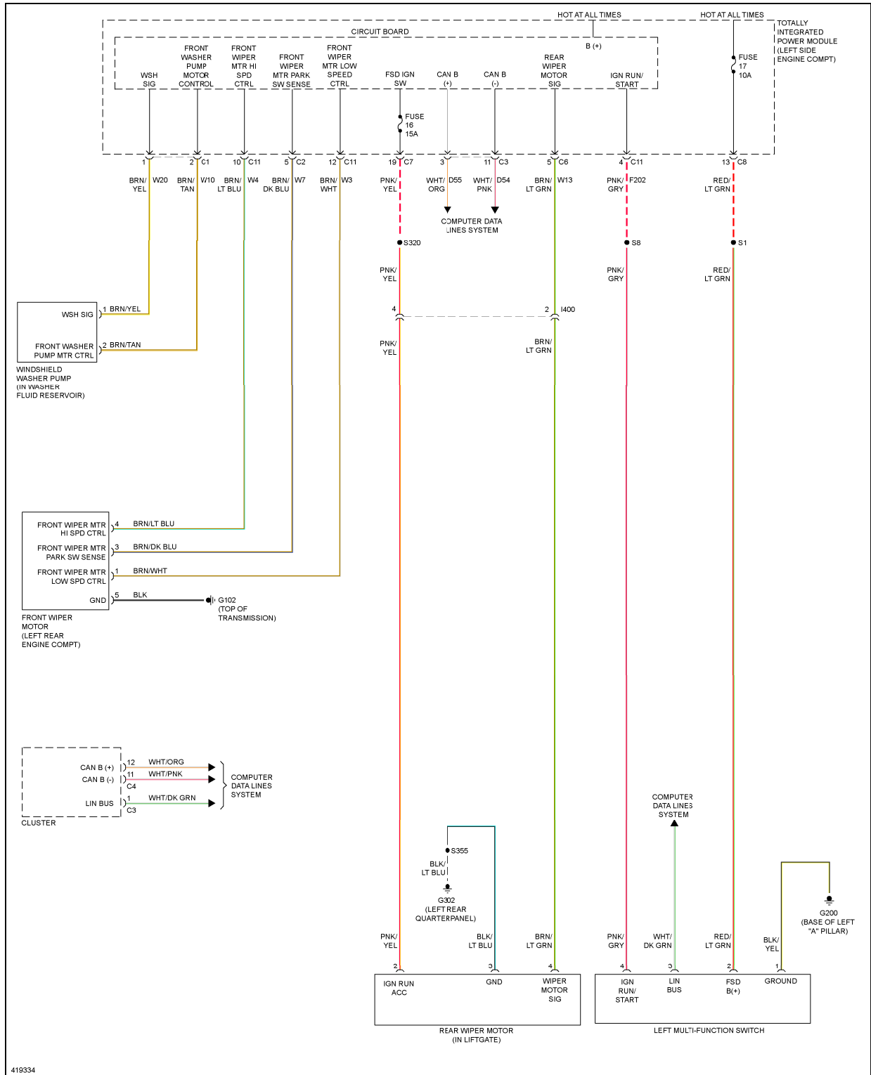
Fig. 69: Wiper/Washer Circuit
