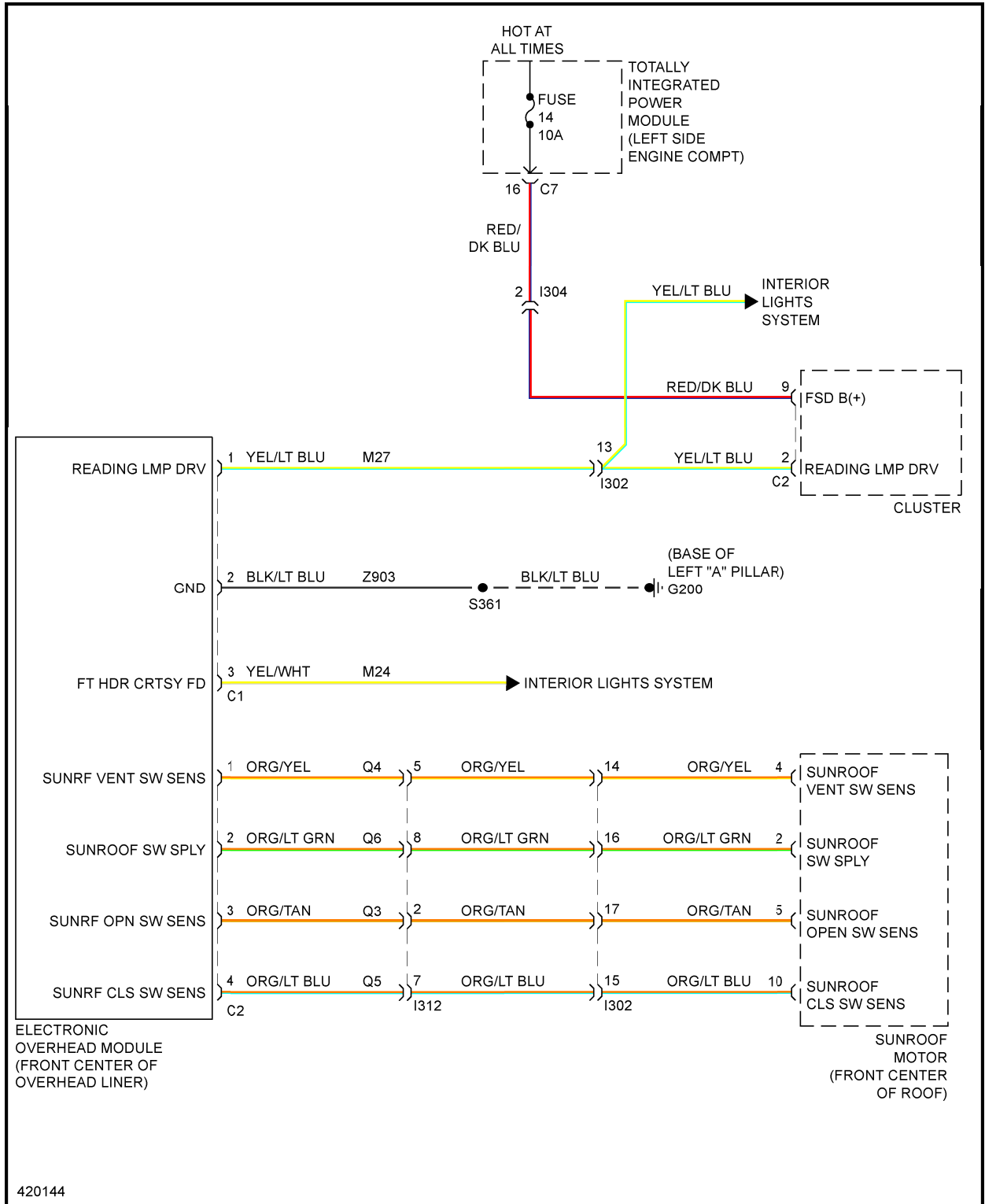
Fig. 33: Overhead Console Circuit
