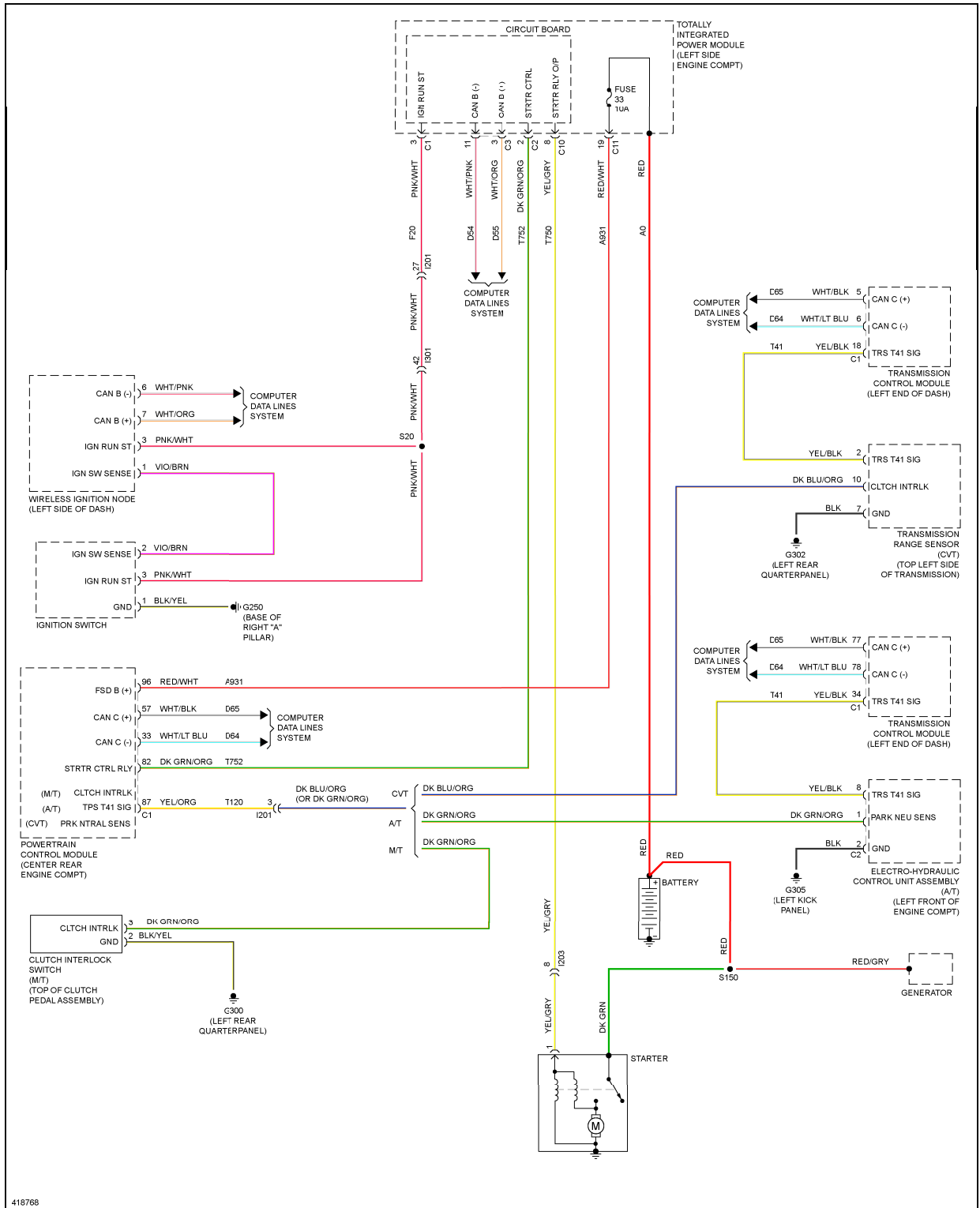
Fig. 60: Starting Circuit
