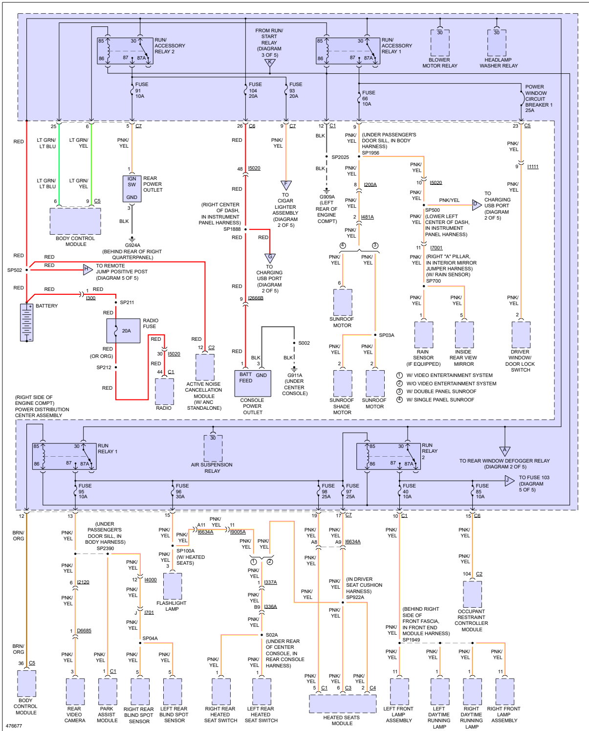
Fig 1: Power Distribution Circuit (1 of 5)
