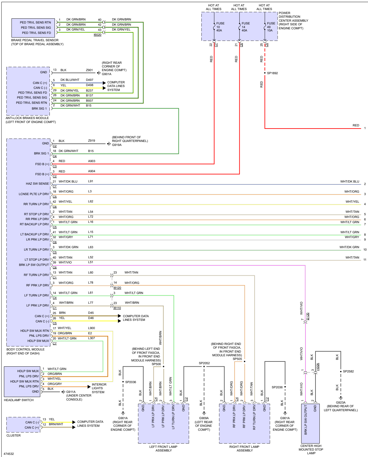
Fig 2: Exterior Lamps Circuit, Base (1 of 2)
