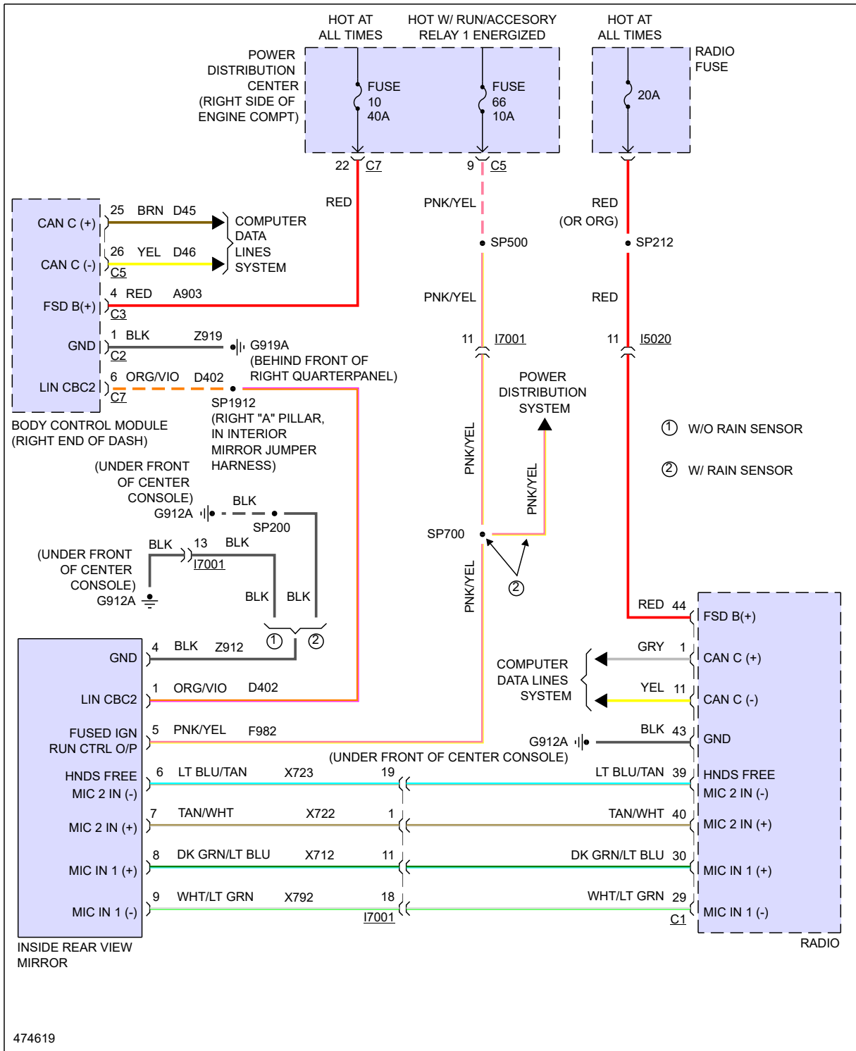
Fig 1: Automatic Day/Night Mirror Circuit
