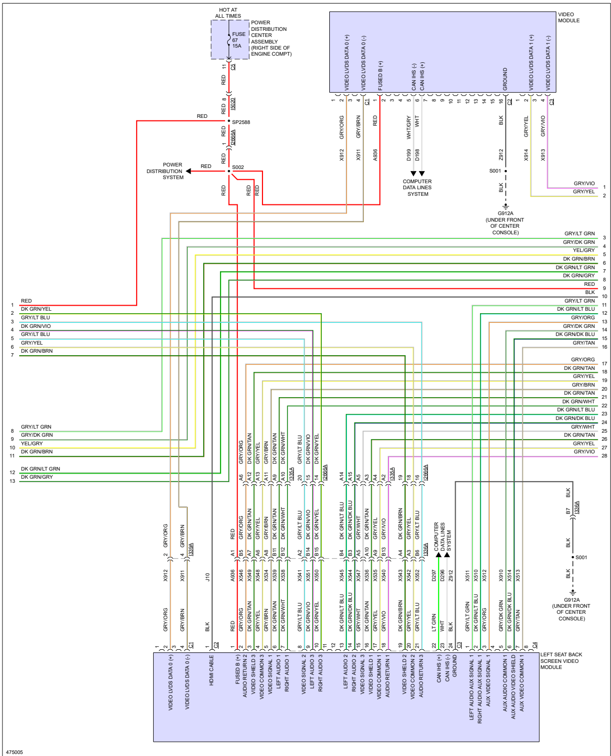
Fig 5: Navigation Circuit, Premium 2 W/ ANC Stand Alone (4 of 6)
