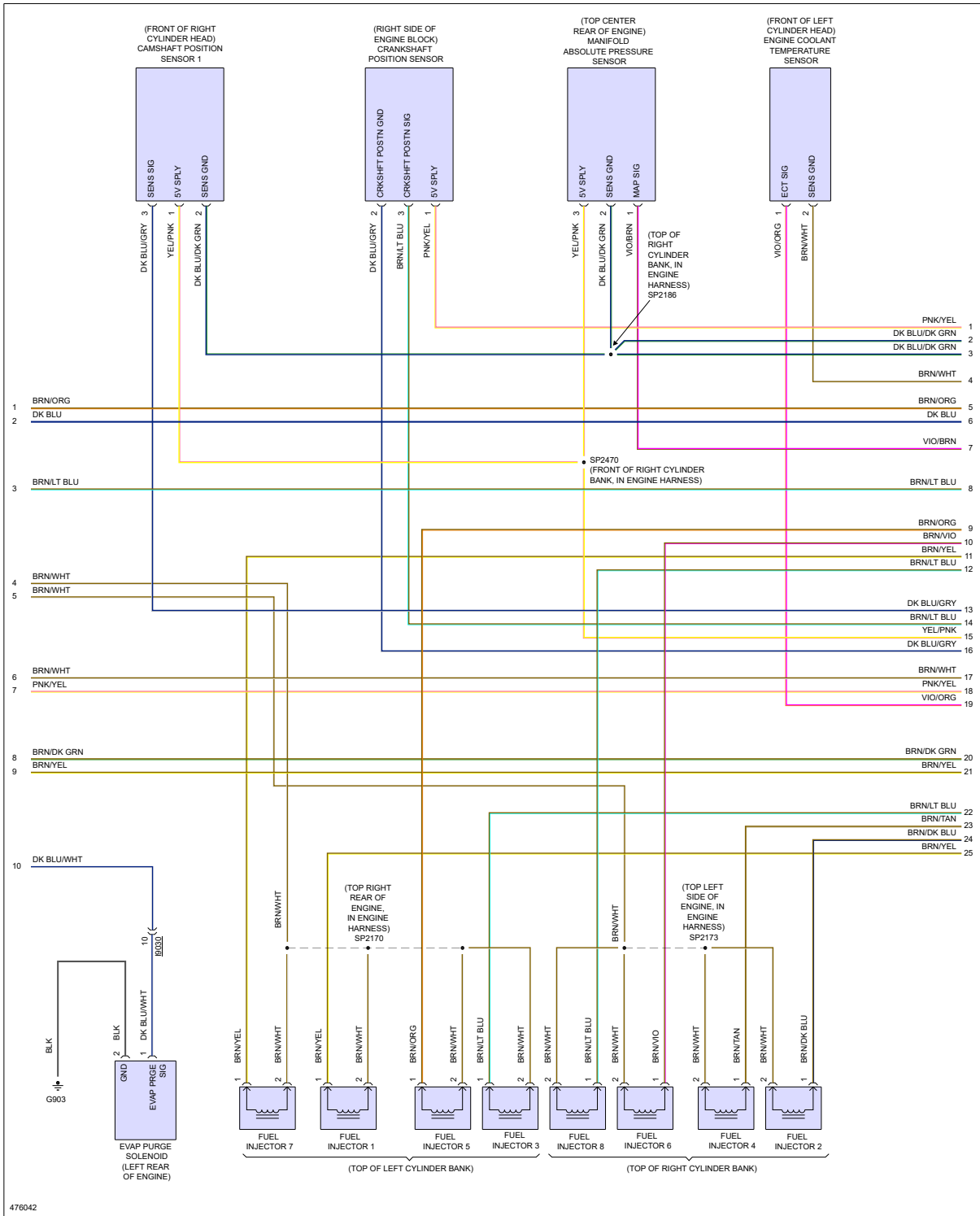
Fig 4: 6.4L, Engine Performance Circuit (4 of 6)
