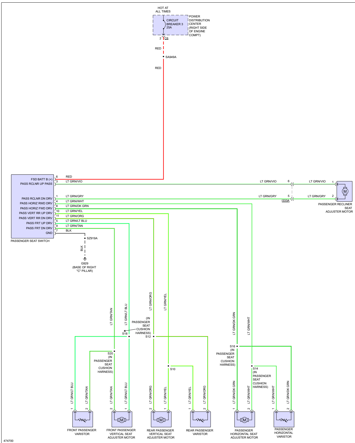
Fig 6: Passenger Power Seat Circuit
