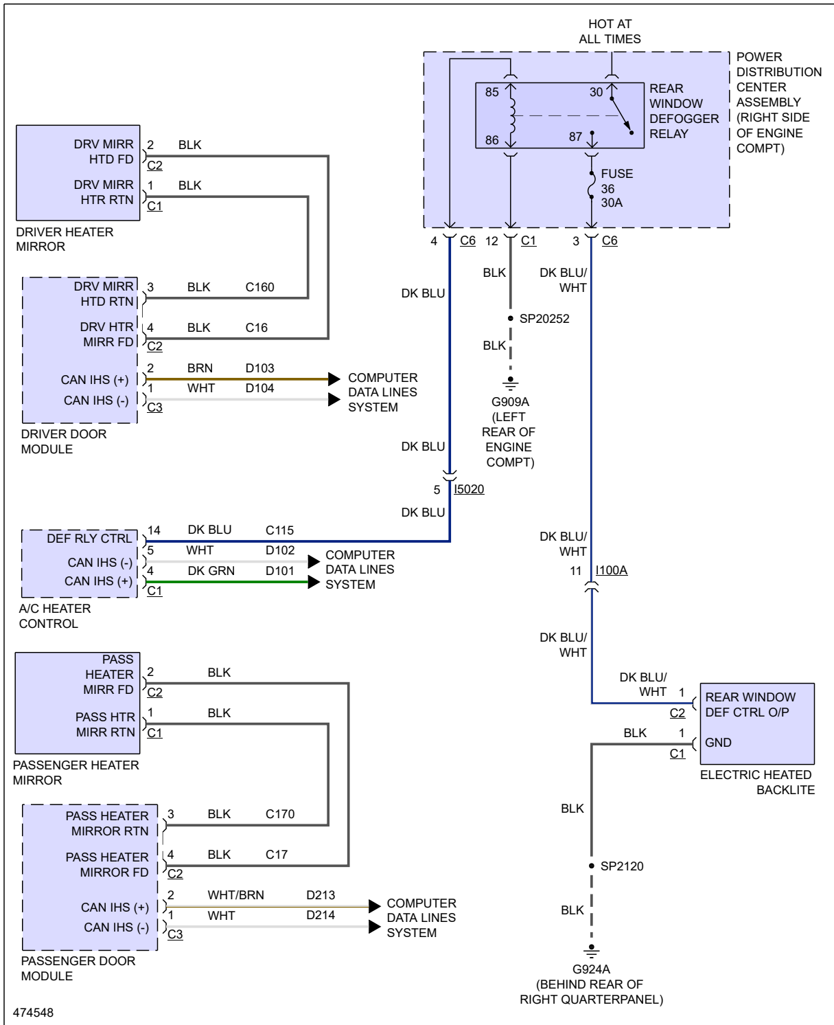
Fig 1: Defoggers Circuit
