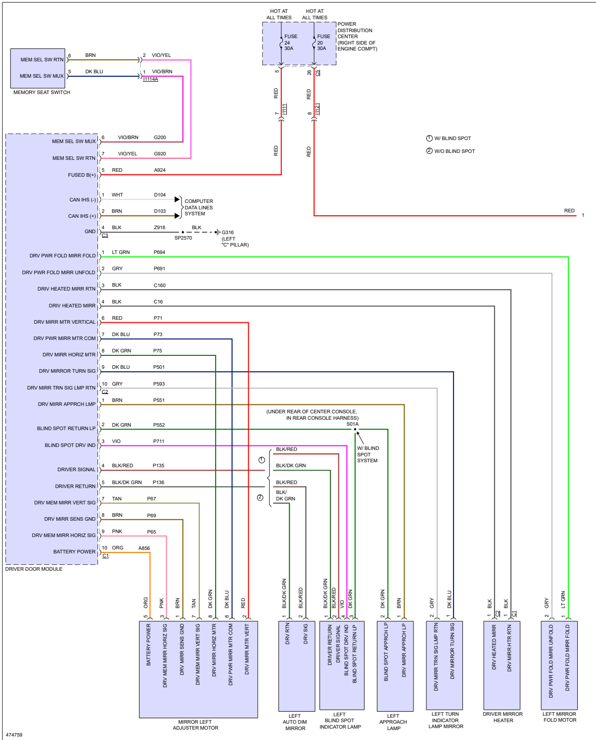
Fig 1: Memory Mirrors Circuit (1 of 2)
