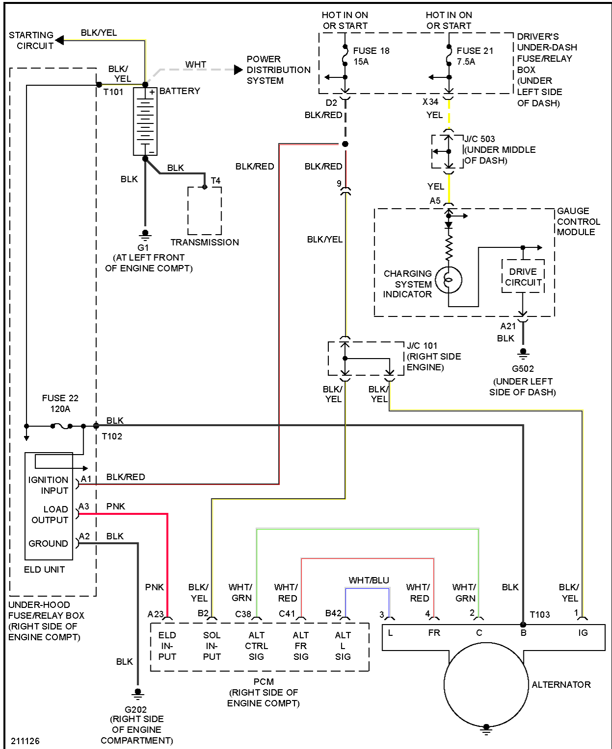
Fig. 86: Charging Circuit
