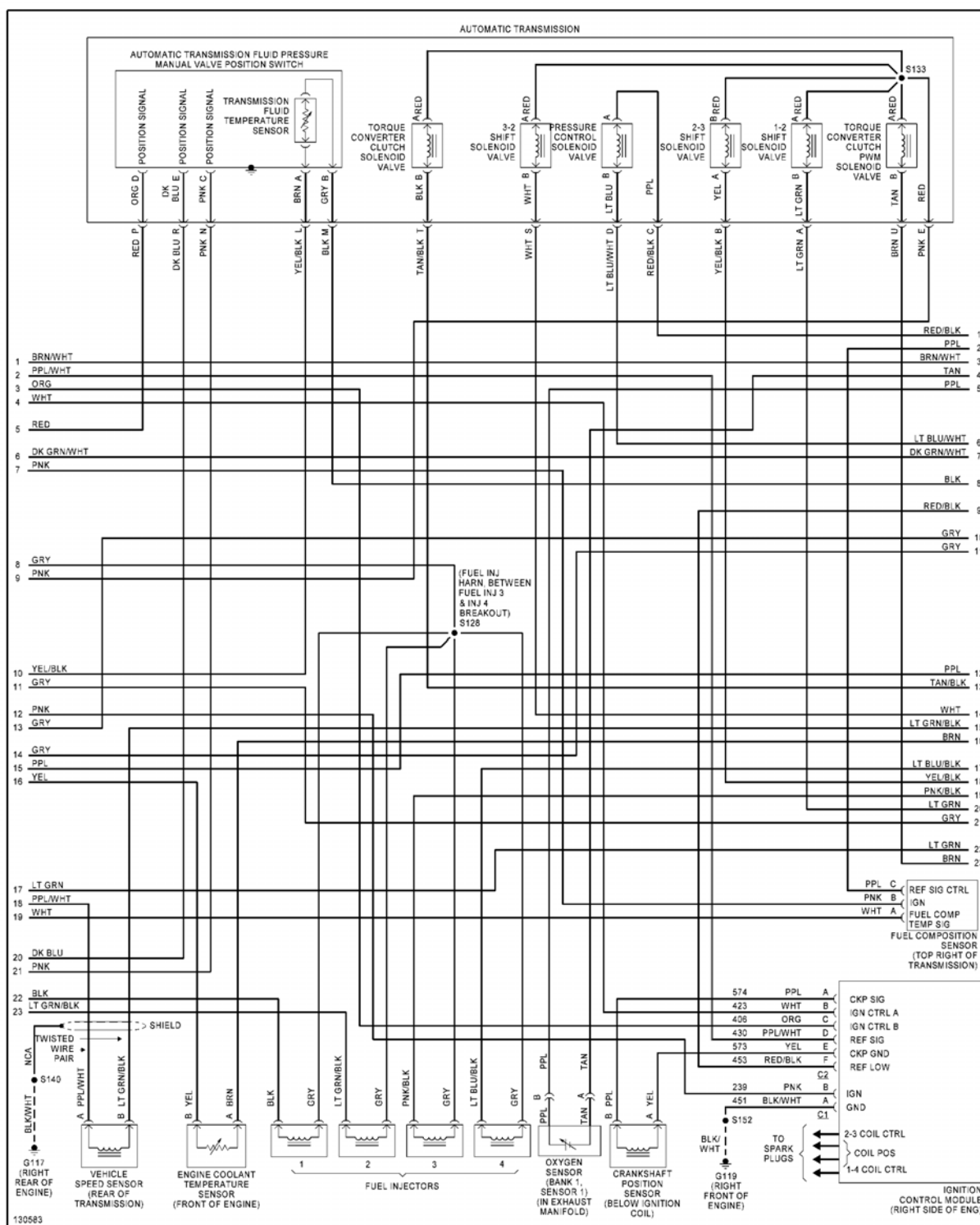
Fig. 17: 2.2L VIN 5, Engine Performance Circuits (2 of 3)
