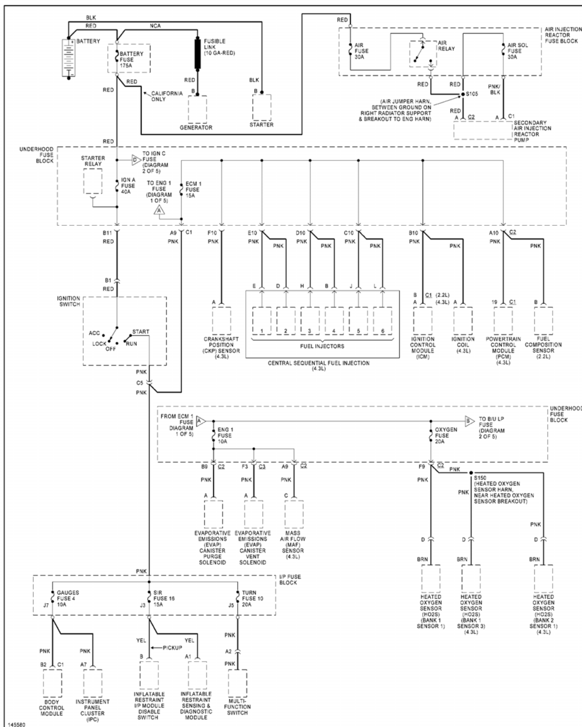
Fig. 35: Power Distribution Circuit (1 of 5)
