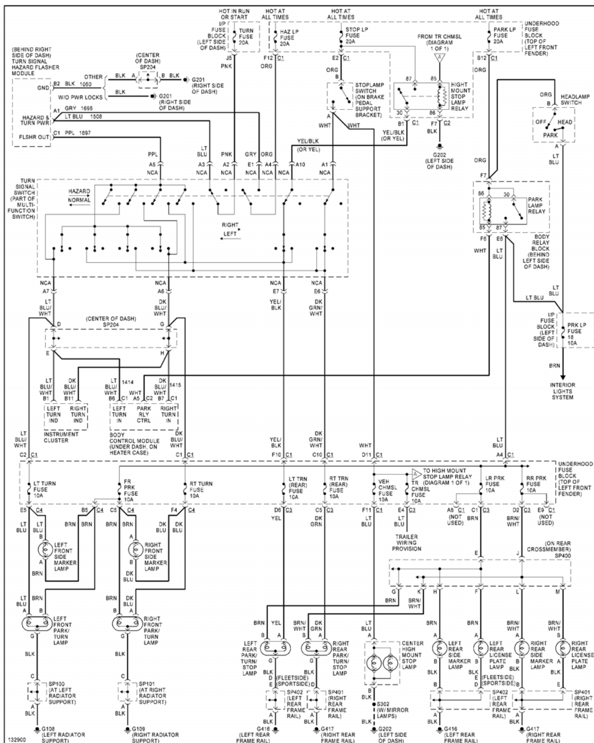
Fig. 24: Exterior Lamps Circuit
