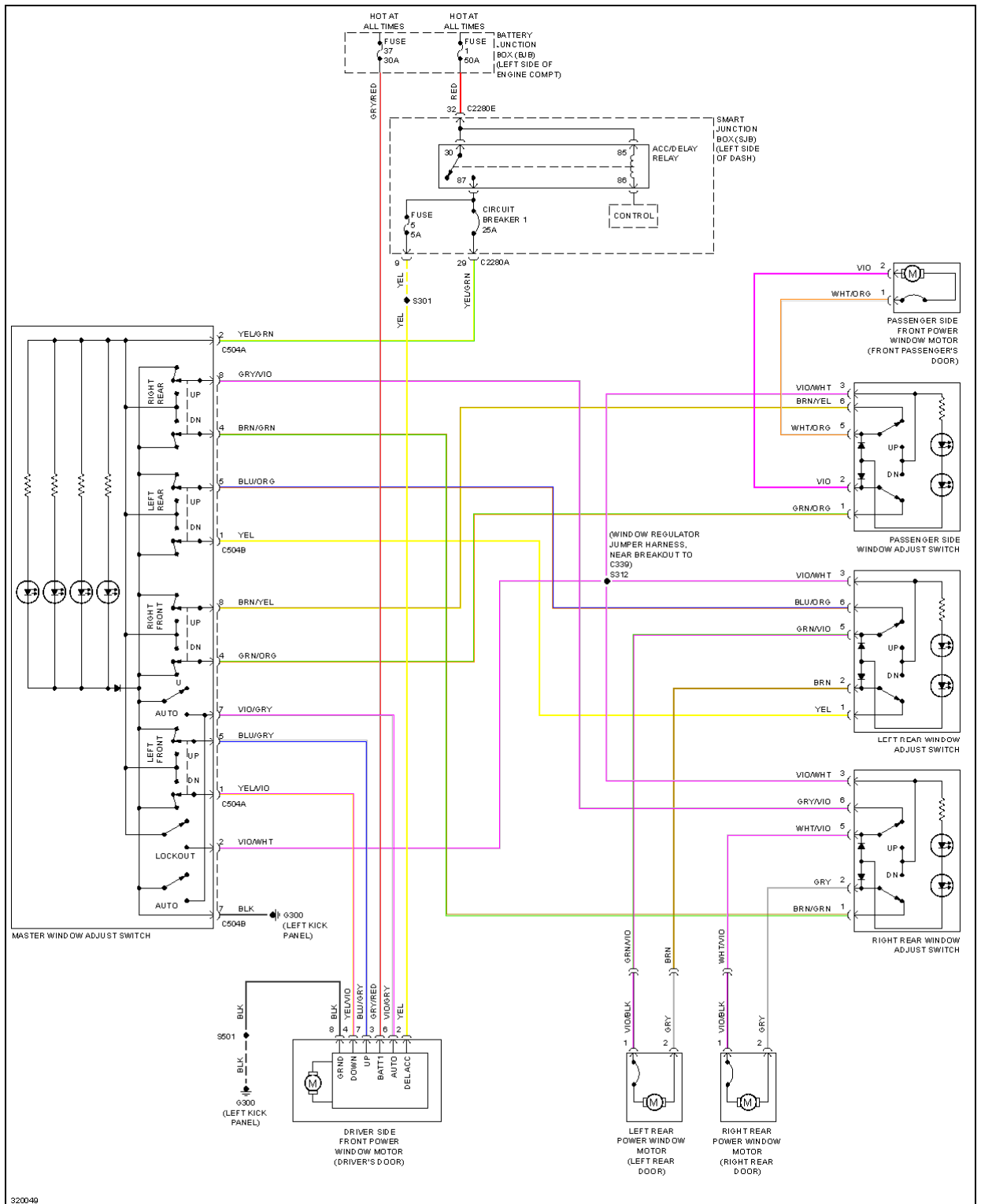
Fig. 61: Power Windows Circuit
