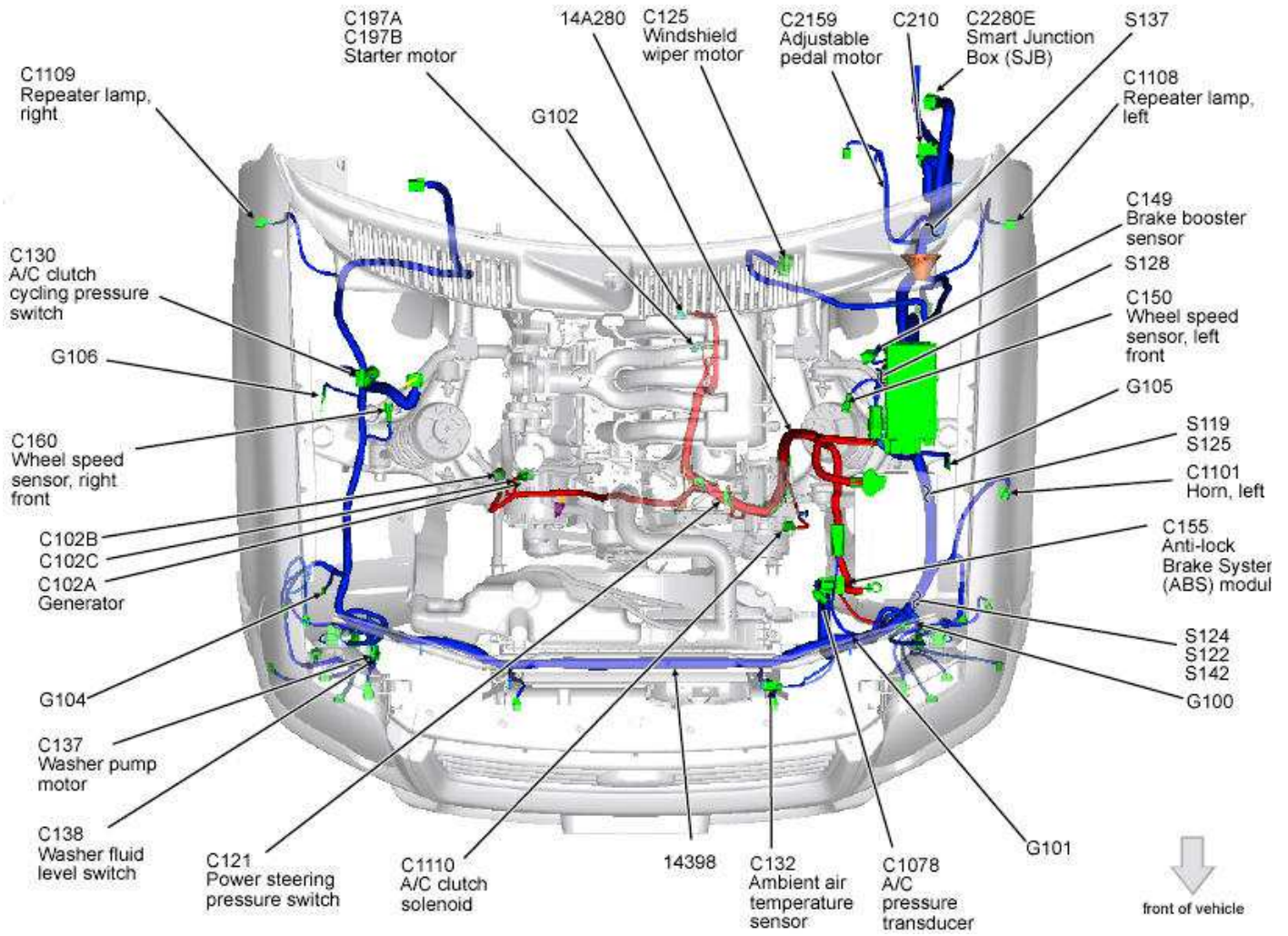
Fig. 4: Engine Compartment (4.0L)
