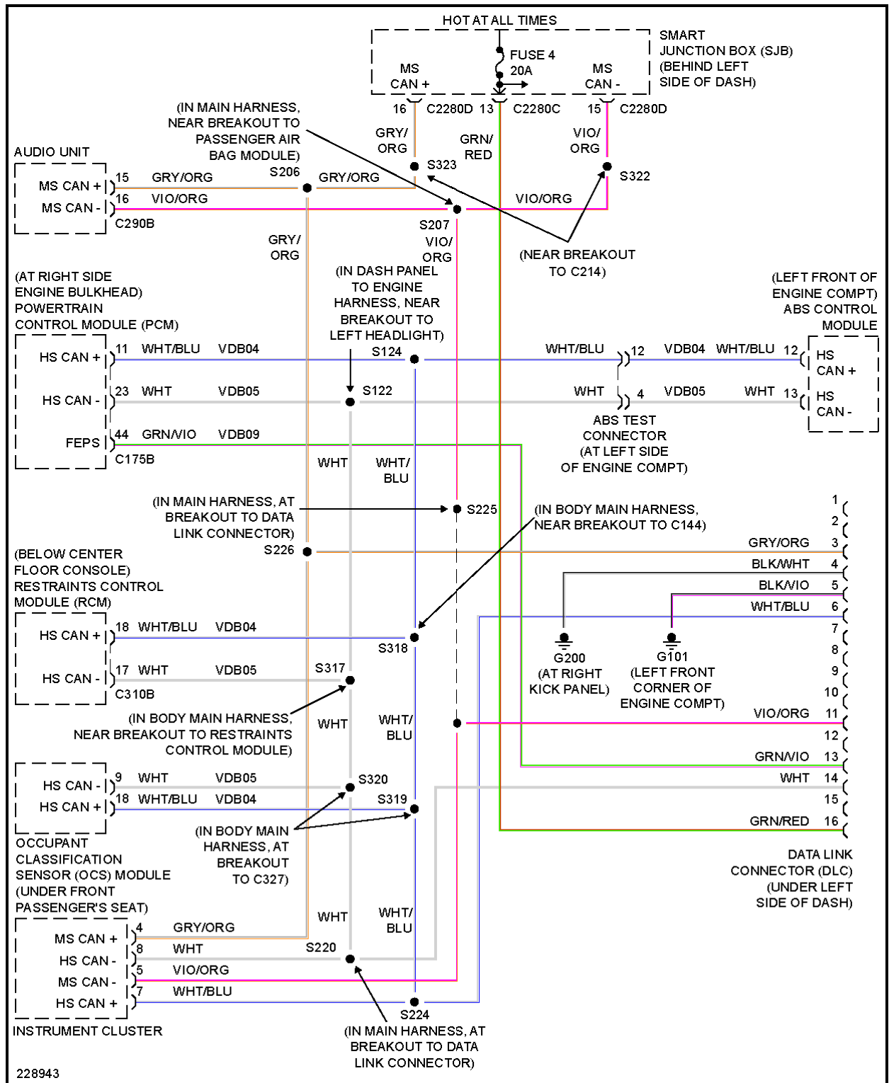
Fig. 9: 4.0L, Computer Data Lines Circuit
