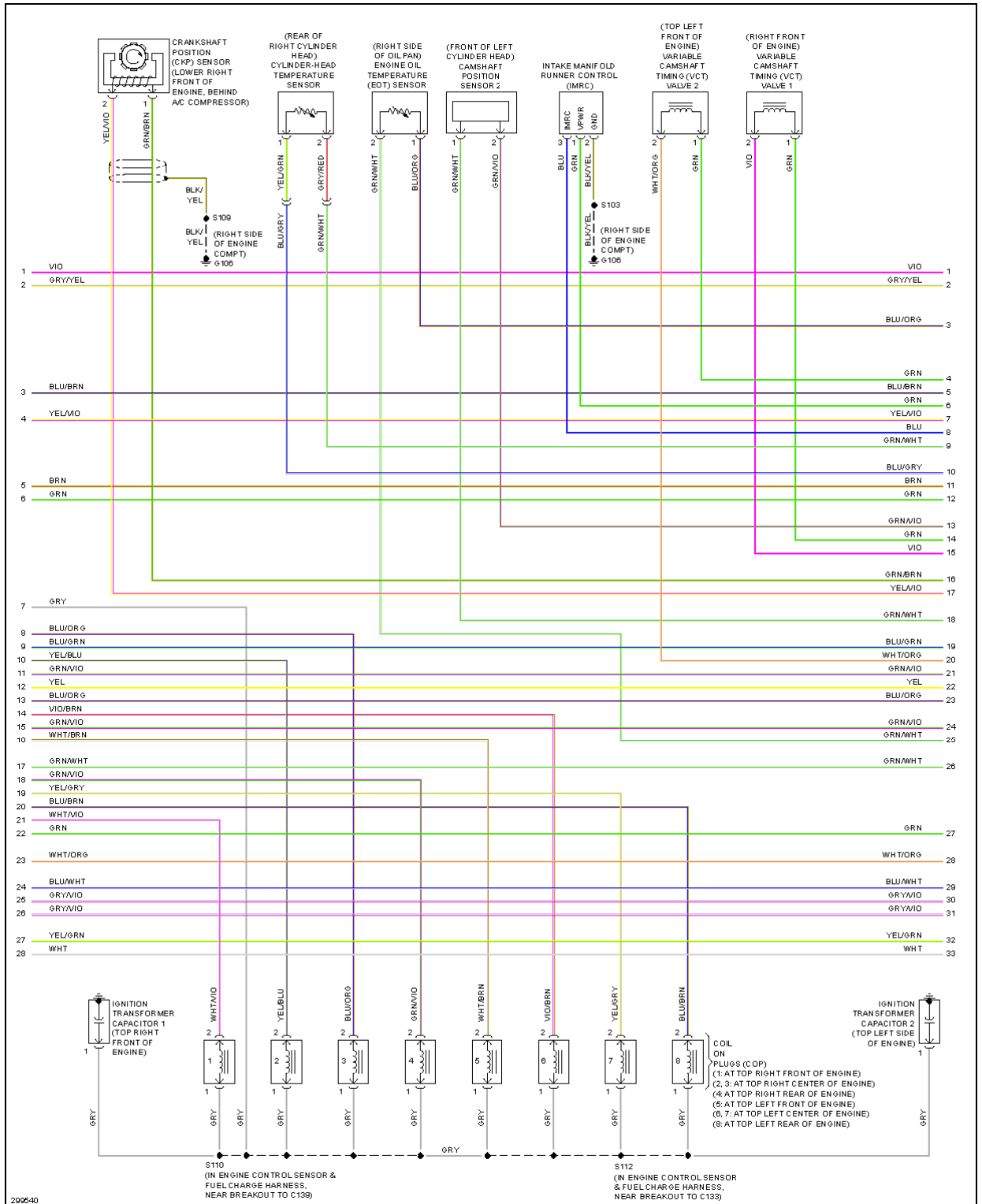
Fig. 22: 4.6L, Engine Performance Circuit (4 of 5)
