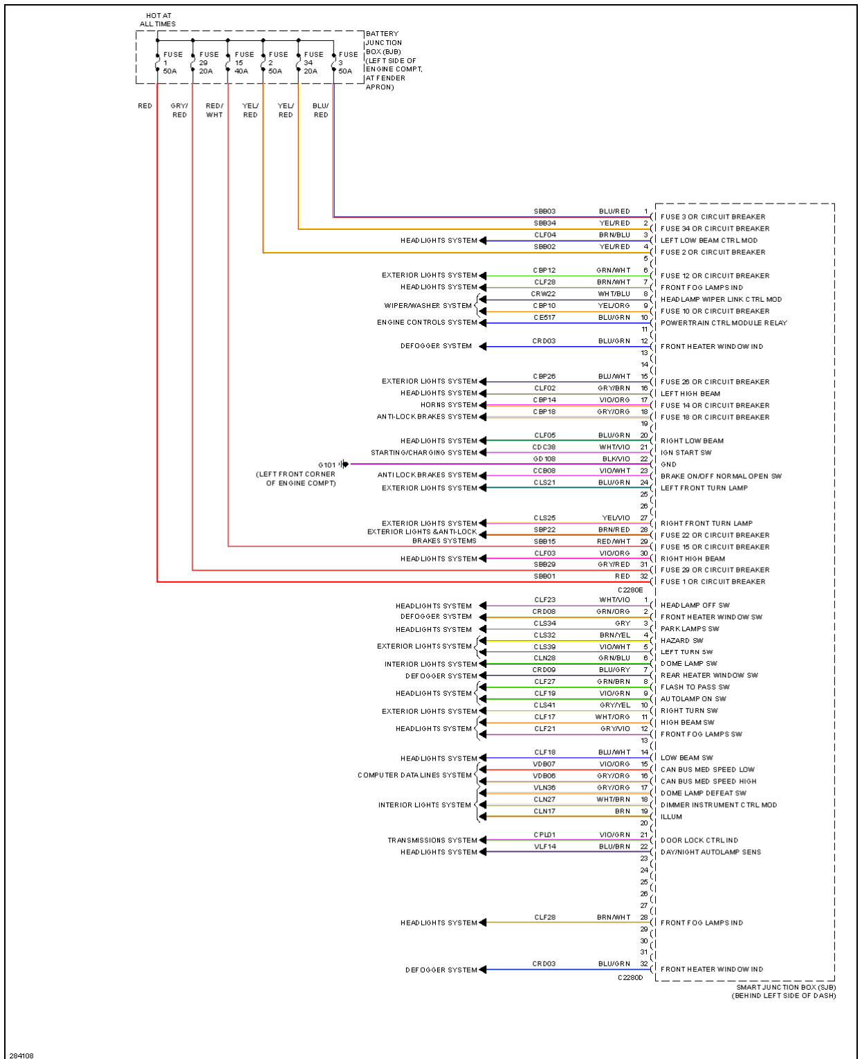
Fig. 8: Body Control Modules Circuit (2 of 2)
