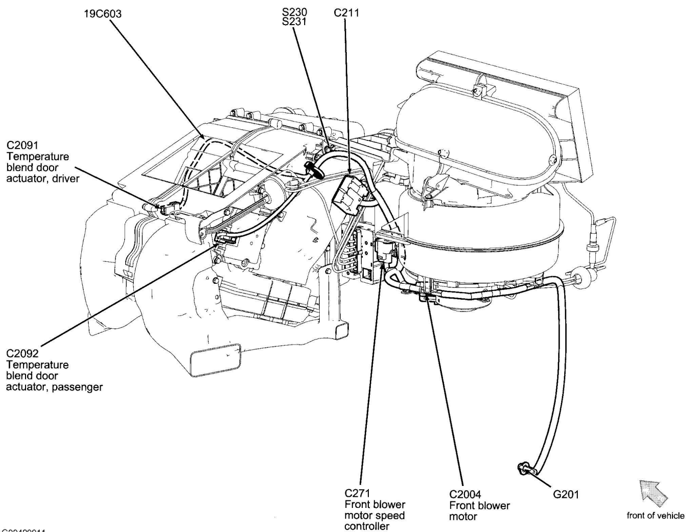
Fig. 25: Front Of HVAC Unit (DEATC)
