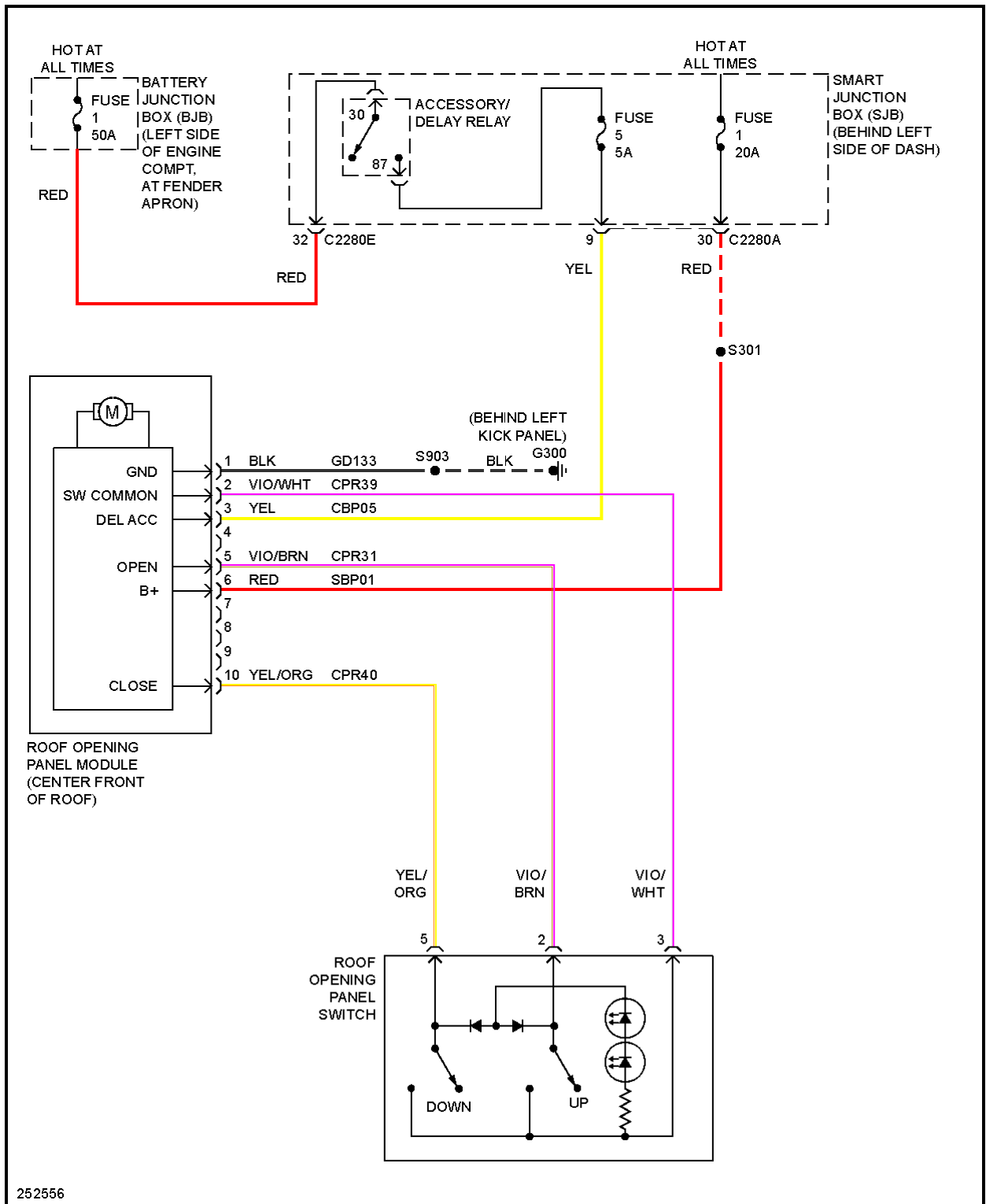
Fig. 59: Power Top/Sunroof Circuit, W/O Medium Overhead Console
