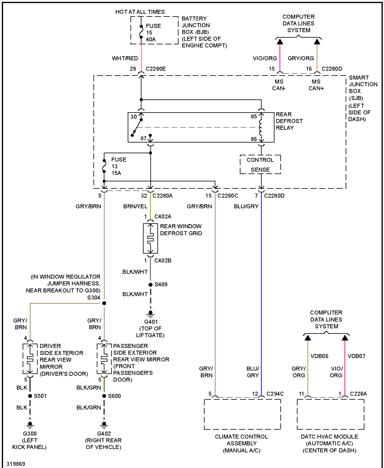
Fig. 12: Defoggers Circuit
