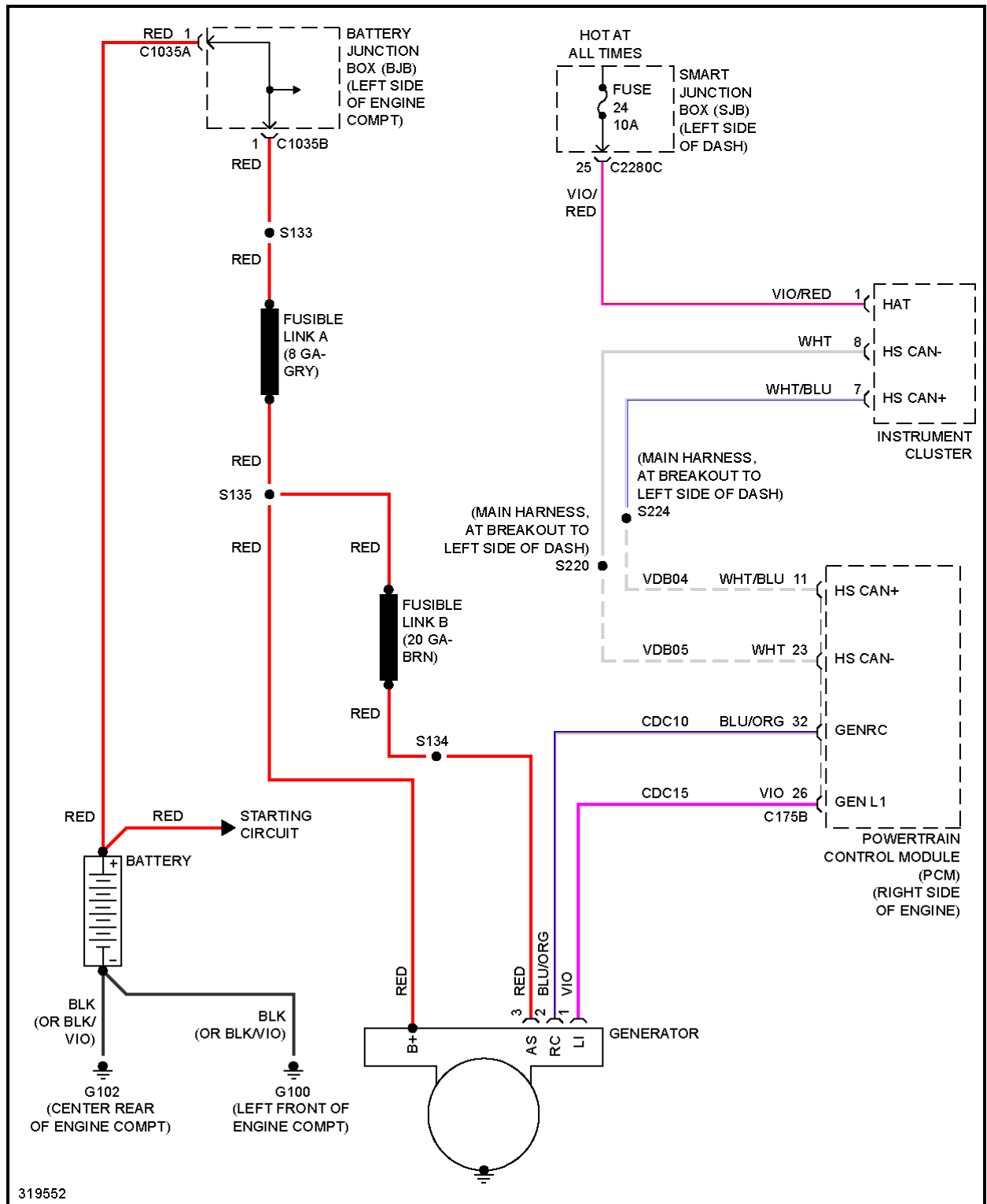
Fig. 72: Charging Circuit
