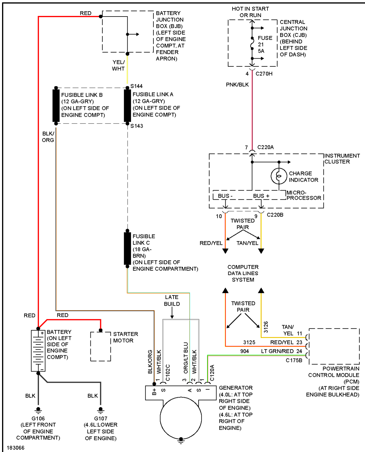
Fig. 60: Charging Circuit
