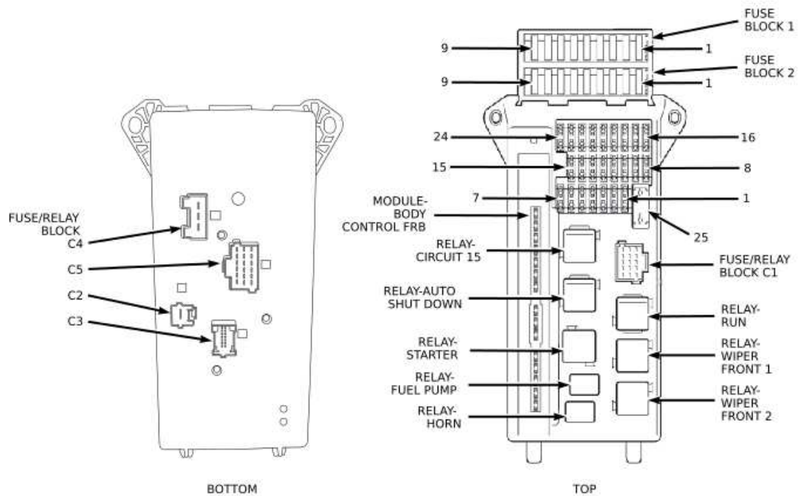
Fig. 14 FUSE/RELAY BLOCK
