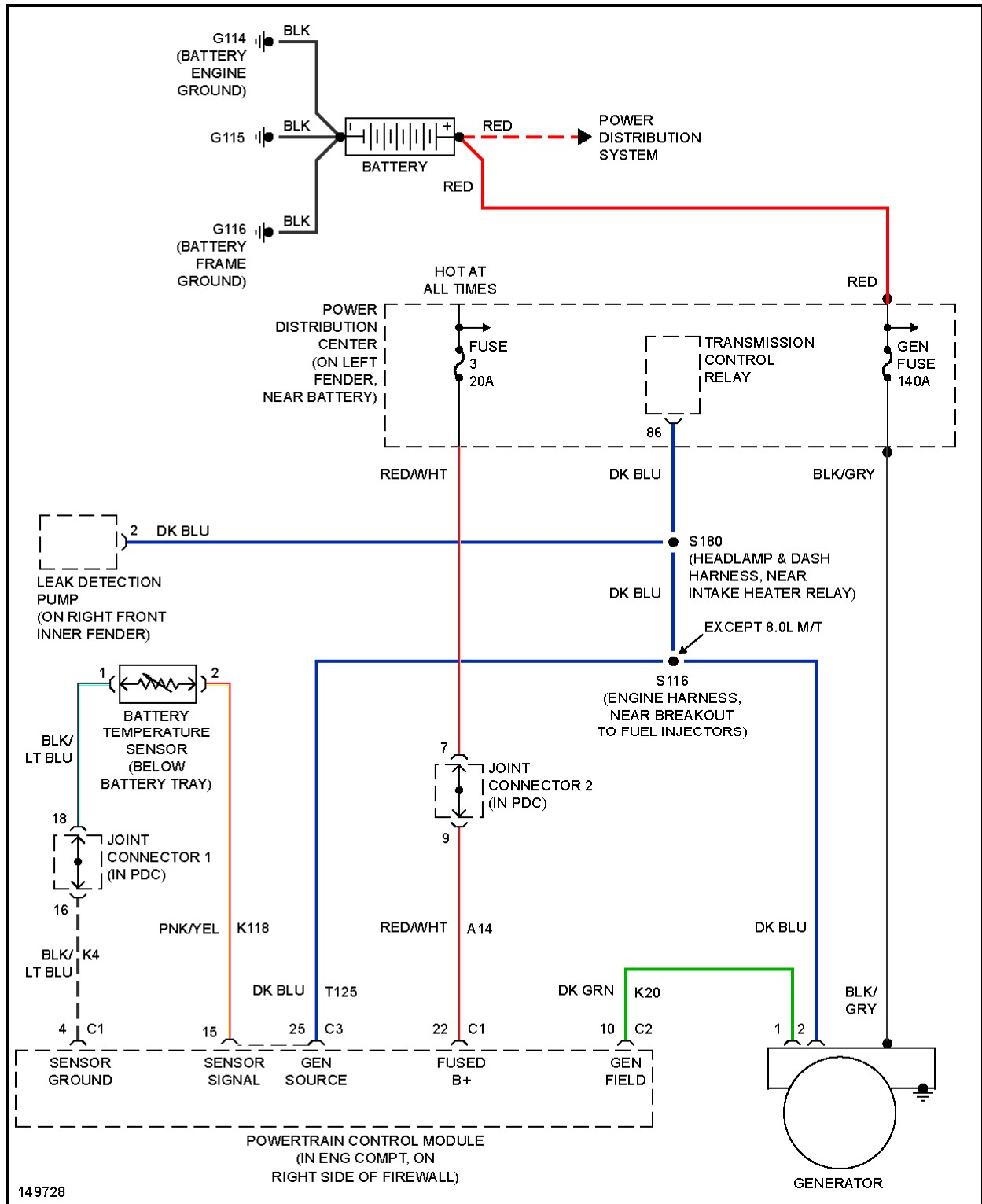
Fig. 60: 8.0L, Charging Circuit
