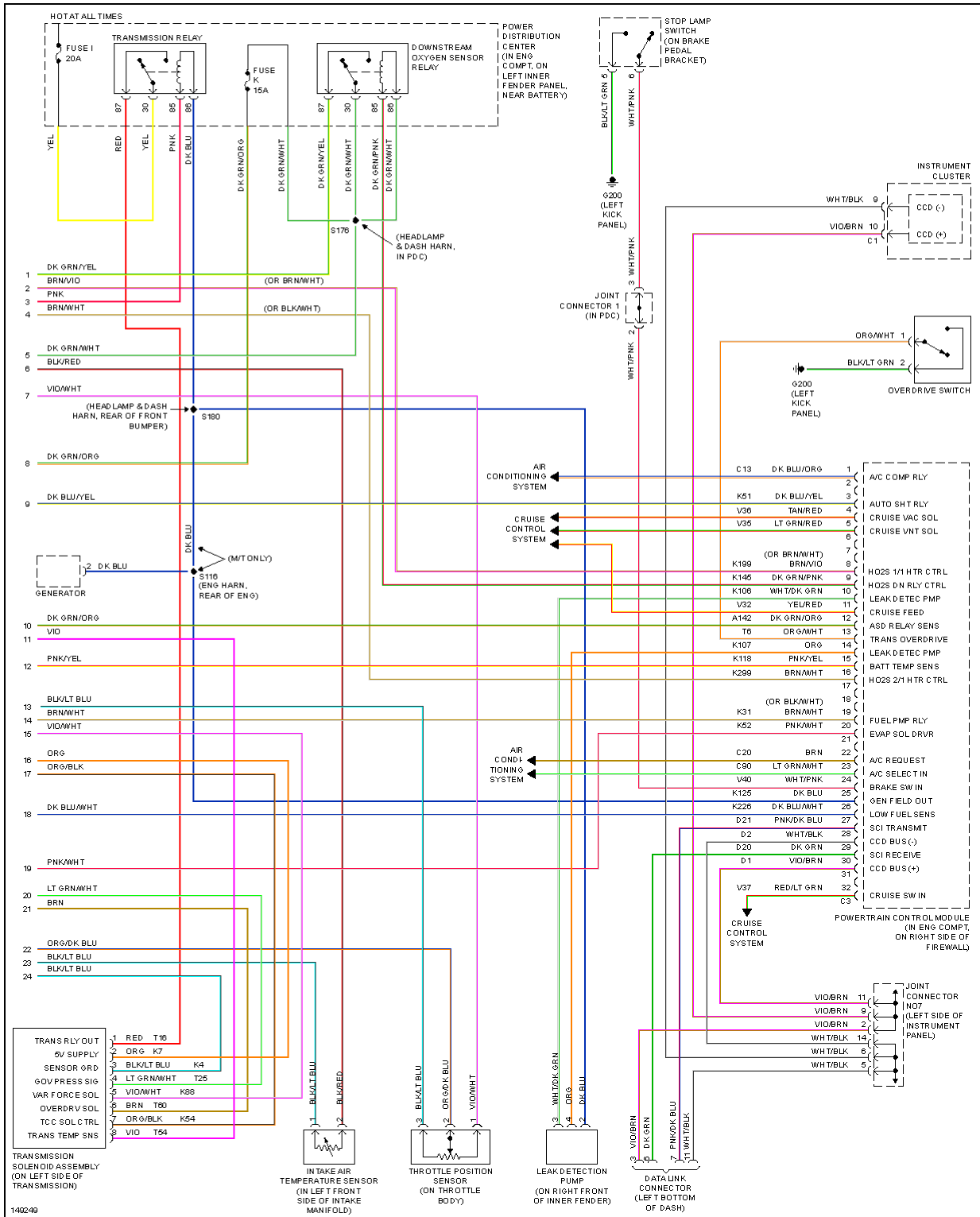
Fig. 26: 8.0L, Engine Performance Circuits (3 of 3)
