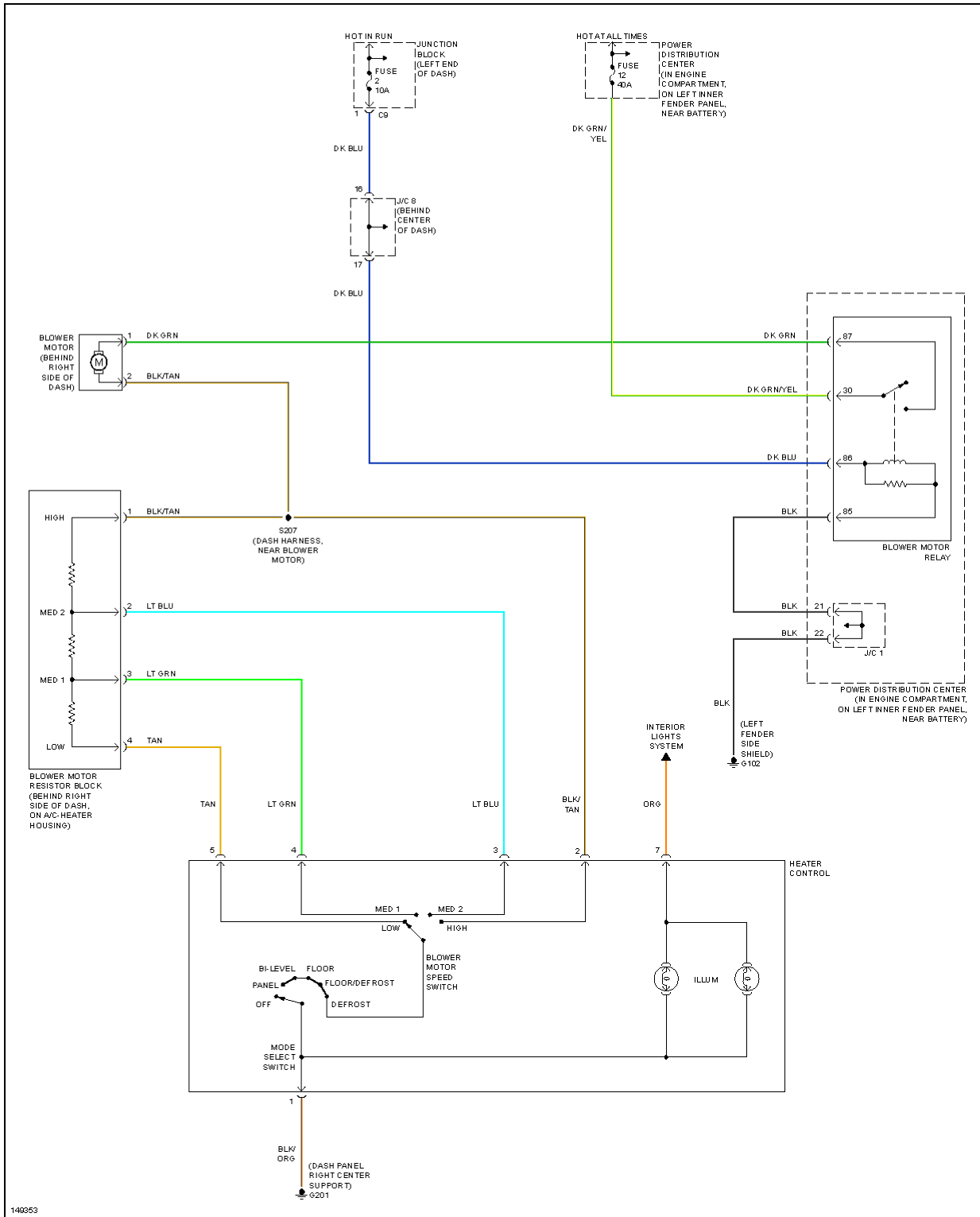
Fig. 1: Heater Circuit
