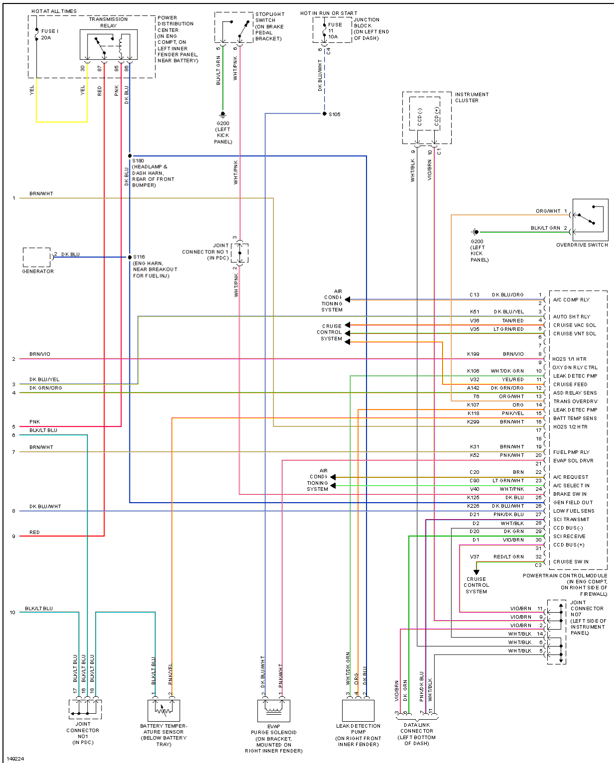
Fig. 19: 5.9L, Engine Performance Circuits, Federal (4 of 4)
