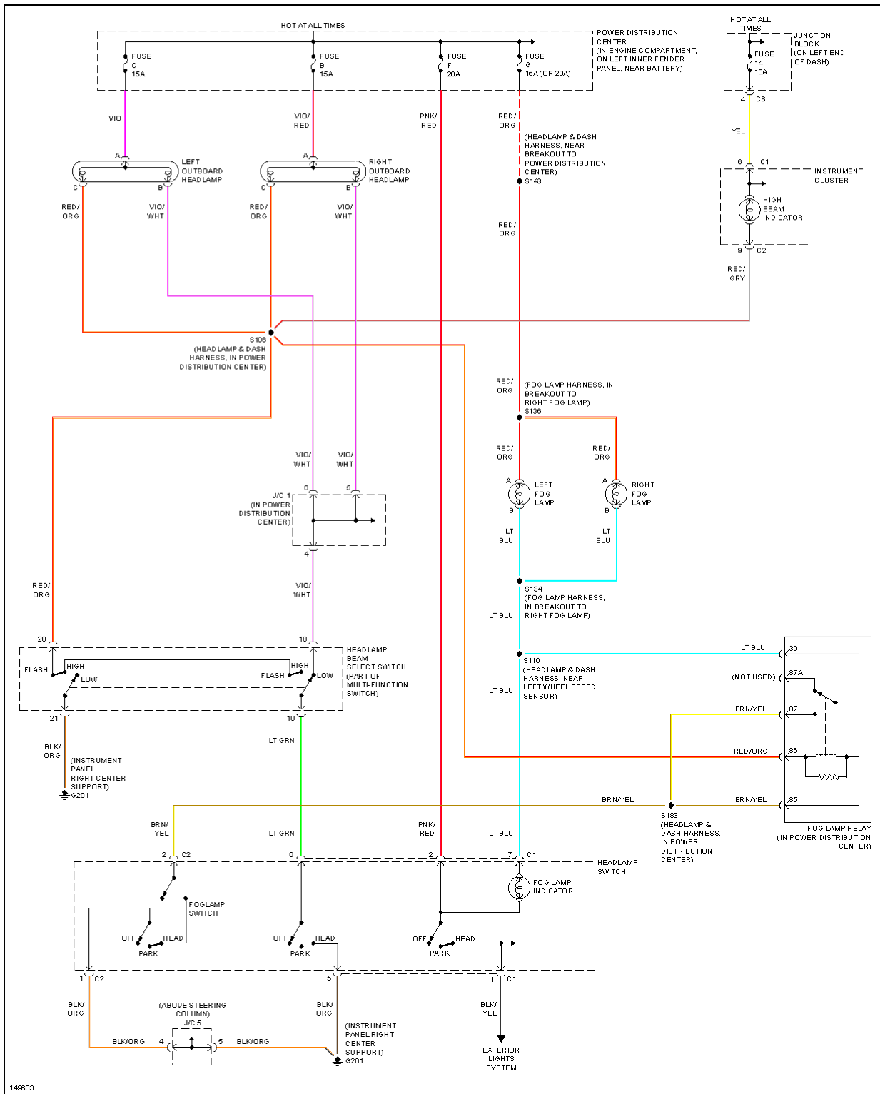
Fig. 37: Headlight Circuit, W/O DRL & W/O Quad Headlights
