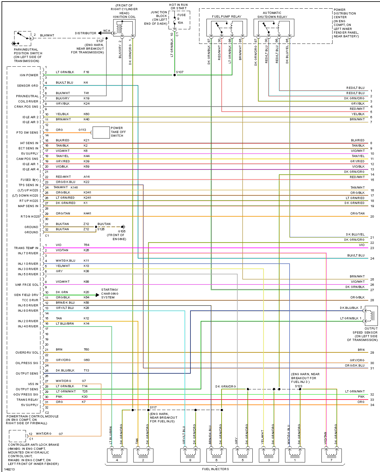
Fig. 12: 5.9L, Engine Performance Circuits, California (1 of 4)
