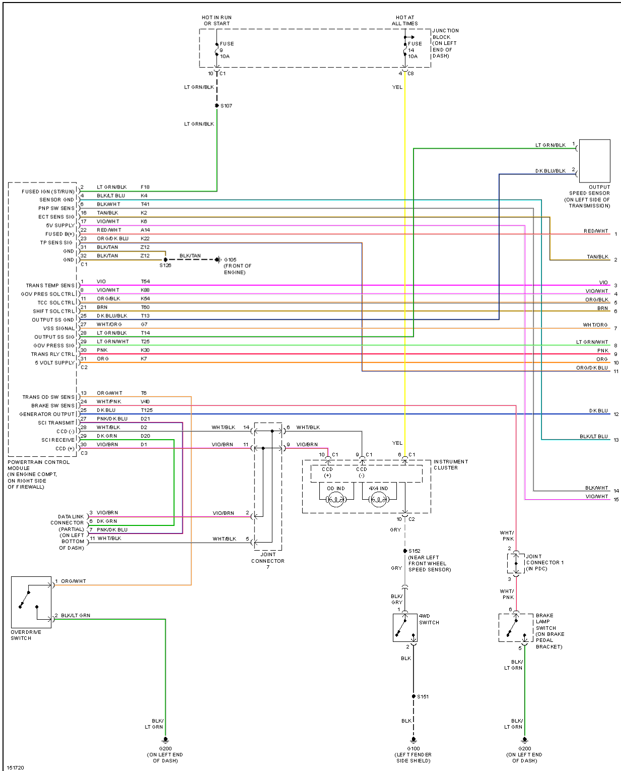
Fig. 65: 5.9L, A/T Circuit (1 of 2)
