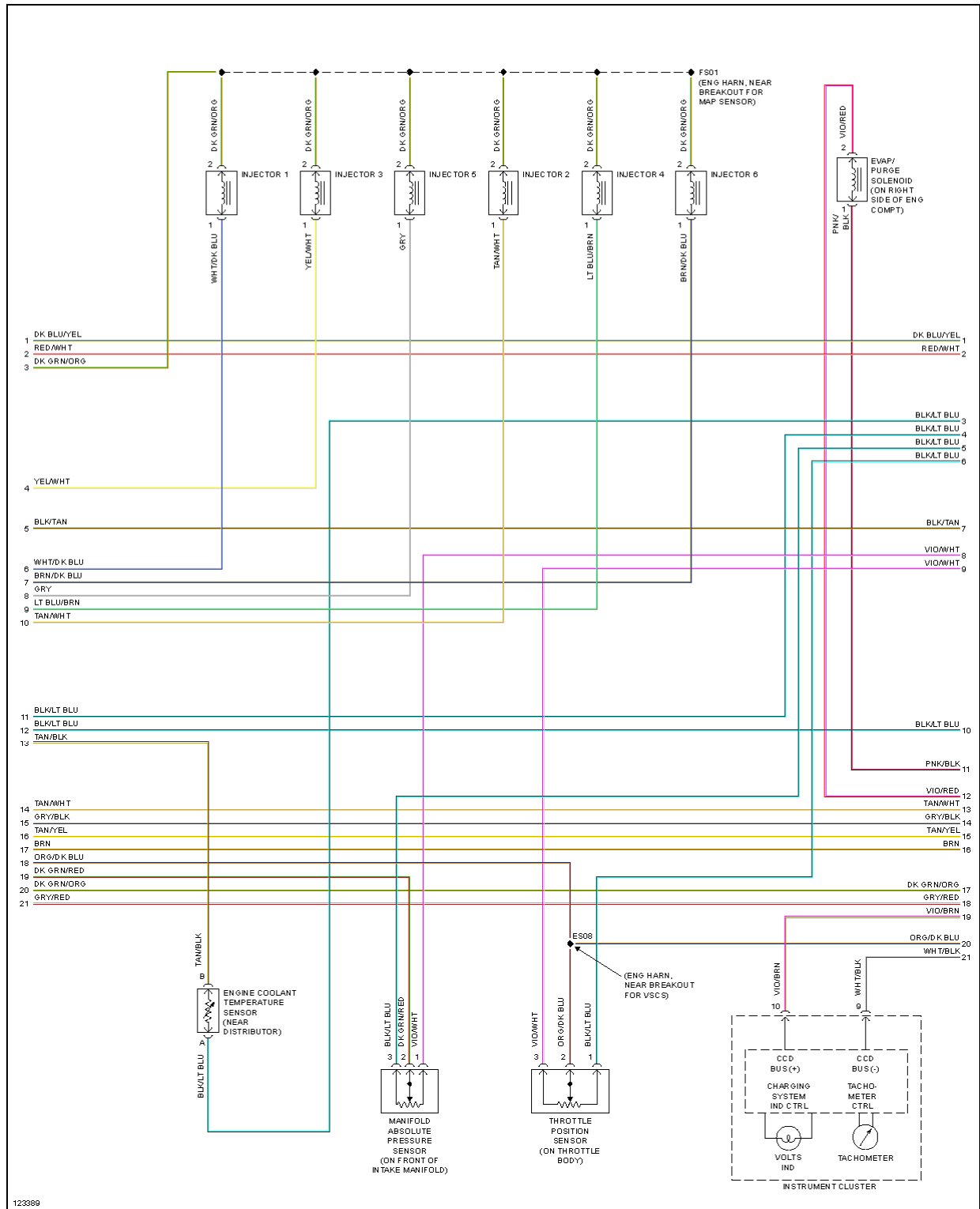
Fig. 17: 3.0L, Engine Performance Circuits (2 of 3)
