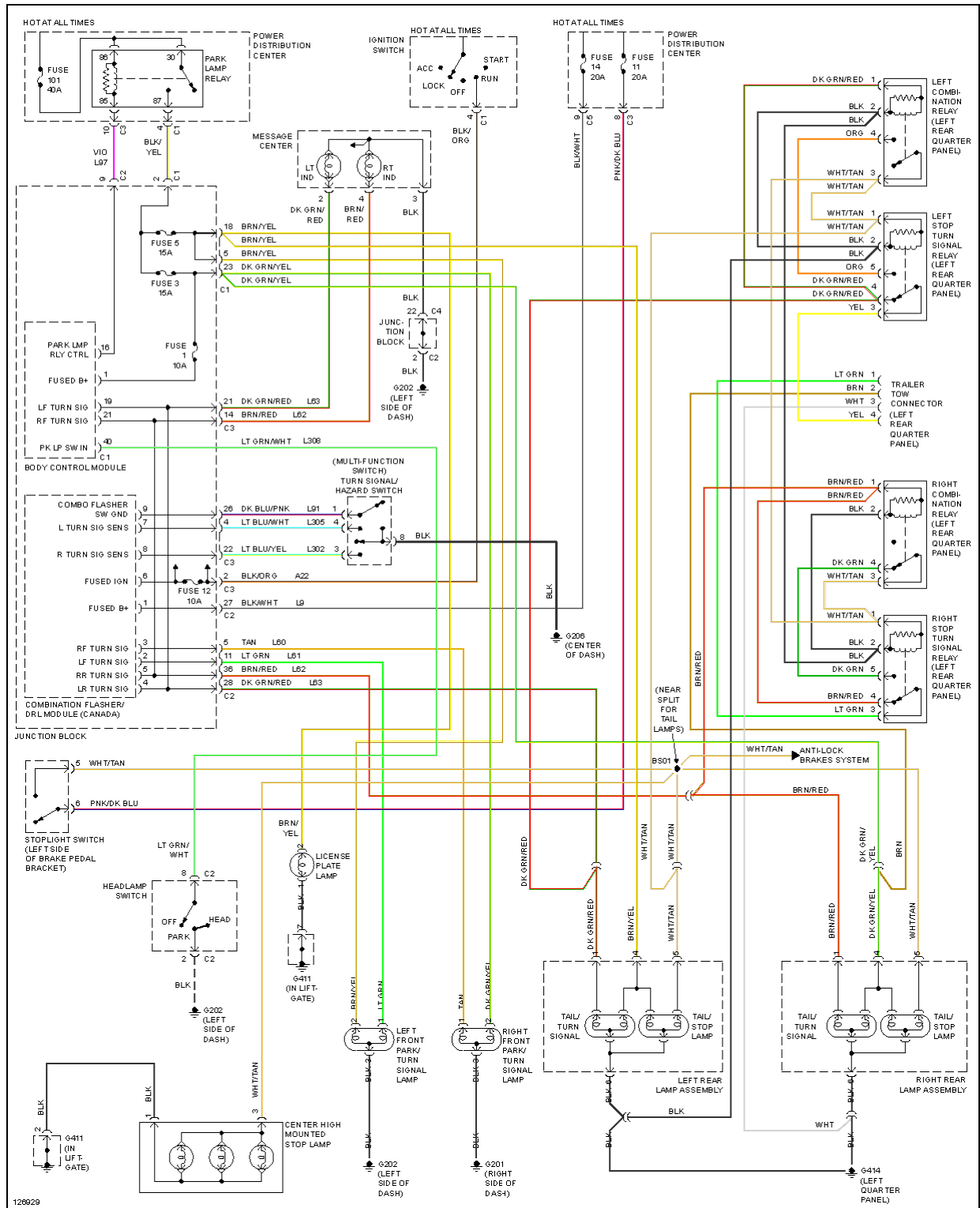
Fig. 29: Exterior Lamps Circuit, W/ Trailer Tow
