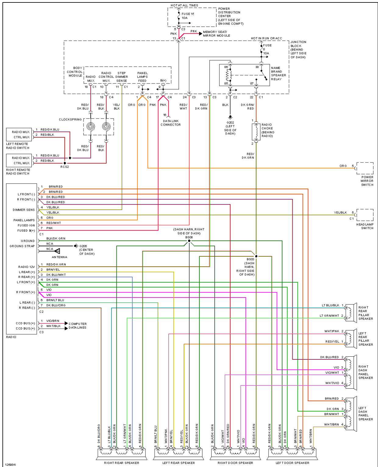
Fig. 50: Premium Sound Radio Circuit
