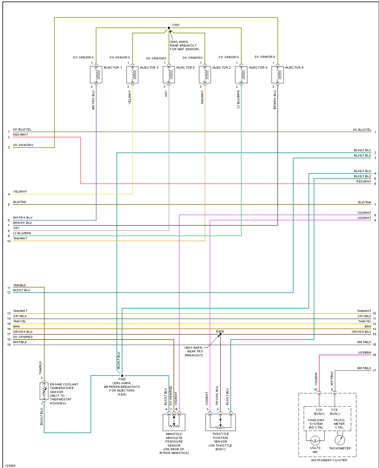
Fig. 23: 3.3L, Engine Performance Circuits (2 of 3)
