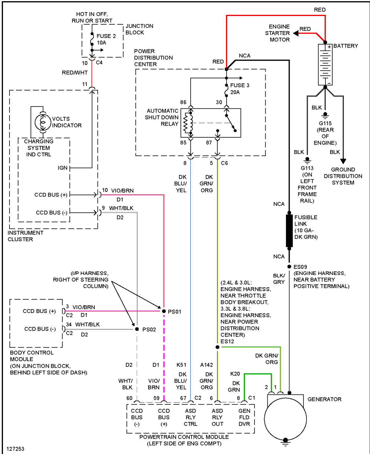
Fig. 53: Charging Circuit
