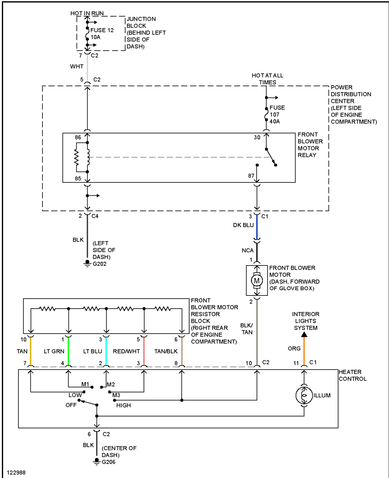
Fig. 1: Heater Circuit
