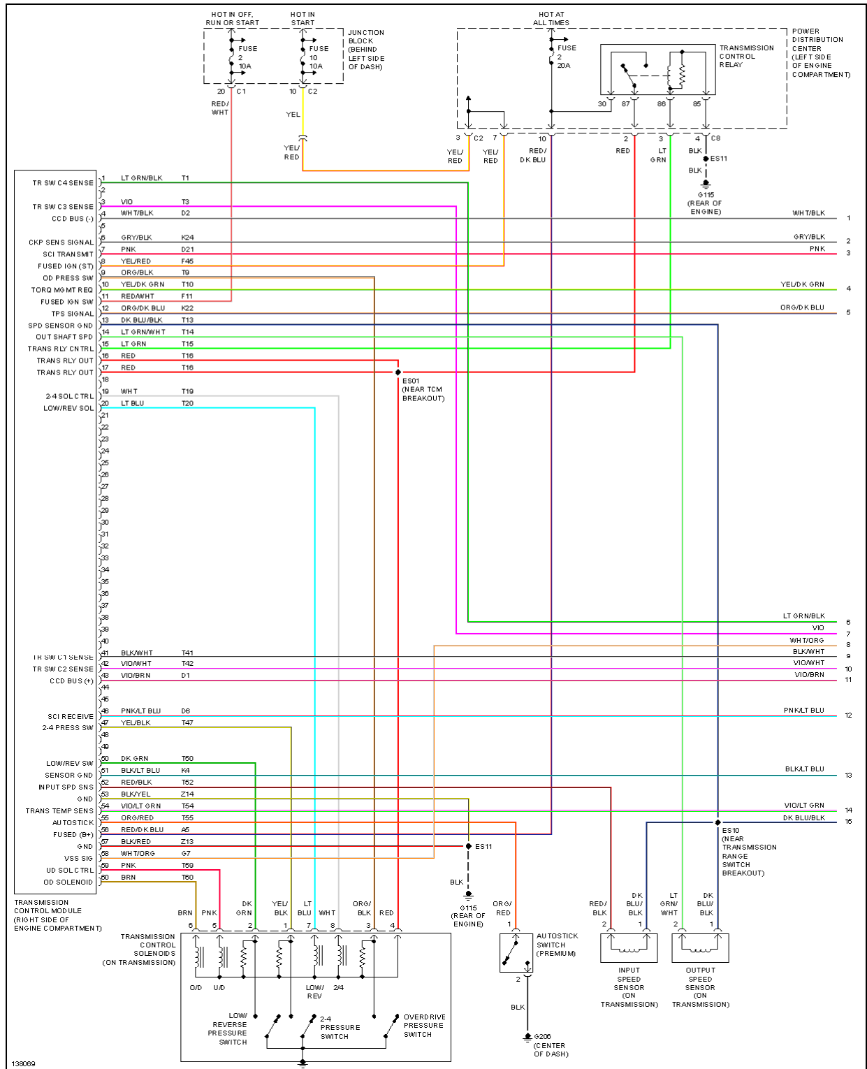
Fig. 59: 3.3L Flex Fuel, A/T Circuit (1 of 2)
