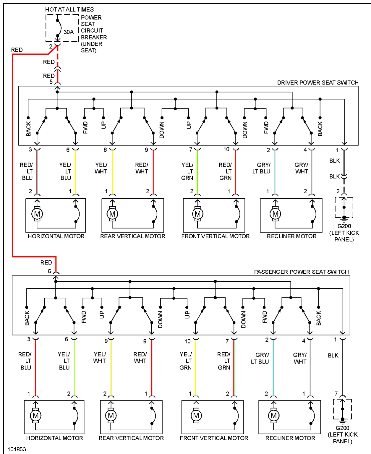
Fig. 47: 6-Way Power Seat Circuit
