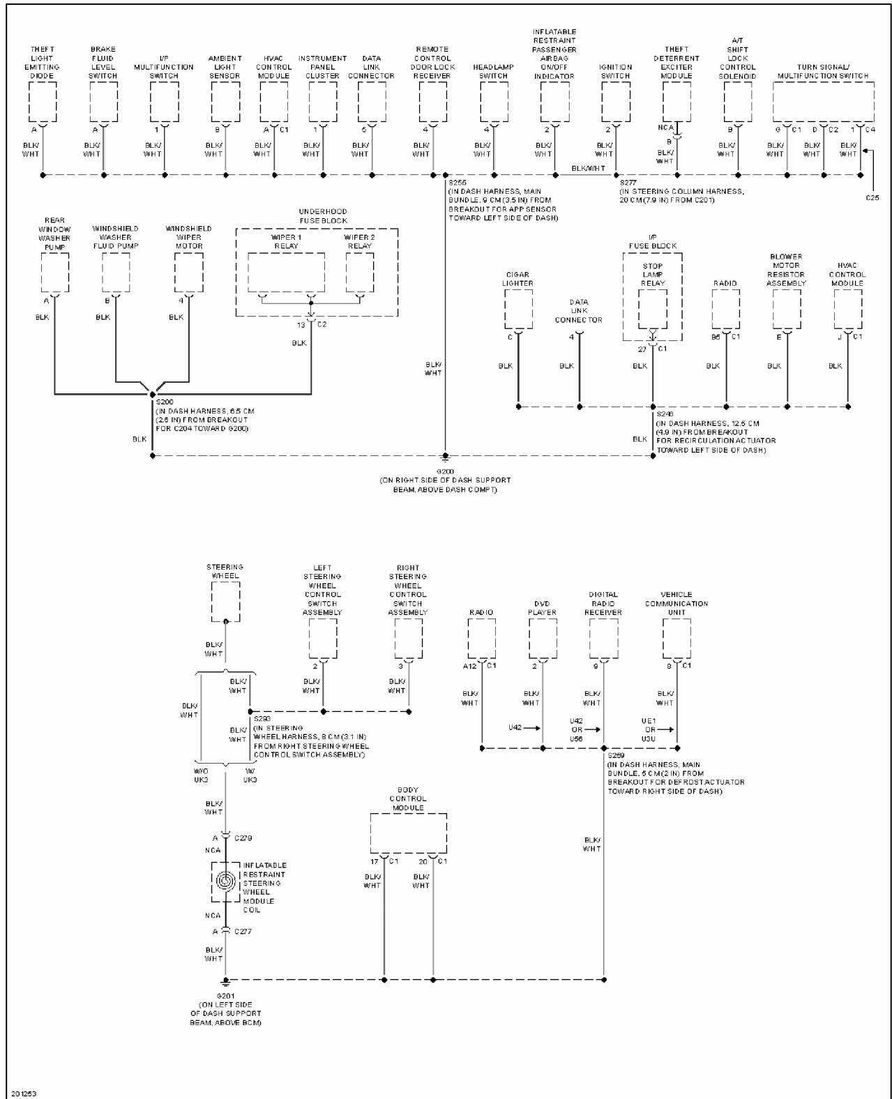
Fig. 23: Ground Distribution Circuit (2 of 5)
