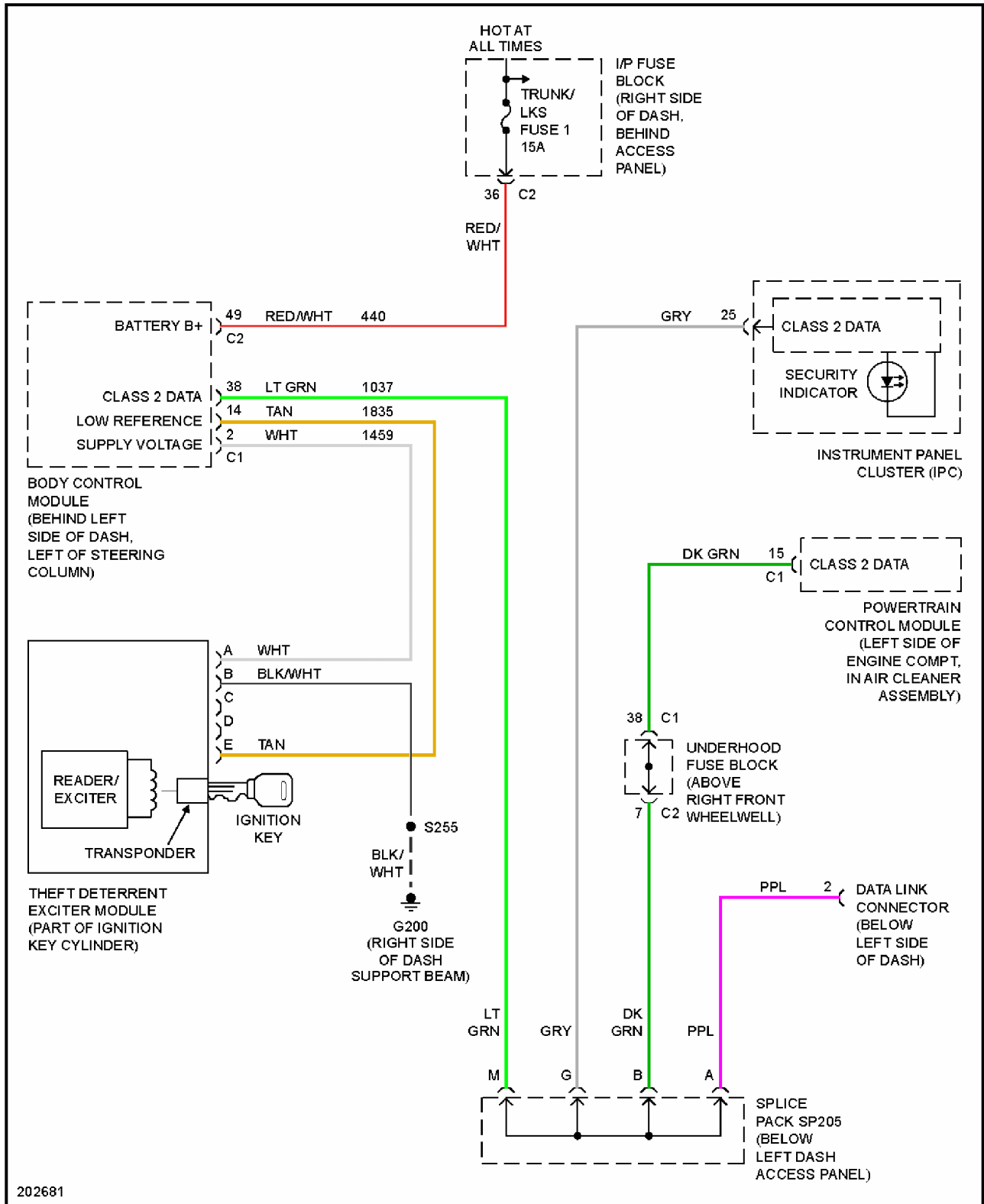
Fig. 8: Pass-Key Circuit
