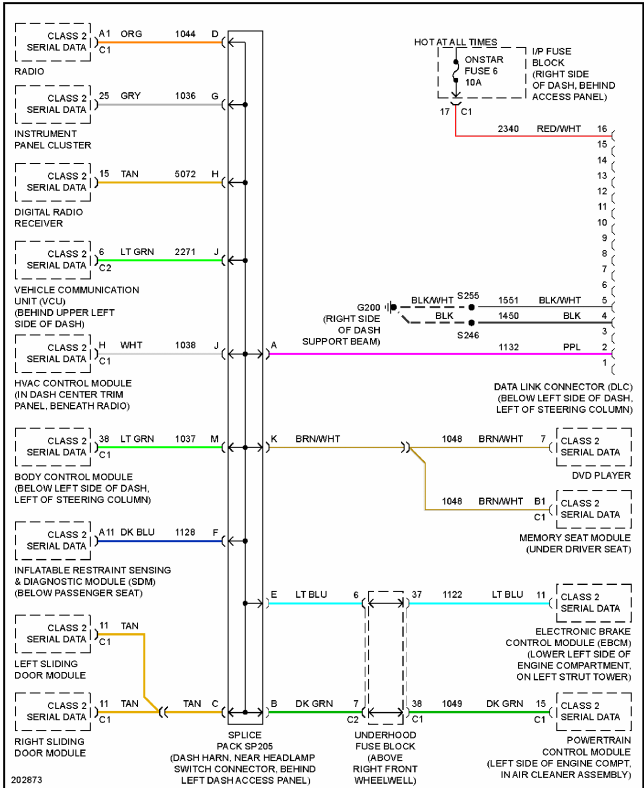
Fig. 10: Computer Data Lines Circuit
