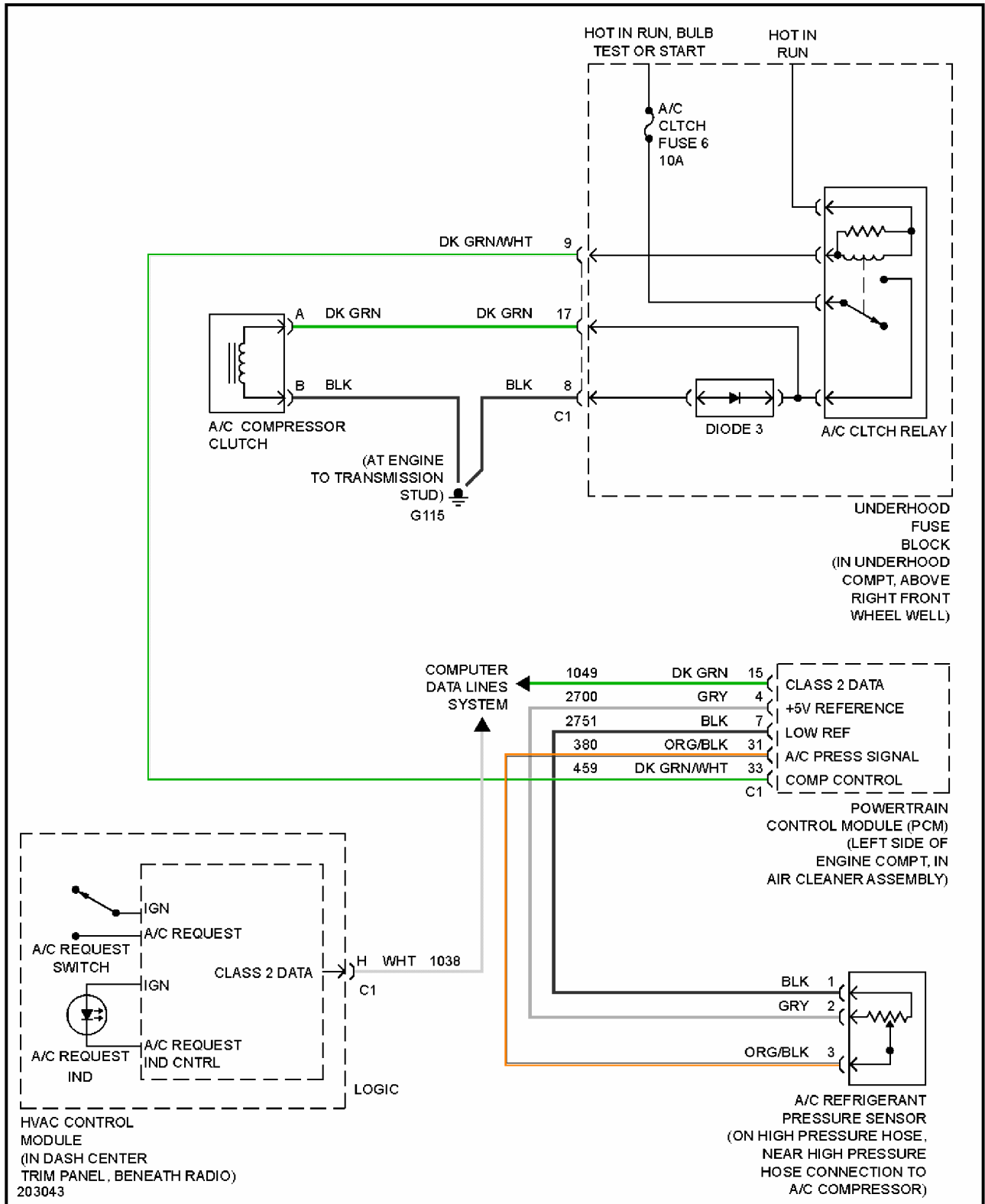
Fig. 1: Compressor Circuit
