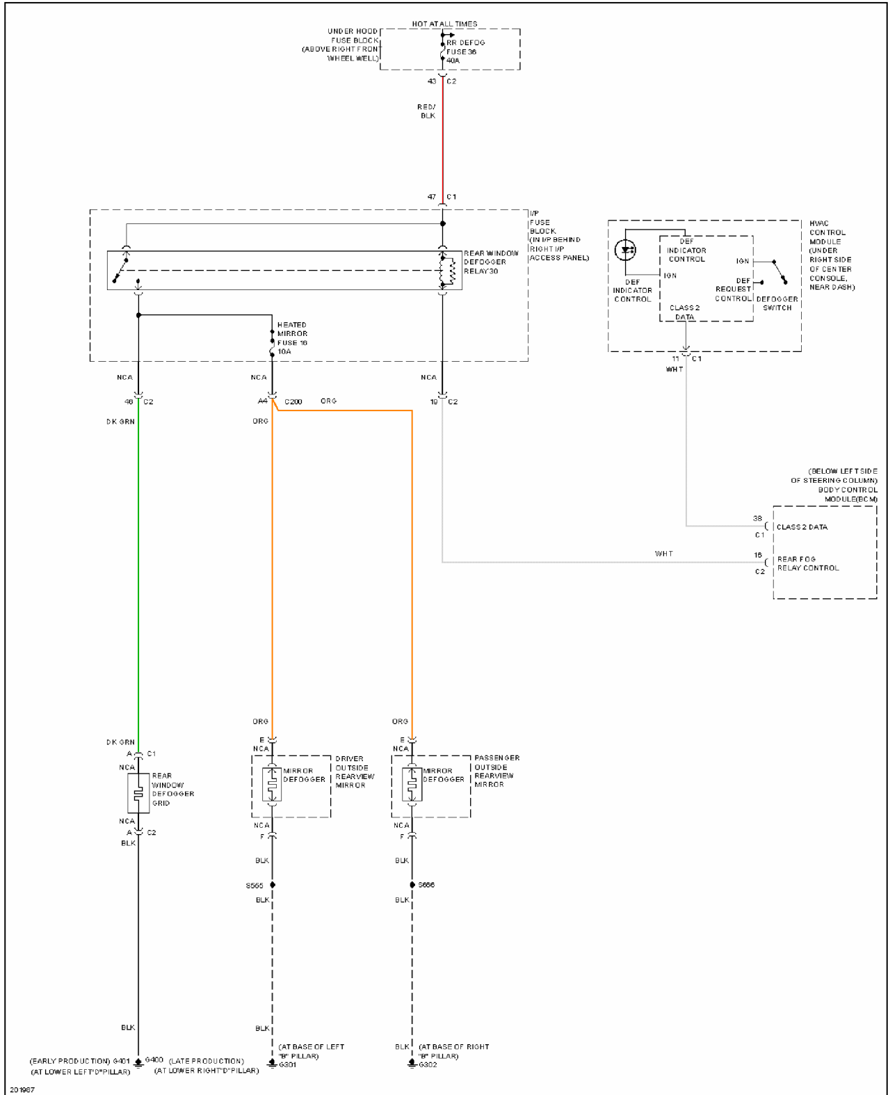
Fig. 13: Defoggers Circuit
