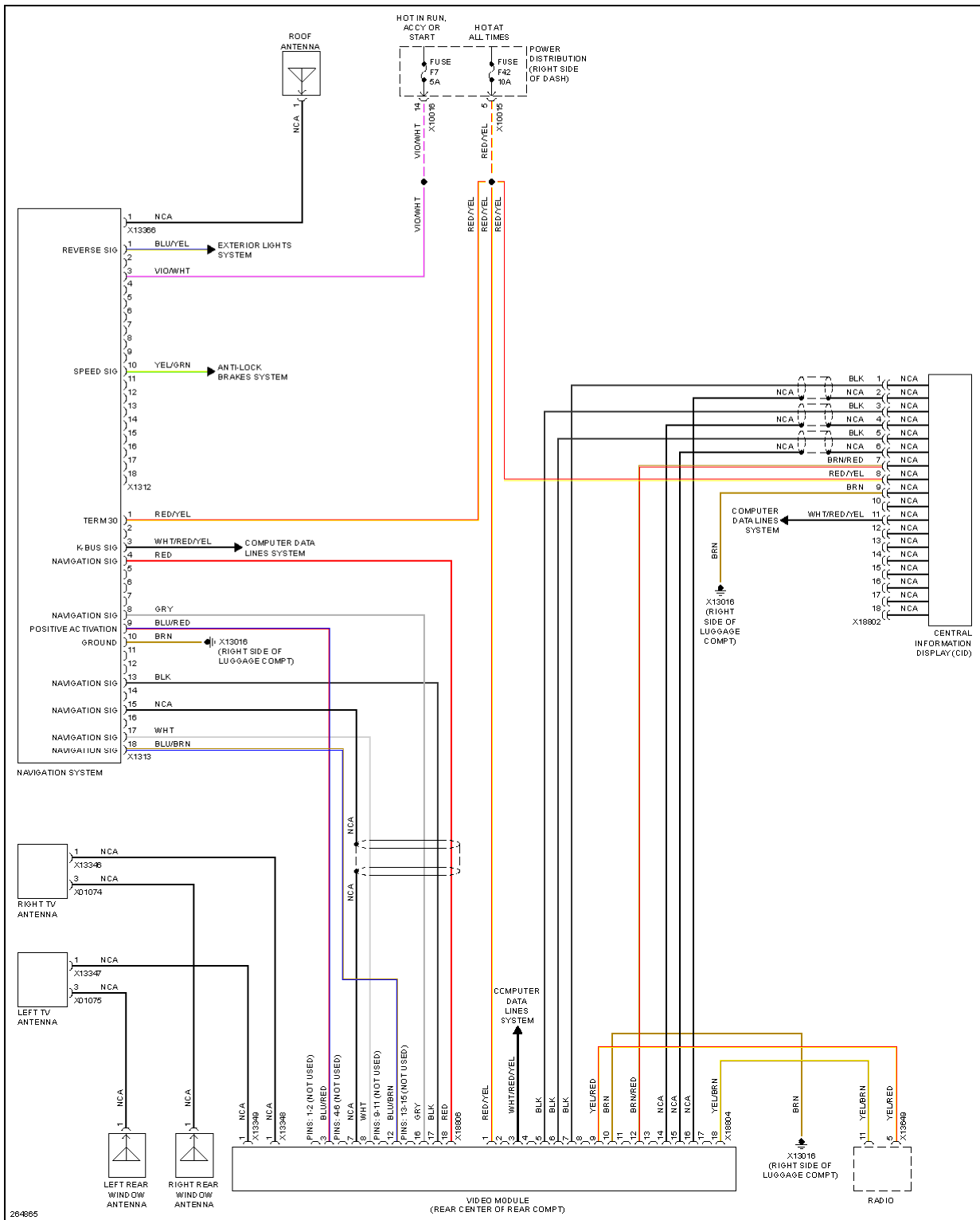
Fig. 36: Navigation Circuit, W/ Video Module
